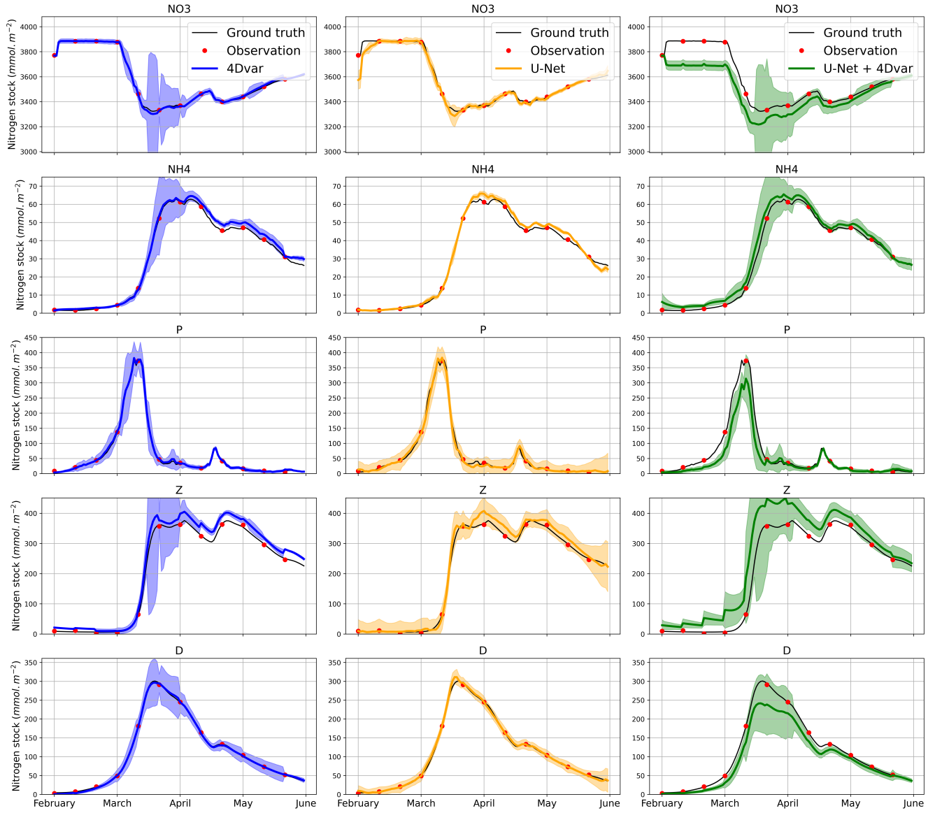
Figure C2. Plot of the reconstructed stocks associated to the five BGC states: NO_3 , NH_4 , P , Z and D ; for one sample using a 4Dvar-based scheme (blue), a UNet-based scheme (orange) and a hybrid 4Dvar+UNet base method (green), w.r.t. a scenario of case 1 forcing uncertainty, states observed with a 10-day time sampling and a CTD+Rosette-like sampling strategy. The bold line refers to the mean stock among the 10-members ensemble and the uncertainty, i.e., the mean value \pm 2\sigma with \sigma the standard deviation of the ensemble, is associated colourized shape. The ground truth is represented by the black curve.
