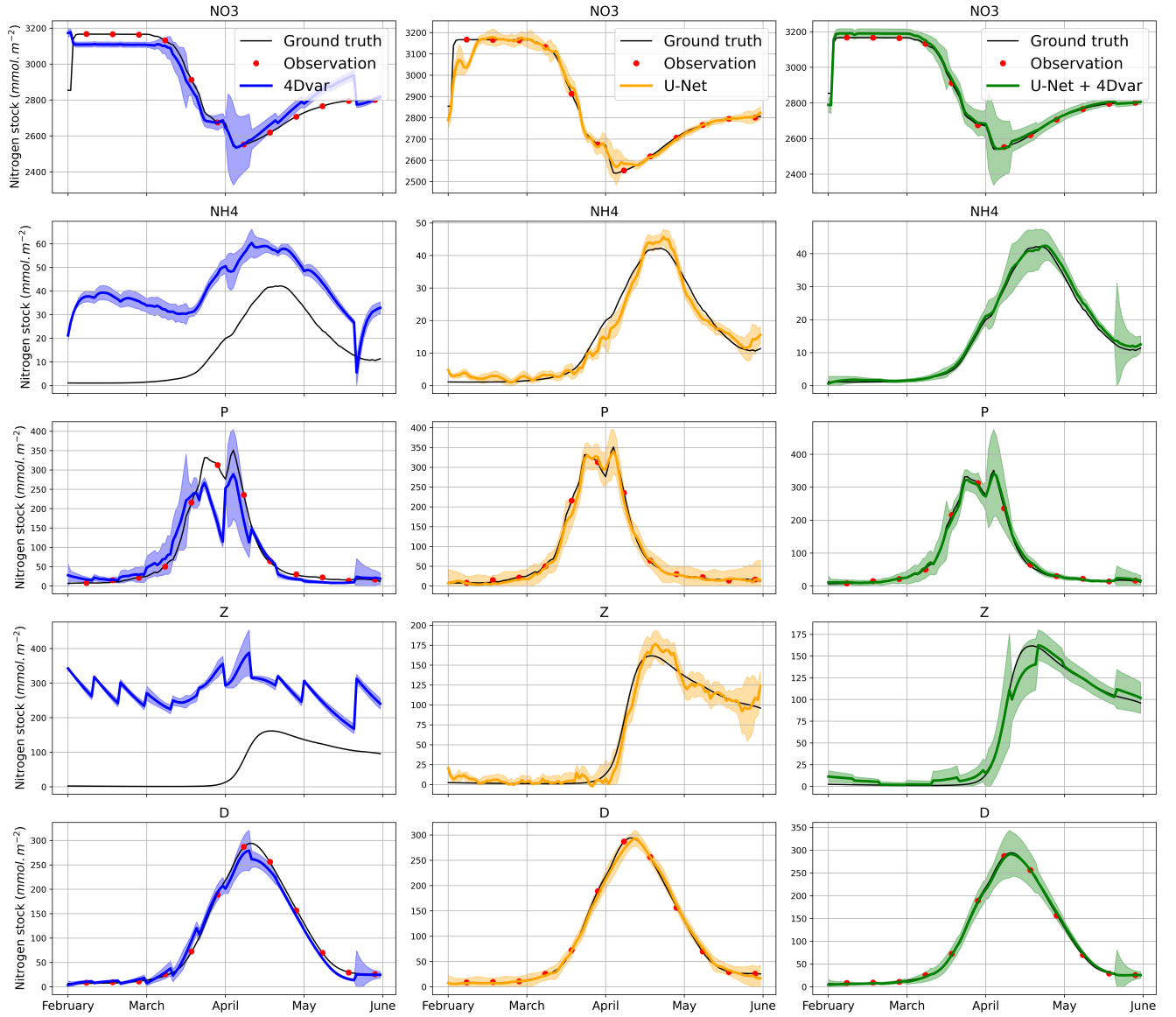
Figure F1. Reconstructed stocks associated with the five BGC states: NO_3 , NH_4 , P , Z and D ; for one ensemble using a DA-based scheme (blue), a UNet-based scheme (orange) and a hybrid 4DVar+UNet base scheme (green), w.r.t. a scenario of case 1 forcing uncertainty, states observed with a 10-day time sampling and a CTD-only sampling strategy. The bold line indicates the mean stock among the 10-member ensemble, with the uncertainty, i.e., the mean value \pm 2\sigma with \sigma being the standard deviation of the ensemble. The aforementioned confidence interval is associated with the coloured shape. The ground truth is represented by the black curve. The observed states are denoted by red dots.
