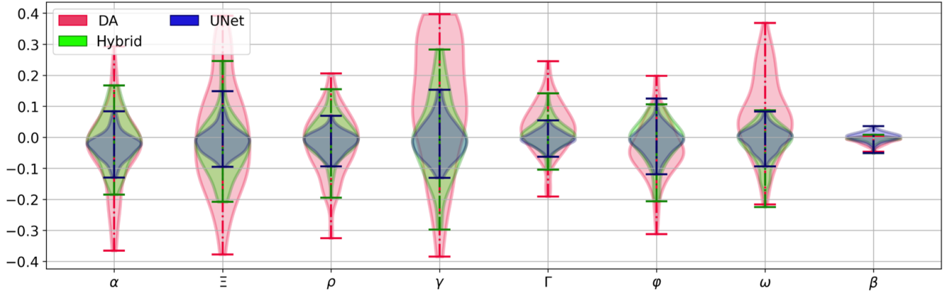
Figure E1. Evaluation metrics of the calibration of the BGC model. We assess a 4Dvar scheme (red distribution), a learning-based scheme (blue distribution) and a hybrid scheme (green distribution). We consider the normalized parameter estimate error as detailed in Section 3.5.
