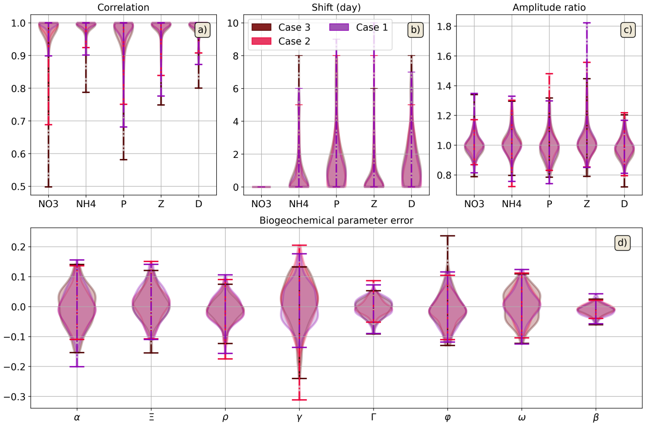
Figure 7. Evaluation metrics of the learning-based calibration of the BGC model with respect to forcings' uncertainties. We consider the same metrics as in Fig. 6 with the same evaluation dataset of 100 1D BGC simulations. We compare the distribution of the metrics for three scenarii with increasing forcings' uncertainty levels: namely, case-1 (purple distribution), case-2 (red distribution) and case-3 (brown distribution) as described in Section 2.3. These experiments rely in the baseline observation configuration with a CTD+Rosette strategy and a 10-day time sampling (see Section 2.4).
