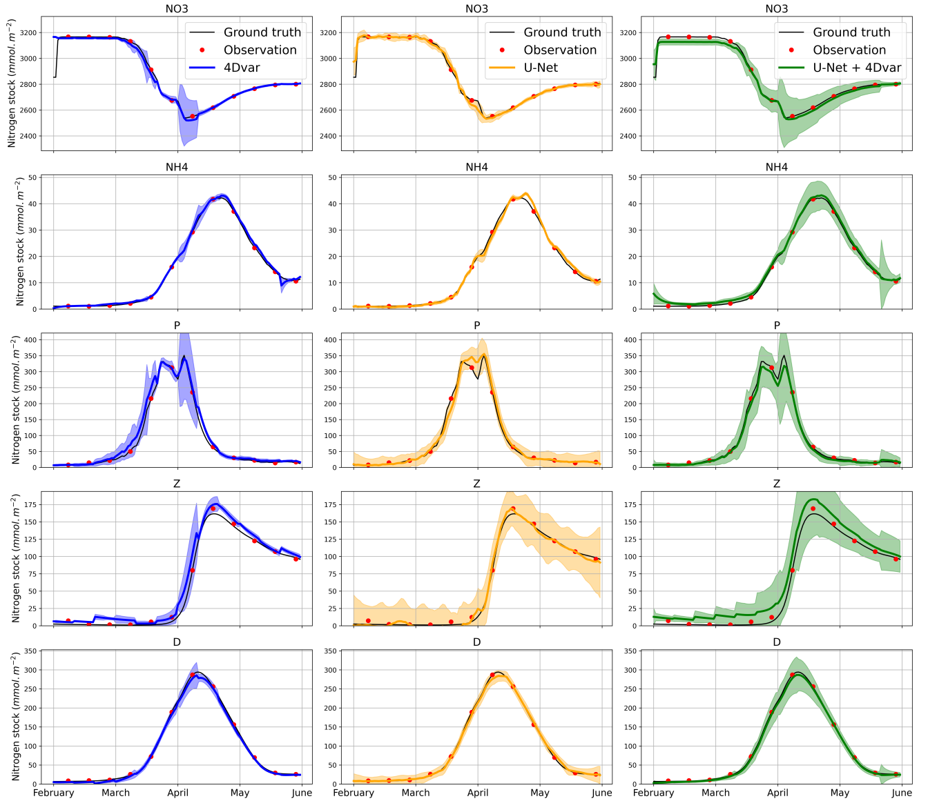
Figure 11. Reconstructed stocks associated with the five BGC states: NO_3 , NH_4 , P , Z and D ; for one sample ensemble (blue), a UNet-based scheme (orange) and a hybrid UNet+4DVar base scheme (green), w.r.t. a scenario of case 1 forcing uncertainty, states observed with a 10-day time sampling and a CTD+Rosette-like sampling strategy. The bold line indicates the mean stock among the 10-member ensemble, with the uncertainty, i.e., the mean value \pm 2\sigma with \sigma being the standard deviation of the ensemble 10 members. The aforementioned confidence interval is associated with the colourized shape. The ground truth is represented by the black curve. The observed states are denoted by red dots.
