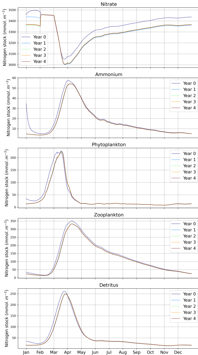
Figure G1. Simulated nitrogen stocks , averaged over one hundred samples across five consecutive years. The stocks are shown for nitrate, ammonium, phytoplankton, zooplankton, and detritus (from top to bottom). The one hundred samples constitute the test dataset and differ in their sets of BGC parameters and physical forcing.
