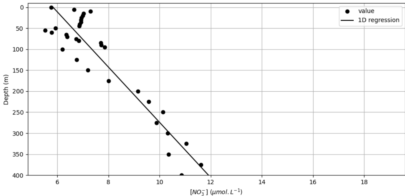
Figure B1. Nitrate vertical profile at the Porcupine Abyssal Plain (PAP) station. Monthly reanalysed nitrate data from Reagan et al. (2024) are shown for December, January, and February (dots), together with a first-order polynomial fit (line).
