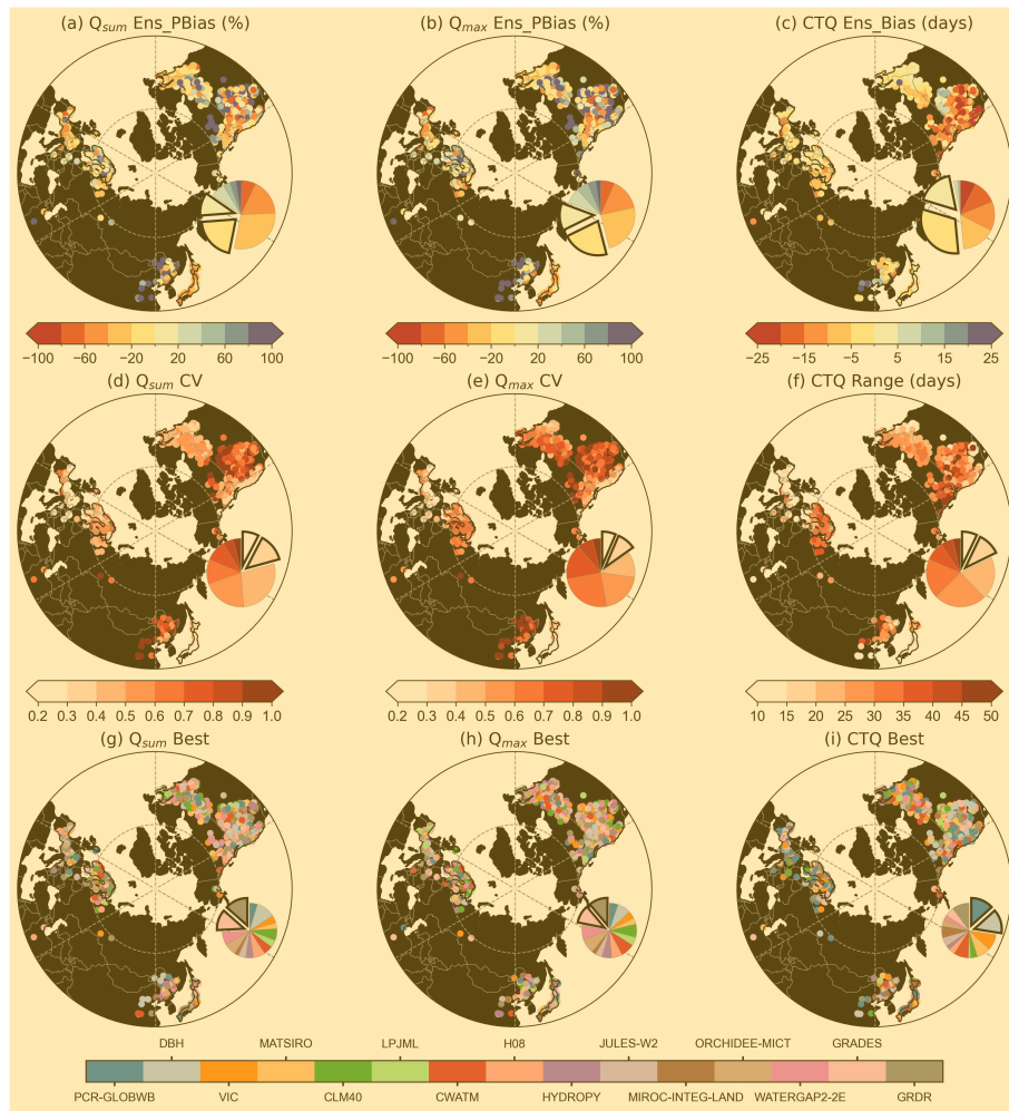
Figure 6. Bias, variability, and the best model for simulated SMR characteristics across different basins. (a–c) show the percent bias of Q_{\text{sum}} (%), percent bias of Q_{\text{max}} (%), and bias of CTQ (days), respectively, in the simulated SMR. (d–f) show inter-model variability represented by the coefficient of variation (CV) for Q_{\text{sum}} and Q_{\text{max}} , and inter-model range of CTQ (days). (g–i) show the model with the smallest bias in each basin for Q_{\text{sum}} , Q_{\text{max}} , and CTQ, respectively. The pie charts provide a summary of these patterns, with bold black outlines highlighting the proportion within \pm 20\% bias in (a–c), the two lowest variability levels in (d–f), and the top two models with the highest proportions in (g–i).
