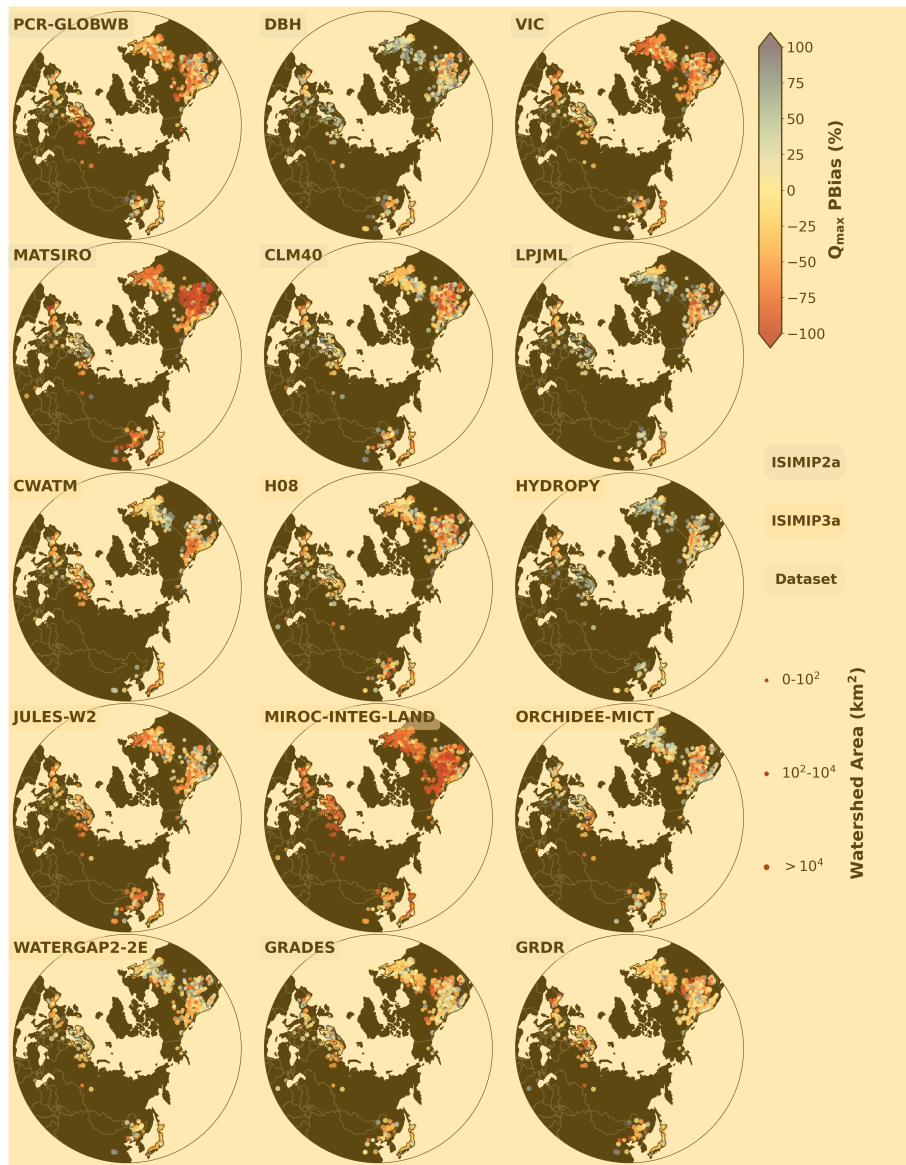
Figure A6. The percentage bias of peak flow ( Q_{\max} ) during the snowmelt period (unit: %). Colors indicate the degree of bias compared to observations: red represents underestimation, blue indicates overestimation, and yellow signifies well-matched total runoff. The point size is adjusted based on station density for better visualization and does not have physical significance. Colored boxes around model/dataset names denote three categories of analysis data.
