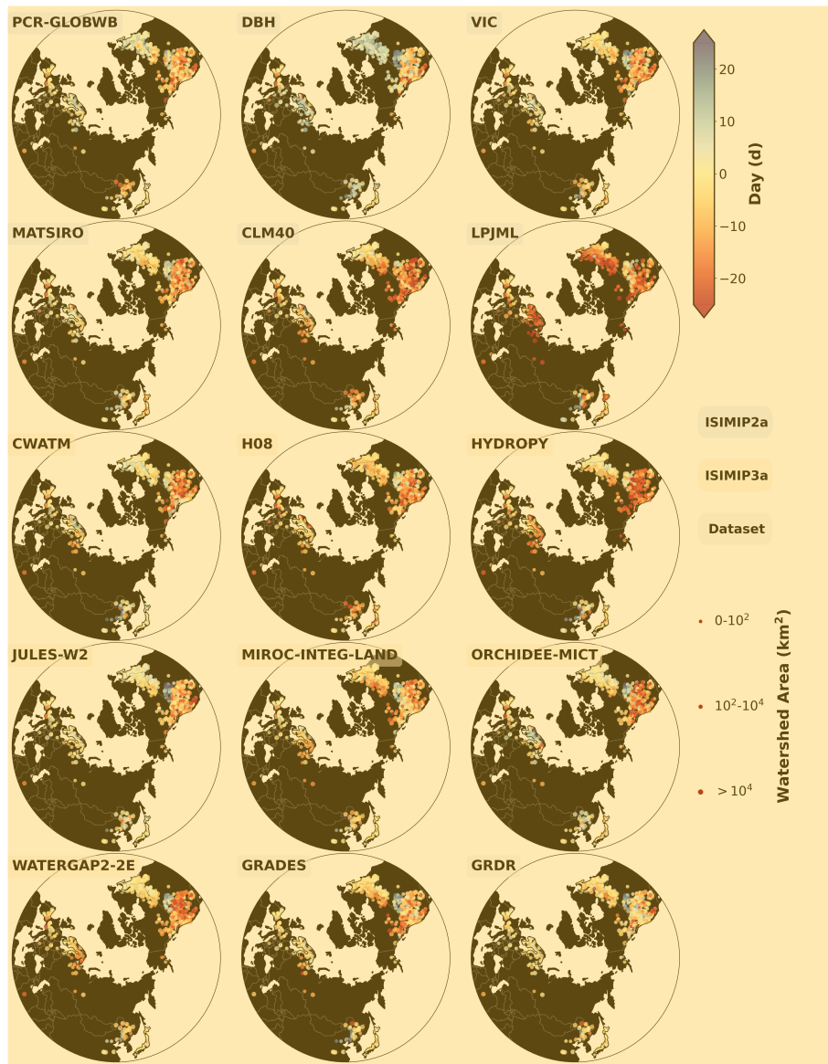
Figure A7. The bias in snowmelt timing, represented by the centroid time of runoff (CTQ) during the snowmelt period (unit: day) Colors indicate the extent of bias compared to observations: red represents earlier snowmelt, blue indicates later snowmelt, and yellow signifies well-matched snowmelt timing. The point size is adjusted based on station density for better visualization and does not have physical significance. Colored boxes around model/dataset names denote three categories of analysis data.
