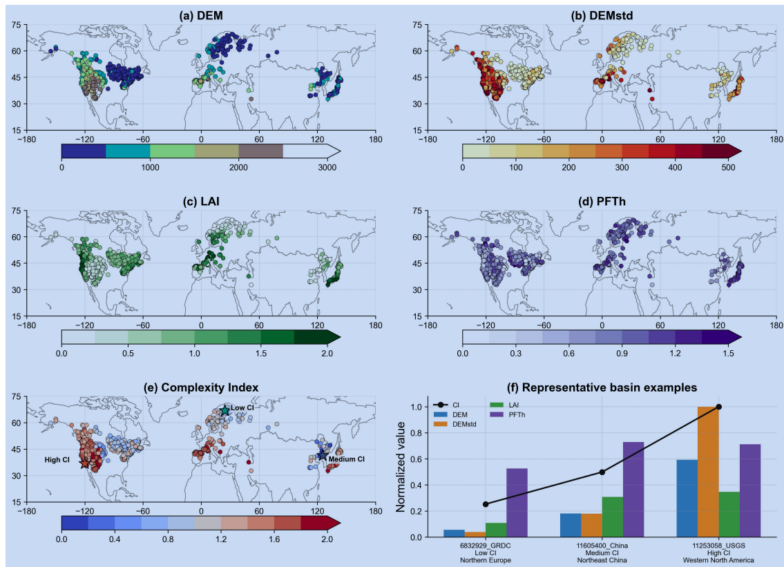
Figure 3. Spatial distribution of basin complexity components and representative examples of the integrated Complexity Index. Panels show (a) DEM, (b) DEMstd, (c) LAI, (d) PFTh, and (e) the integrated Complexity Index (CI) across the study basins. The three starred basins in panel (e) are representative examples of Low CI, Medium CI, and High CI conditions. Panel (f) compares the normalized values of DEM, DEMstd, LAI, PFTh, and CI for these three representative basins.
