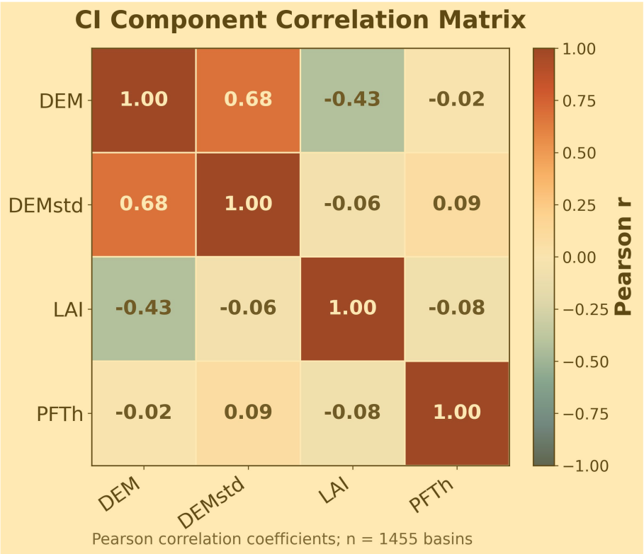
Figure A1 Pearson correlation matrix among the four components used to construct the basin complexity index. The value of each grid represents the Pearson correlation coefficients among teh DEM, DEMstd, LAI, and PFTh.
