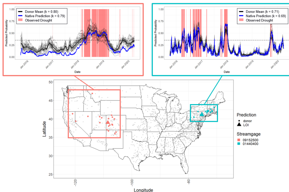
Figure 8. Two example prediction locations in the Southwest United States (U.S. Geological Survey [USGS] streamgage 09152500) and Northeast (USGS streamgage 01440400). The map displays the prediction locations as triangles, and the 19 selected donor gages for predicting at that location as circles of the same color. Time series of predicted streamflow drought probability for the model test period 2015-2020 are displayed for their corresponding prediction locations, with periods of observed streamflow drought displayed in red, the donors in black (mean donor prediction is bold), and the at-site model predictions in blue. A dashed line at 0.35 indicates the threshold for predicted streamflow drought status, where predictions above the line indicate streamflow drought and below indicate non-drought.
