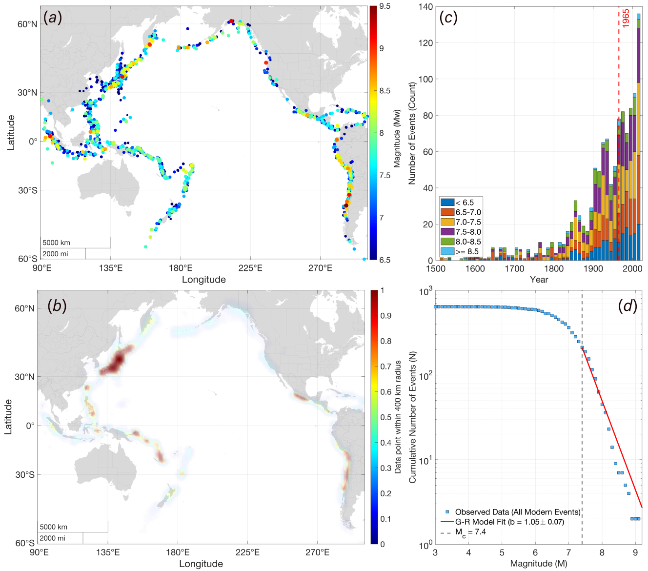
Figure 1. (a) Historical tsunamigenic earthquakes based on ~1600 events from ~500 BCE to 2025. The colormap indicates event magnitude (Mw); (b) Spatial density plot (heatmap) showing earthquake clustering, calculated with a 400 km radius of influence; (c) Histogram of historical events per decade since 1500, with bars color-coded by event magnitude. The vertical red line at 1965 marks the start of modern event records used in this study; (d) b-value estimate, showing the Gutenberg–Richter model fit (red line) to historical data since 1965 for events of magnitude \geq 7.4 . Basemap created with Natural Earth data.
