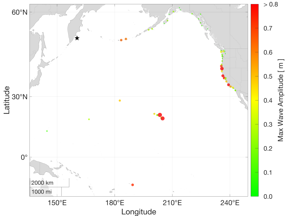
Figure 10. Maximum observed water levels at NOAA tide gauge stations along the coastline. Basemap created with Natural Earth data.
