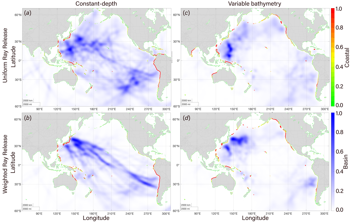
Figure 3. Basin-wide ray density and coastal tsunami exposure for 9,000 tsunami rays released along potential fault zones (shown in Figure 2). Panels (a,b) represent constant-depth cases, highlighting the effects of fault location and orientation, while panels (c,d) incorporate variable bathymetry to show the combined influence of seafloor geometry and fault configuration. The top row shows uniformly released rays, and the bottom row applies probabilistic weighting (using the annual rate parameter \lambda from Section 2) based on return period derived from the Gutenberg–Richter relation. The ocean-floor heatmap (white to blue) illustrates ray convergence and geometric focusing, and coastline colors (green–yellow–red) indicate relative coastal exposure using a normalized ray-count proxy (0–1), with redder areas denoting higher exposure. Basemap created with Natural Earth data.
