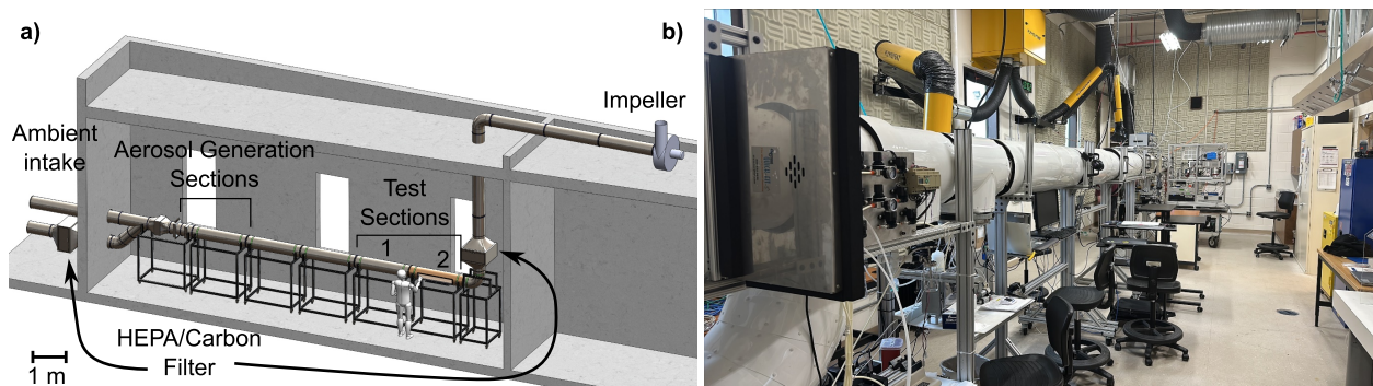
Figure 1. a) Diagram of the design of the AATF. b) Photo of the implementation. Manufactured by S3I, Inc. (S3I Engineering, n.d.).
