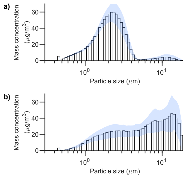
Figure 10. Comparison of size distribution (as reported by APS 2) between a) liquid (Caffeine, 5 g/L) and b) dry (Arizona Test Dust) generation methods. The shaded area represents that standard deviation.
