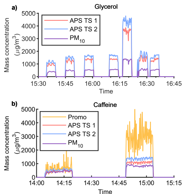
Figure 8. Comparison of the micro-APC PM 10 to standard laboratory equipment using a) liquid sample and a b) solid sample dissolved in liquid. The micro-APC performs significantly better for solid aerosols. (Promo data is unavailable for the glycerol sample.)
