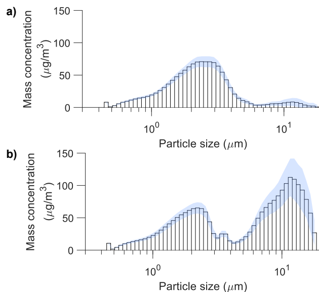
Figure 9. Mass distribution (as reported by APS 2) of caffeine dissemination on two different days with relative humidity a) < 80% and b) about 90%. The shaded area represents that standard deviation.
