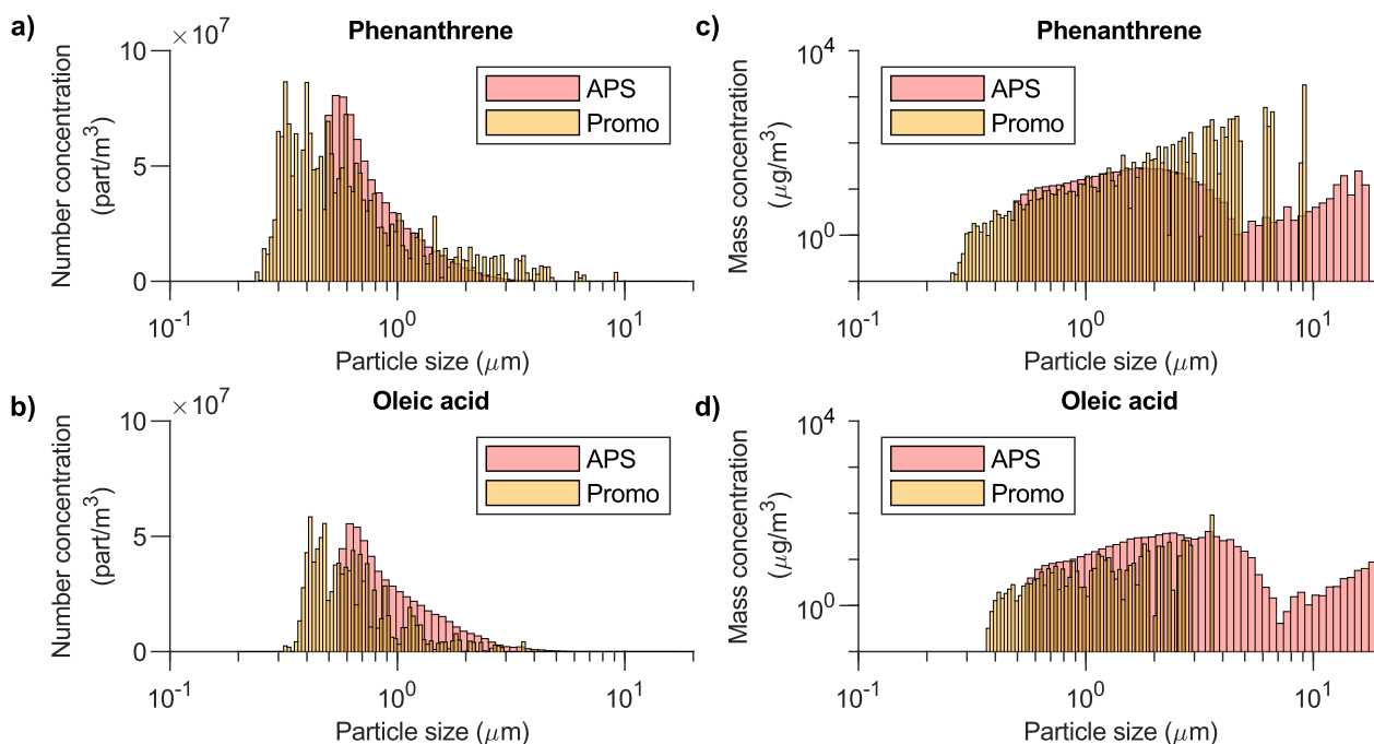
Figure 7. The number (a and b) and mass (c and d) size distributions from APS 1 and the Promo for oleic acid and for phenanthrene is compared for the average 10 s interval. The Promo distribution from phenanthrene has a long tail leading to a highly varying mass distribution shifted to larger particles compared to that of the APS. This trend is not observed for oleic acid, leading to the variation of the ratio of masses reported by the two instruments.
