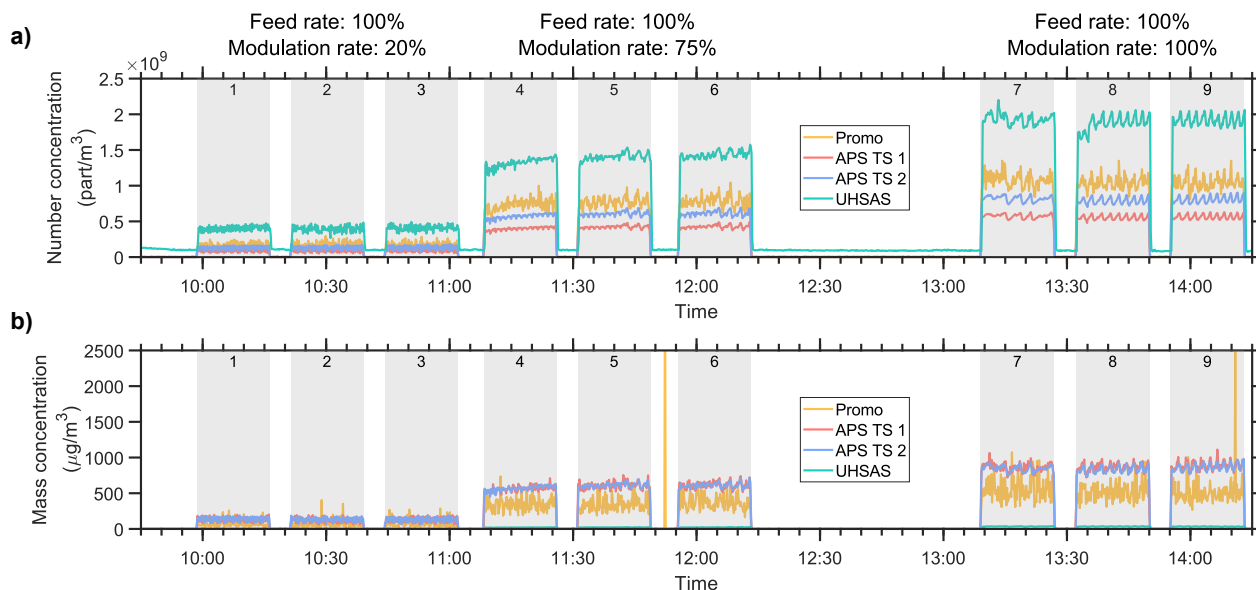
Figure 6. The number and mass concentrations for the two APSes, the Promo, and the UHSAS during the dissemination of 5 g/L oleic acid in ethanol. Each dissemination event is labeled with a number.
