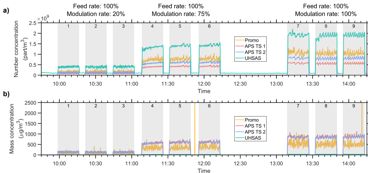
Figure 6. The number and mass concentrations for the two APSes, the Promo, and the UHSAS for during the dissemination of 5 g/L oleic acid in ethanol . Each dissemination event is labeled with a number. The data shown in Fig. 5 is from event 4.
