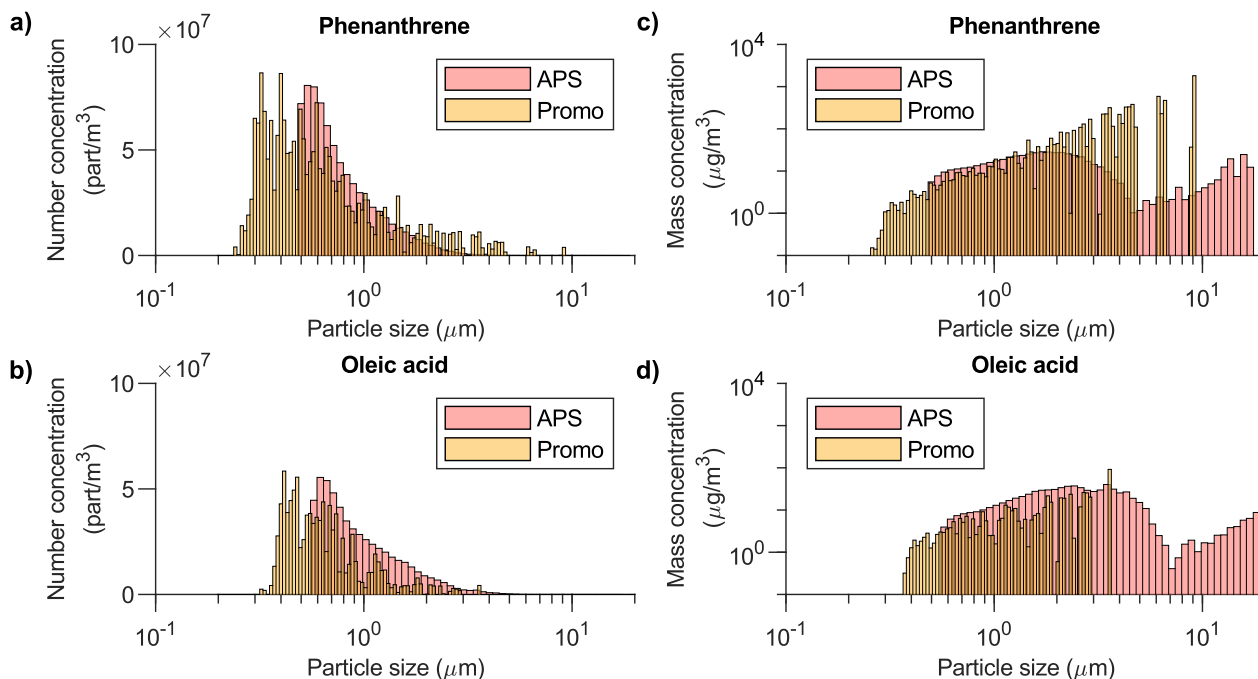
Figure 7. The number (left a and b) and mass (right c and d) size distributions from APS 1 and the Promo for oleic acid and for phenanthrene is compared for the average 10 s interval. The Promo distribution from phenanthrene has a long tail leading to a highly varying mass distribution shifted to larger particles compared to that of the APS. This trend is not observed for oleic acid, leading to the variation of the ratio of masses reported by the two instruments.
