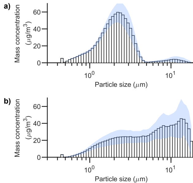
Figure 10. Comparison of size distribution (as reported by TSI-APS 33212) between a) liquid (Caffeine, 5 g/L, top ) and b) dry (Arizona Test Dust, bottom ) generation methods. The shaded area represents that standard deviation.
