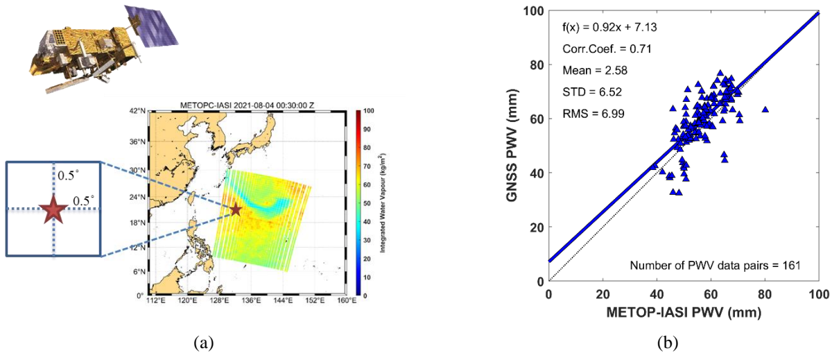
315 Figure 7. Comparison of shipborne GNSS PWV against satellite MetOp-IASI PWV. (a) The satellite-borne PWV values were calculated using the average within \pm 0.5^\circ of latitude and longitude from the vessel's location marked by a red star at the time of observation. (b) Scatter diagram of shipborne GNSS PWV and satellite MetOp-IASI PWV. The legend shows the equation for a linear relationship, correlation coefficient, mean, standard deviation (STD), and root mean square (RMS). The thick blue line and black dotted line represent the linear regression line and the reference line ( y=x ), respectively. (Image source of MetOp spacecraft: https://www.eumetsat.int/our-satellites/metop- 320 series)
