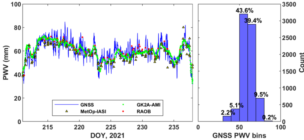
195 Figure 4. (Left) PWV time series for shipborne GNSS, radiosonde (RAOB), low Earth orbit (MetOp-IASI), and geostationary satellites (GK2A-AMI) for the 27 days from DOY 211 (July 30) to DOY 237 (August 25). (Right) Histogram for shipborne GNSS PWV count.
