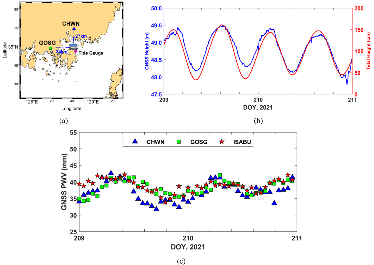
170 Figure 2. PWV from GNSS ground stations and R/V ISABU. (a) The distribution of two GNSS ground stations (CHWN and GOSG), R/V 175 ISABU, and a tide station. (b) Height variation from the vessel's GNSS and tide gauge from DOY 209 to 210, 2021. (c) The time series of PWV was derived from the CHWN, GOSG, and R/V ISABU from DOY 209 to 210, 2021.
