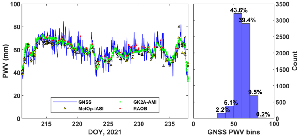
Figure 4. (Left) PWV time series for shipborne GNSS, radiosonde (RAOB), low Earth orbit (MetOp-IASI), and geostationary satellites (GK2A-AMI) for the 27 days from DOY 211 (July 30) to DOY 237 (August 25). (Right) Histogram for shipborne GNSS PWV count.
