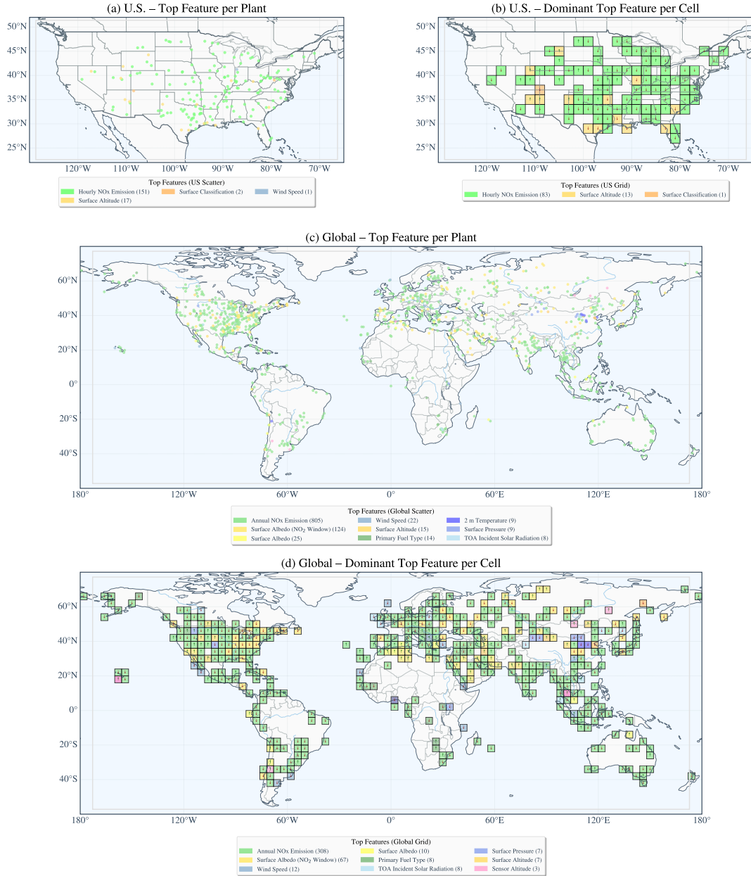
Figure D2. Plant-level feature importance via SHAP score. (a,c) Plant-level scatter: each point is a power plant colored by its most influential feature. (b,d) Grid-mode maps: within each cell ( 2^\circ U.S.; 4^\circ global), the color marks the modal top feature. Legend counts (in parentheses) report the number of plants (a, c) or grid cells (b, d) for which that feature ranks first; the legend lists the top 9 features, so a small number of plants whose top feature falls outside this list are plotted but not enumerated. SHAP values are computed on the held-out test split of the dataset. Dataset: modeling subset (Sect. 3.3; 171 U.S. plants, n = 189,713 observations; 1,065 global plants, n = 161,118 observations); the held-out test split contains n = 37,943 U.S. and n = 32,224 global observations.
