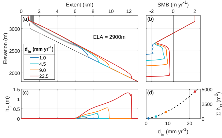
Figure B2. Steady-state glaciers for variable debris input rates d_{in} (1.0, 4.5, 9.0, and 22.5 mm yr -1 ) with otherwise the same parameter setting as in Fig. 2 with the resulting steady-state (a) glacier surface geometries, (b) surface mass balance, and (c) debris cover thickness h_D . The gray area marks the debris input area below the headwall and the englacial debris transport trajectory.
