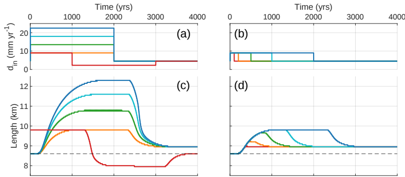
Figure C1. Debris input step-change experiments deb-1: (a) increasing d_{in} at time zero from 4.5 \text{ mm yr}^{-1} to double (orange), triple (green), quadruple (cyan), quintuple (blue), as well as doubling followed by halving (red) after 1000 years. After 2000 years the debris input is reset to the initial value. (b) Varying duration of debris input doubling d_{in} experiment: 100 (red), 200 (orange), 500 (green) 1000 (cyan), and 2000 years (blue). (c,d) Corresponding glacier length responses.
