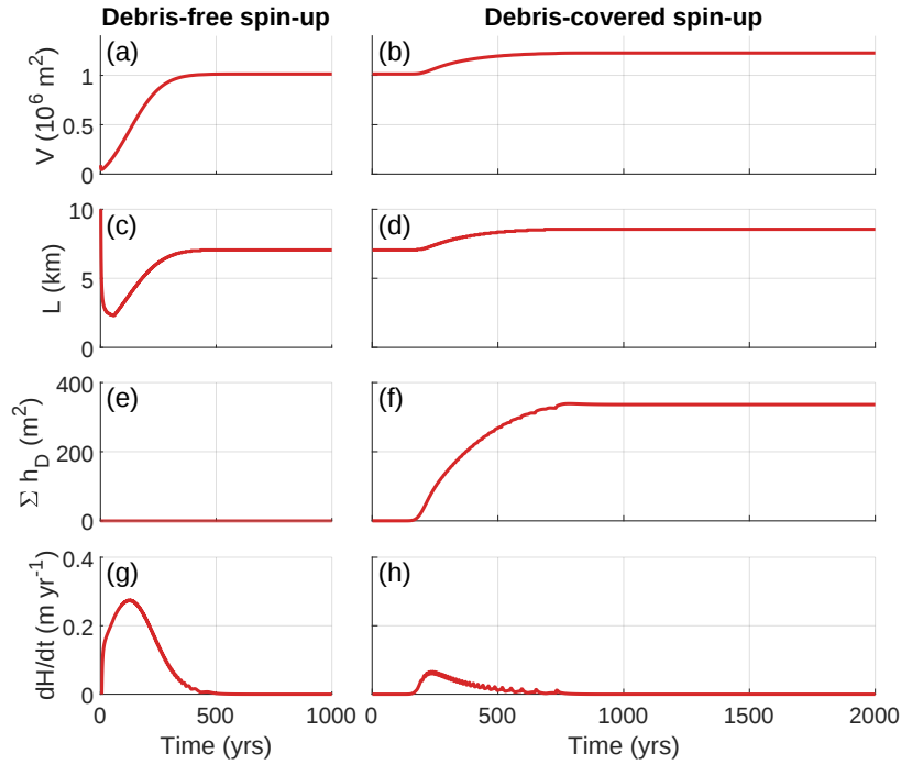
Figure B1. Full model spin-up procedure: (a & b) ice volume, (c & d) glacier length, (e & f) total supraglacial debris volume, and (g & h) glacier-averaged change in ice thickness ( \partial H/\partial t ) evolving over two spin-up periods. First, an initial debris-free spin-up period of 1000 years, initialized from 10 m of ice thickness along the entire bed at time 0. Second, a steady debris input is introduced and the simulation is run for 2000 years, when the modelled glacier has reached a steady-state for any steady-state parameter set.
