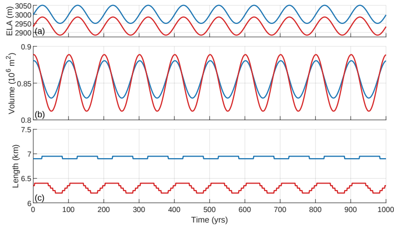
Figure B5. Sine wave climate experiment comparing a clean-ice (red) to a debris-covered (blue) glacier. (a) ELA oscillating with an amplitude of 50 m and \lambda = 100 yr around 2935 (clean-ice) and 3000 m a.s.l. (debris-covered). This corresponds to equal steady-state volumes, enabling a direct comparison of dynamic response: (b) glacier volume and (c) length response.
