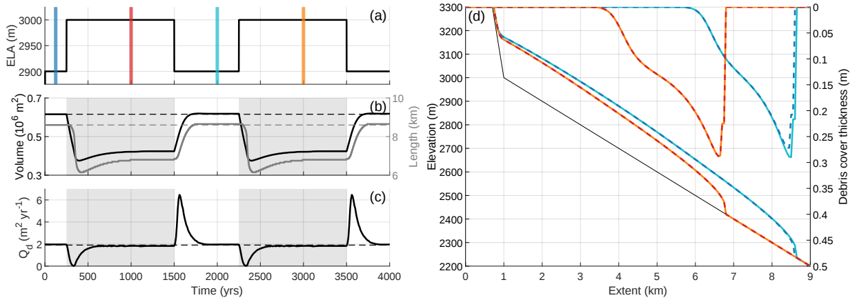
Figure C3. Repeated 100 meter ELA step-change experiment: (a) ELA forcing and markings for the four steady-states shown in (d). (b) Glacier volume and length response, (c) near-terminus debris flux response. (d) Four steady-state glacier geometries as marked with the colored bars in (a), at 2900 m (blue, cyan) and 3000 m (red, orange) ELA.
