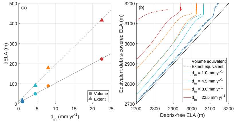
Figure 3. Experiments steady-2 & clim-2: (a) Relationship of steady-state debris input with dELA (dELA = equivalent debris-covered ELA – debris-free ELA, measured at 2700 m debris-free ELA) for volume and extent equivalent ELAs, showing a roughly linear relationship. (b) Debris-free ELA compared to debris-covered ELA, showing the debris-covered ELA required to result in a volume or extent equivalent to the debris-free case. Four cases are shown, with a debris input of 1.0 \text{ mm yr}^{-1} (blue), 4.5 \text{ mm yr}^{-1} (cyan), 8.0 \text{ mm yr}^{-1} (orange), and 22.5 \text{ mm yr}^{-1} (red).
