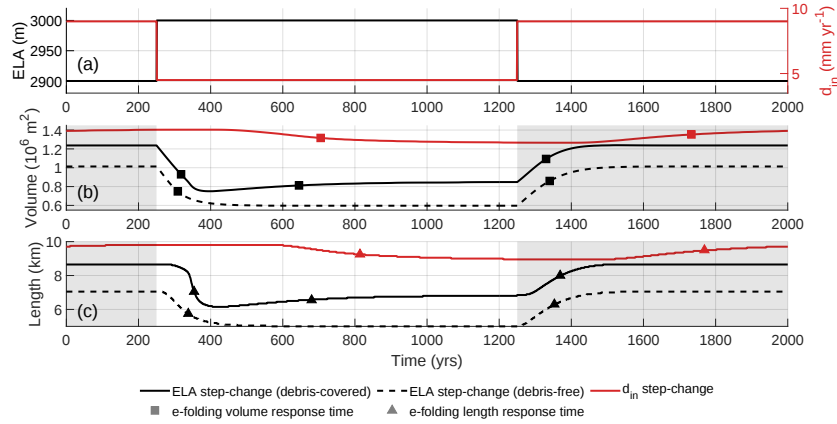
Figure 5. Experiments clim-1 & deb-1: Response times to a step-change in ELA (Exp. clim-1), for a debris-covered (black solid line) and a debris-free glacier (black dashed line), and to a step-change in debris input rate d_{in} (red solid line; Exp. deb-1): (a) forcing, (b) volume response and e-folding volume response times, and (c) length response and e-folding length response time. The symbols mark the time of reaching the response time (e-folding time) after the step-changes.
