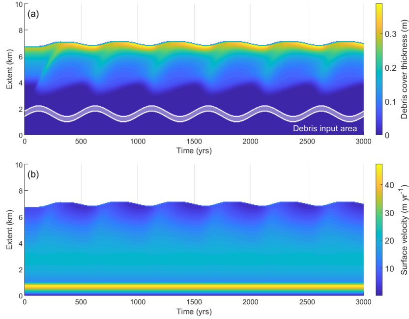
Figure B4. Varying debris input position in a sine wave (wavelength = 500 years, amplitude = 800 m with 1000\text{ m} \leq x_d \leq 1800\text{ m} , ELA = 3000 m). (a) Debris cover thickness response and (b) surface velocity over time and along-glacier extent.
