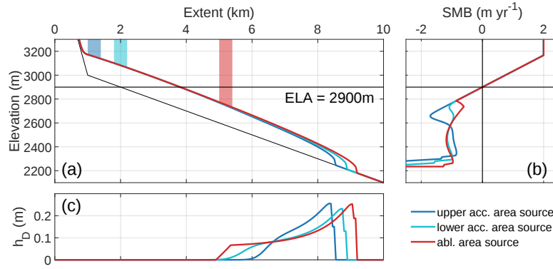
Figure B3. Steady-state glaciers for different debris input area locations (0, 800, and 4000 meters from headwall slope break) using the same debris input rate of 4.5 \text{ mm a}^{-1} and an ELA of 2900m with the resulting steady-state glacier (a) surface geometries, (b) surface mass balance, and (c) debris cover thickness h_D .
