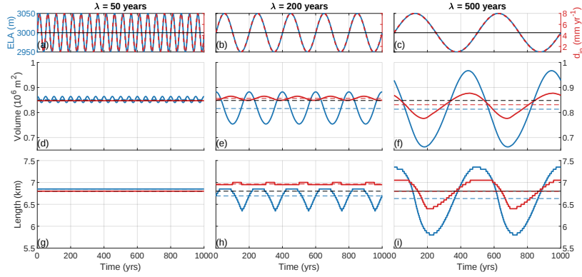
Figure 7. Experiments clim-3 & deb-2deb-3 : Comparing glacier volume and length response to sine variations in climate (ELA, blue solid lines; Exp. clim-3) and debris input ( d_{in} , red lines; Exp. deb-2deb-3 ) forcing with three different period lengths: (a,d,g) 50 years, (b,e,h) 200 years, and (c,f,i) 500 years. Dashed lines indicate volumes and lengths of a steady-state glacier (black) with the corresponding time-constant mean ELA and debris input rates, compared to mean volumes and lengths of the transient-state glaciers (blue and red lines).
