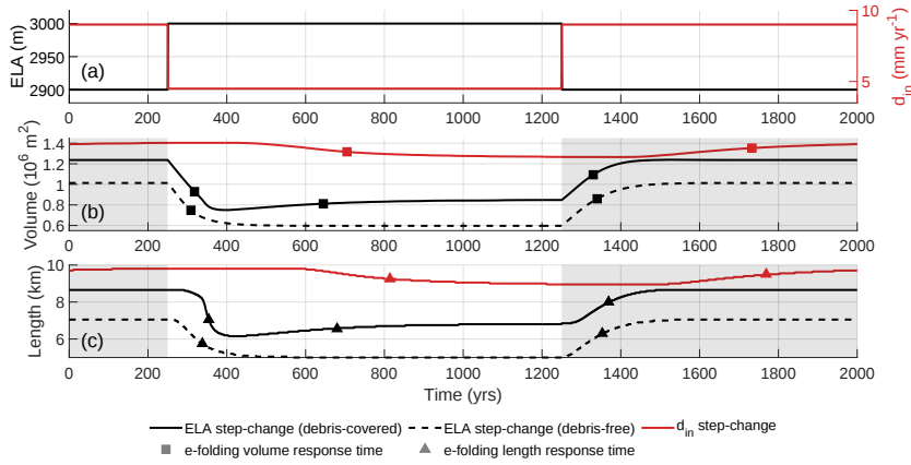
Figure 5. Experiments clim-1 & deb-1: Response times to a step-change in ELA (Exp. clim-1), for a debris-covered (black solid line) and a debris-free glacier (black dashed line), and to a step-change in debris input rate d_{in} (red solid line; Exp. deb-1): (a) forcing, (b) volume response and e-folding volume response times, and (c) length response and e-folding length response time. The symbols mark the time of reaching the response time (e-folding time) after the step-changes.
