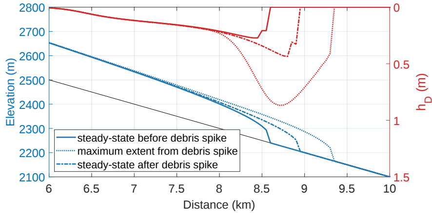
Figure C2. Geometry adjustment in short-term debris input spike experiment (Exp. deb-3 deb-2 ; Fig. 6): glacier geometry (blue) and debris cover thickness (red) at three relevant points in time: at the steady-state before the first spike event (solid lines), at maximum extent caused by the spike (dotted lines), and at the new steady-state after the event (dashed lines).
