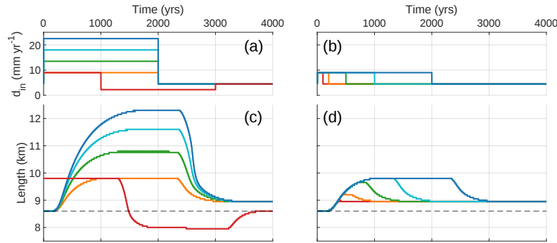
Figure C1. Debris input step-change experiments deb-1: (a) increasing d_{in} at time zero from 4.5 \text{ mm yr}^{-1} to double (orange), triple (green), quadruple (cyan), quintuple (blue), as well as doubling followed by halving (red) after 1000 years. After 2000 years the debris input is reset to the initial value. (b) Varying duration of debris input doubling d_{in} experiment: 100 (red), 200 (orange), 500 (green) 1000 (cyan), and 2000 years (blue). (c,d) Corresponding glacier length responses.
