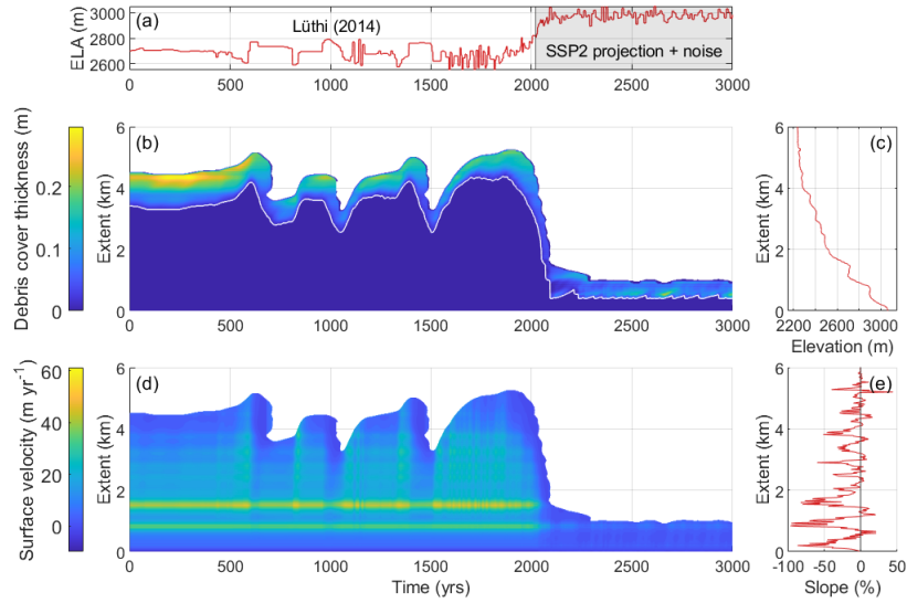
Figure 11. Experiment clim-5b: Debris-covered transient response to complex climate forcing on an undulated bed topography: (a) ELA forcing derived from reconstructed climate history (Lüthi, 2014) and , SSP2-4.5 scenario (Masson-Delmotte et al., 2021), and adjusted to produce a realistically sized glacier. (b) debris cover thickness response, (c) along-glacier bed elevation, (d) surface velocity response over the extent of the glacier on a Zmuttgletscher-like bed topography (Fig. 10), and (e) along-glacier bed slope. The white line in (b) marks the first grid point where debris thickness > 0.01 m, i.e. where debris starts emerging.
