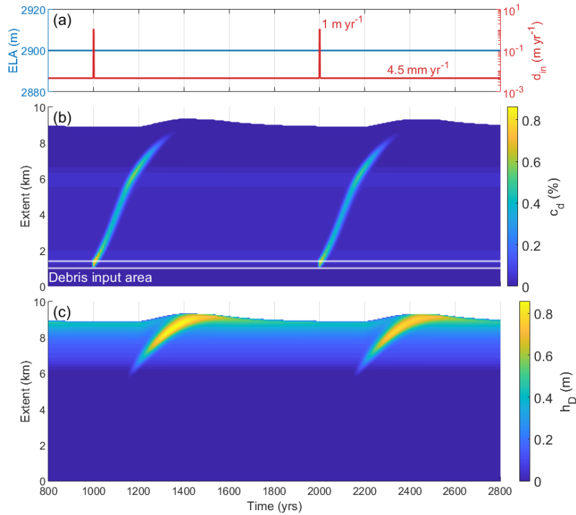
Figure 6. Experiment deb-3 deb-2 : Short-term debris input spike experiment (Exp. deb-3 deb-2 ): (a) constant ELA and spike debris input rate forcing, (b) resulting depth-averaged englacial debris concentration over time and glacier extent, and (c) resulting debris cover thickness over time and glacier extent. During the spike event, 1 meter of debris is deposited on the glacier over 1 year. In the intermediate periods the standard debris input rate of 4.5 \text{ mm yr}^{-1} is used.
