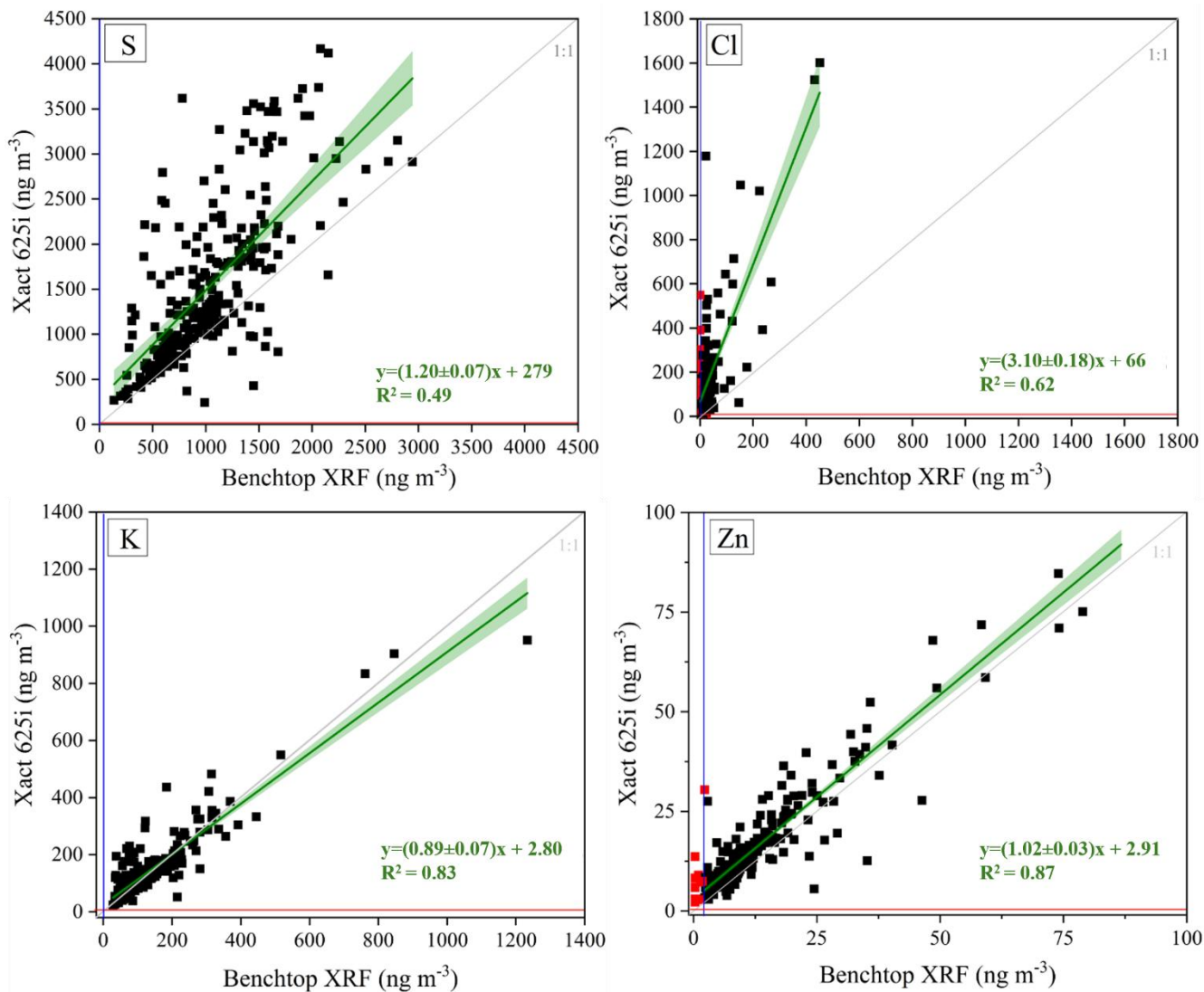
440 Figure 7: Comparison of elemental concentrations in ng m -3 for S, Cl, K and Zn for the CAO-NIC station. The blue lines indicate the LOQ thresholds for the benchtop XRF spectrometer, while the red lines represent the corresponding thresholds for the Xact 625i continuous elemental monitor. The grey line represents the 1:1 reference line, while the green line represents the linear regression fit. Data points below the LOQ were excluded from the analysis to ensure accurate comparison between the two instruments and are highlighted in red, distinguishing measurements with higher uncertainty.
