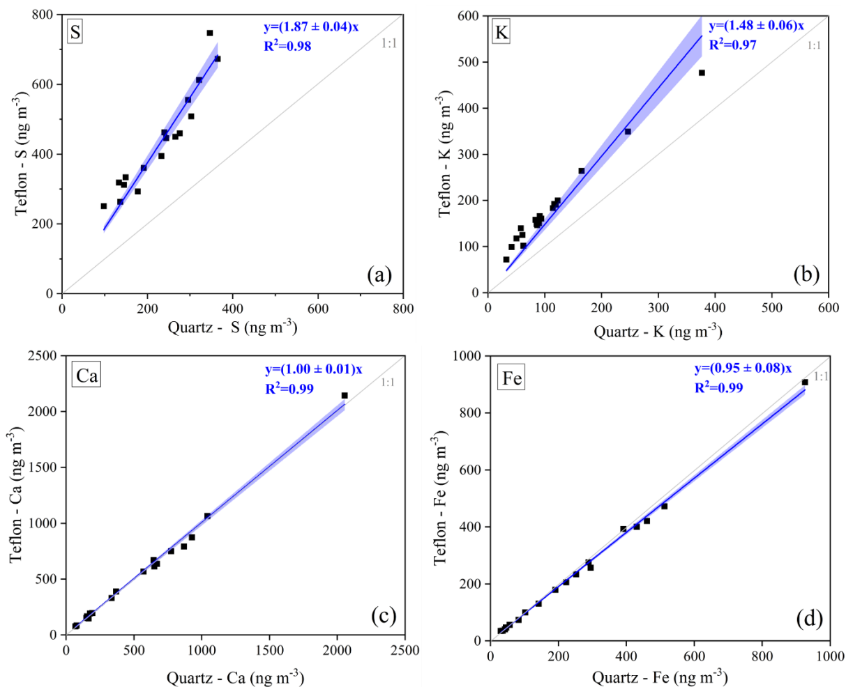
310 Figure 3: Comparison of Elemental Concentrations: Teflon vs. Quartz Filters of S (a), K (b), Ca (c) and Fe (d) using data from the 315 dedicated measurement campaign conducted between January 13 and January 31, 2024, at the ATH-DEM station to explore potential differences in elemental composition across filter substrates. The shaded blue regions denote the 95% confidence intervals of the fitted regression slopes.
