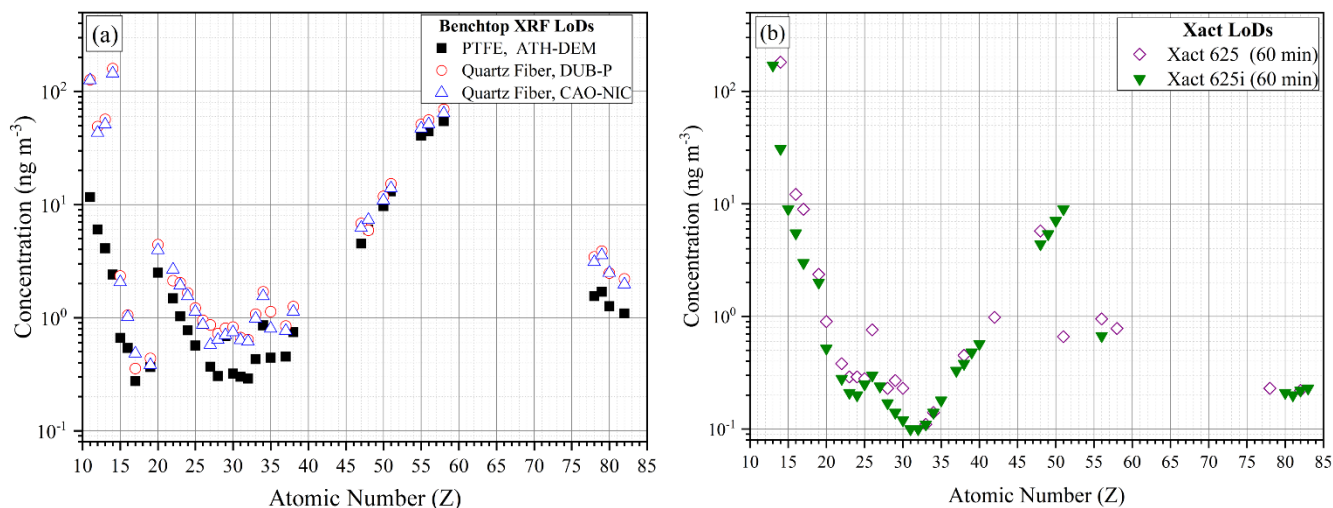
235 Figure 2: a) Limits of detections for the benchtop XRF spectrometer, for PTFE and Quartz fiber filters in ng m -3 . b) Limits of detections for the Xact 625 and 625i for 60-minute time resolution.
