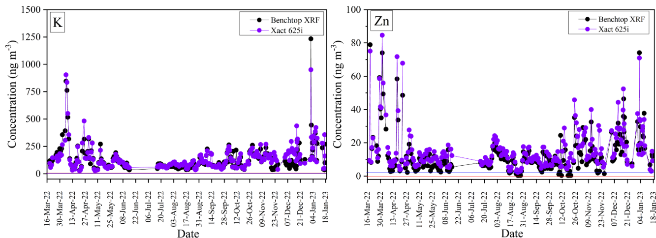
440 Figure 8: Time series graphs comparing K and Zn concentrations in \text{ng m}^{-3} from 16 March 2022 to 18 January 2023. The red and blue lines indicate the LOQ thresholds for the Xact 625i and the benchtop XRF spectrometer, respectively.
