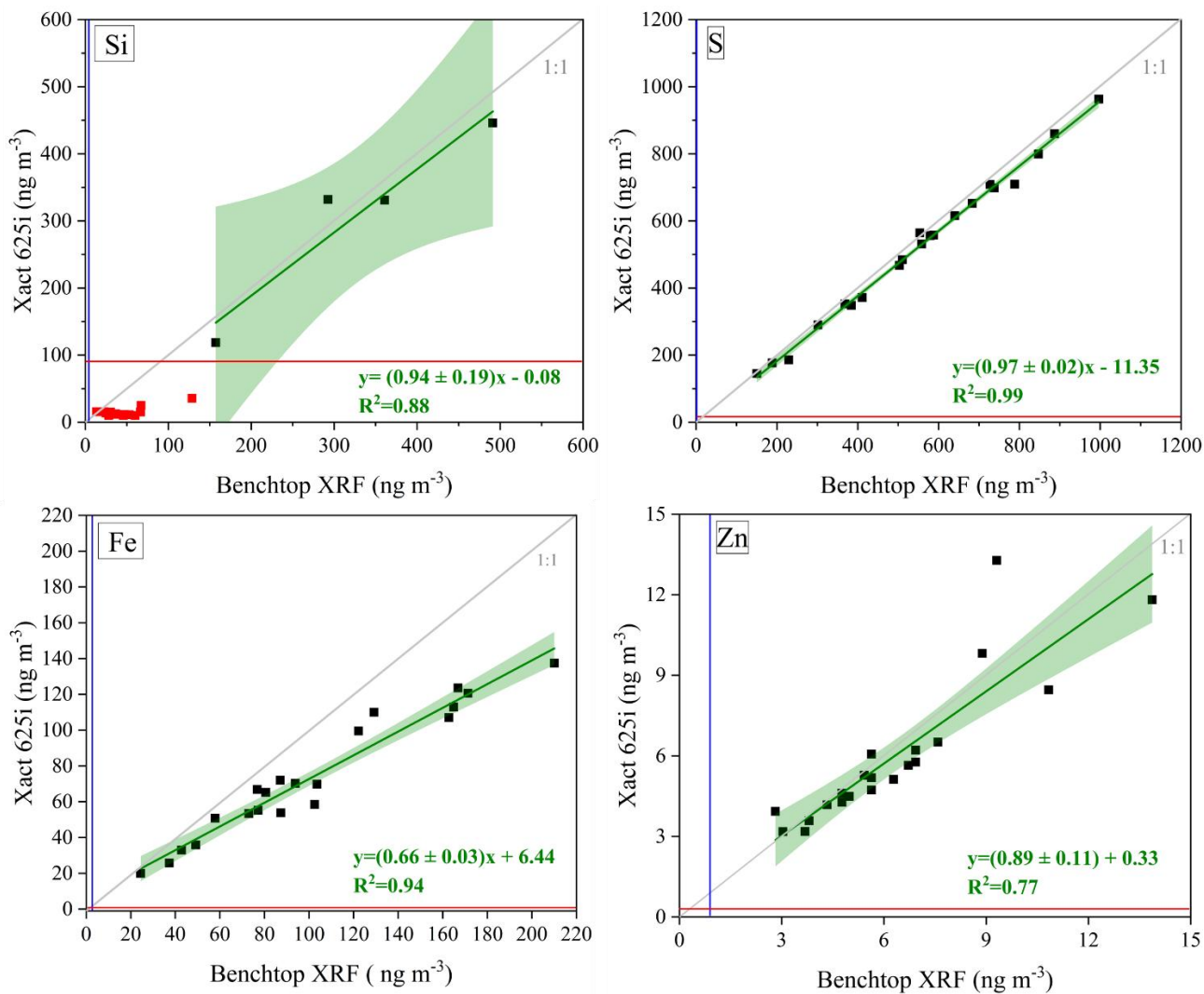
395 Figure 5: Comparison of elemental concentrations in \text{ng m}^{-3} for Si, S, Fe, and Zn for the ATH-DEM station. The blue lines indicate the LOQ threshold for the benchtop XRF spectrometer, while the red lines represent the corresponding threshold for the Xact 625i continuous elemental monitor. The grey line represents the 1:1 reference line, while the green line represents the linear regression fit. Data points below the LOQ were excluded from the analysis to ensure accurate comparison between the two instruments and are highlighted in red, distinguishing measurements with higher uncertainty.
