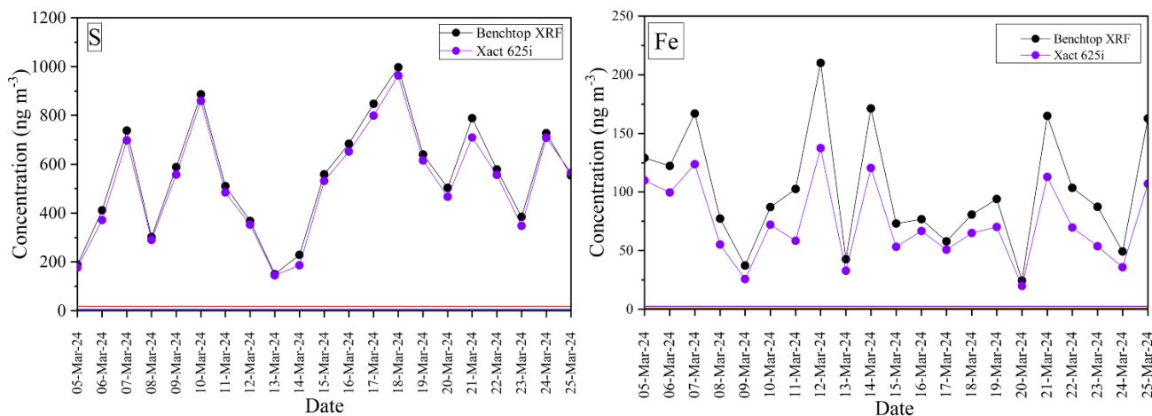
400 Figure 6: Time series graphs comparing S and Fe concentrations ( \text{ng m}^{-3} ) from March 5 to 25, 2024, show strong agreement for S, while Fe exhibits a consistent deviation, with lower values reported by the Xact 625i. This suggests differences in the calibration curves for heavier elements between the instruments. The red and blue lines indicate the LOQ thresholds for the Xact 625i and the benchtop XRF spectrometer, respectively.
