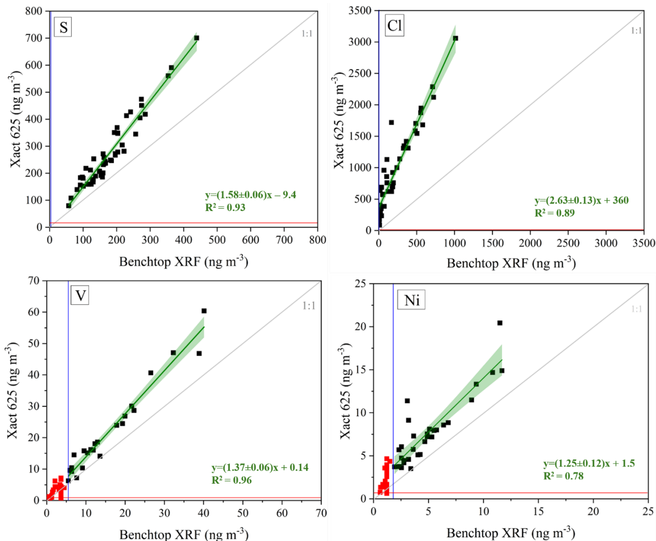
465 Figure 9: Comparison of elemental concentrations in \text{ng m}^{-3} for S, Cl, V and Ni for the DUB-P station. The blue lines indicate the LOQ thresholds for the benchtop XRF spectrometer, while the red lines represent the corresponding thresholds for the Xact 625 continuous elemental monitor. The grey line represents the 1:1 reference line, while the green line represents the linear regression fit. Data points below the LOQ were excluded from the analysis to ensure accurate comparison between the two instruments and are highlighted in red, distinguishing measurements with higher uncertainty.
