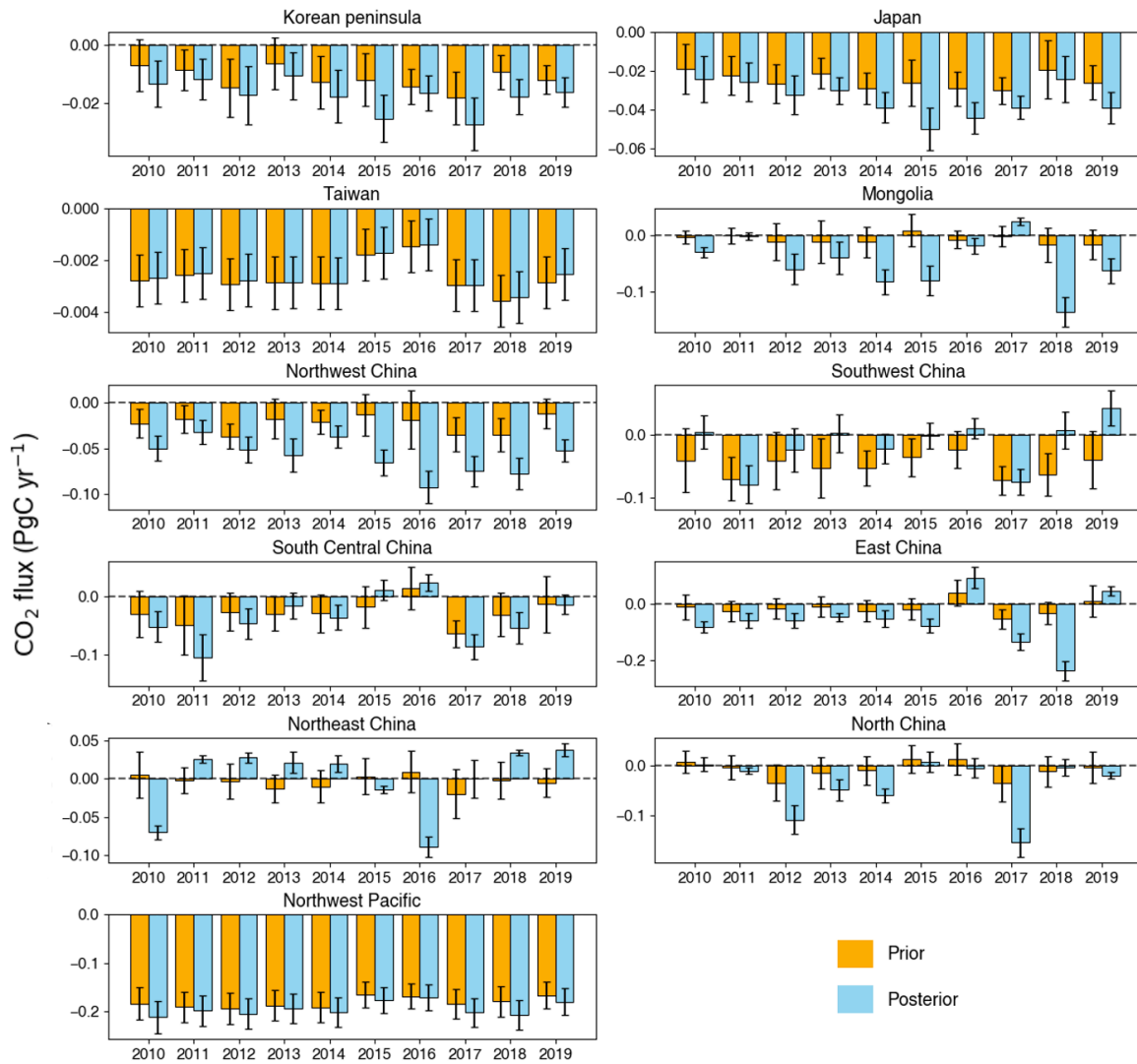
420 Figure 4. Annual regional CO 2 fluxes over East Asia for the period 2010–2019, estimated from the prior (orange) and posterior (blue) fluxes. Each panel represents a different region, and negative values indicate net CO 2 uptake (sink). Error bars represent the uncertainty of the flux estimates.
