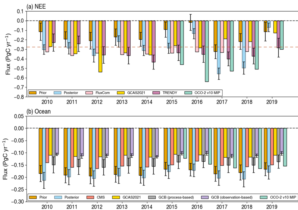
485 Figure 5. Comparison of prior and posterior flux estimates with other flux products from 2010 to 2019. (a) NEE and (b) Ocean carbon flux over East Asia. Bars indicate annual mean fluxes from each dataset. Error bars represent the uncertainty ranges for the prior and posterior estimates, while those for TRENDY and GCB Ocean denote the inter-model standard deviations. The orange dashed line is the NEE of East Asia for 2000-2020 calculated by RECCAP-2 (Wang et al., 2024)
