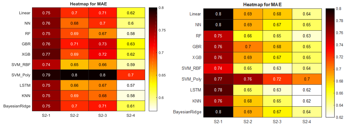
Figure 6: Heatmap of performance metrics ( R^2 , MSE, MAE) for one-month-ahead SPI prediction ( SPI_{t+1} ) at the Anzali (right columns) and Zabol (left columns) stations under four temporal memory scenarios (S2-1 to S2-4). The results clearly demonstrate that for most models, particularly LSTM, increasing the memory length from 3 months (S2-1) to 12 months (S2-4) leads to a substantial increase in R^2 and a reduction in error, underscoring the importance of longer-term historical data.
