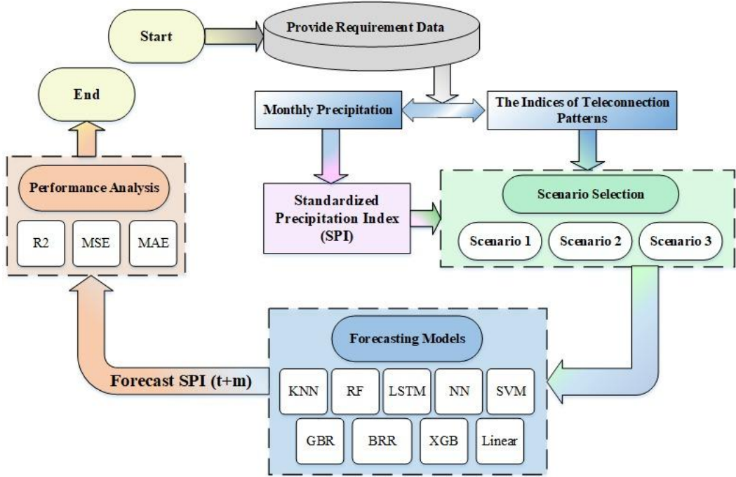
Figure 3: Methodological framework of the research for short-term drought forecasting in Iran. This flowchart illustrates the step-by-step process, from the ingestion of raw data (precipitation and teleconnection indices), calculation of the SPI, design of input scenarios, training of a suite of machine learning models, to the final performance evaluation and selection of the optimal model.
