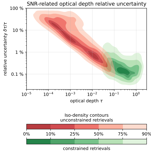
Figure 10. SNR-related cloud optical depth relative uncertainty against cloud optical depth for constrained (green contours) and unconstrained (red contours) backward retrievals. The darker the contour, the larger the number of measurements. For each color, the total colored area correspond to 90 % of the observations. For each color, the darkest contour corresponds to 10 % of the observations, where measurements are the denser.
