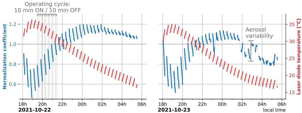
Figure 5. Time series of laser diode temperature (Celsius degrees, red line) and normalization coefficient (arbitrary unit, blue line) for two nights (local time) of flight ST2_C1_02_STR1. The normalization coefficient is the instrumental constant arbitrarily scaled to 1 at a given time. On the left panel (October 22, 2021) the operating cycle (10 minutes ON/10 minutes OFF) is highlighted in grey.
