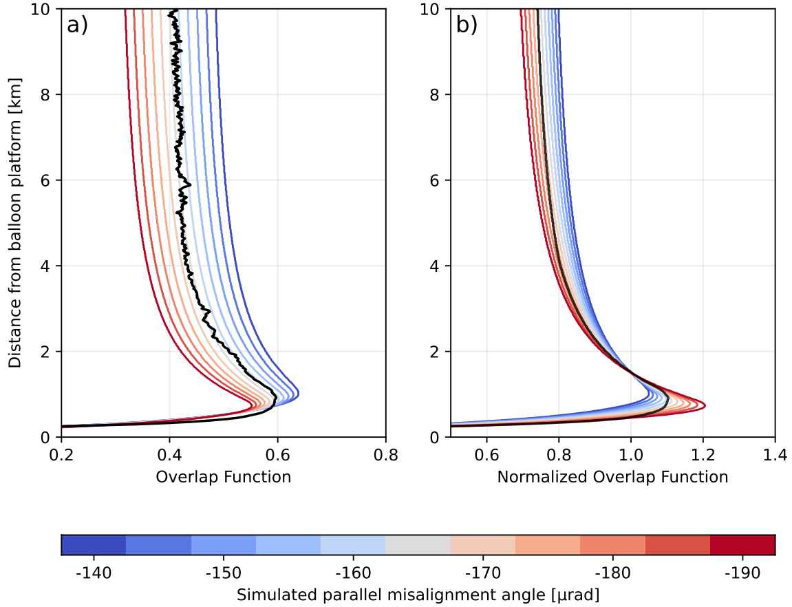
Figure 3. a) Simulated overlap functions for different parallel misalignment angles between the emission and the reception optical channels. The parallel misalignment angle varies from -140 (blue line) to -190 \mu\text{rad} (red line). Negative values correspond to slightly converging optical axes. The solid black line is a reference clear sky profile used to derive the empirical overlap correction for a given instrument: it is the ratio of the mean lidar profile over a 3 h cloud-free window to a synthetic Rayleigh lidar profile. b) Same overlap functions (blue to red lines) normalized at a distance of 1.5 km from the platform, along with the empirical overlap correction (smooth solid black line) derived from the reference clear-sky profile, normalized at the same distance.
