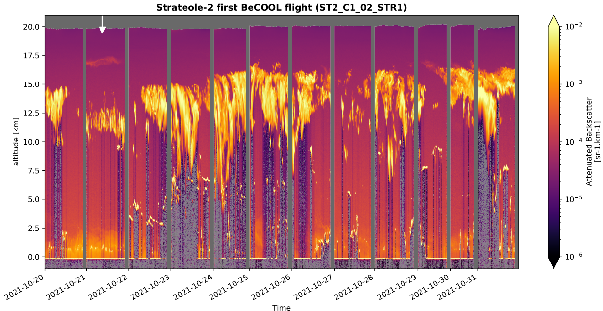
Figure 6. Lidar cross section (time vs altitude) of the attenuated backscatter signal for the first BeCOOL flight of Strat ole2 2021-2022 scientific campaign, between October 20, 2021 and October 31, 2021. Vertical grey lines separate two consecutive nights (BeCOOL is not operated during ). The upper horizontal grey-shaded area stands for no data. The upper white arrow is pointing the time corresponding to the profile retrieved in section 4.
