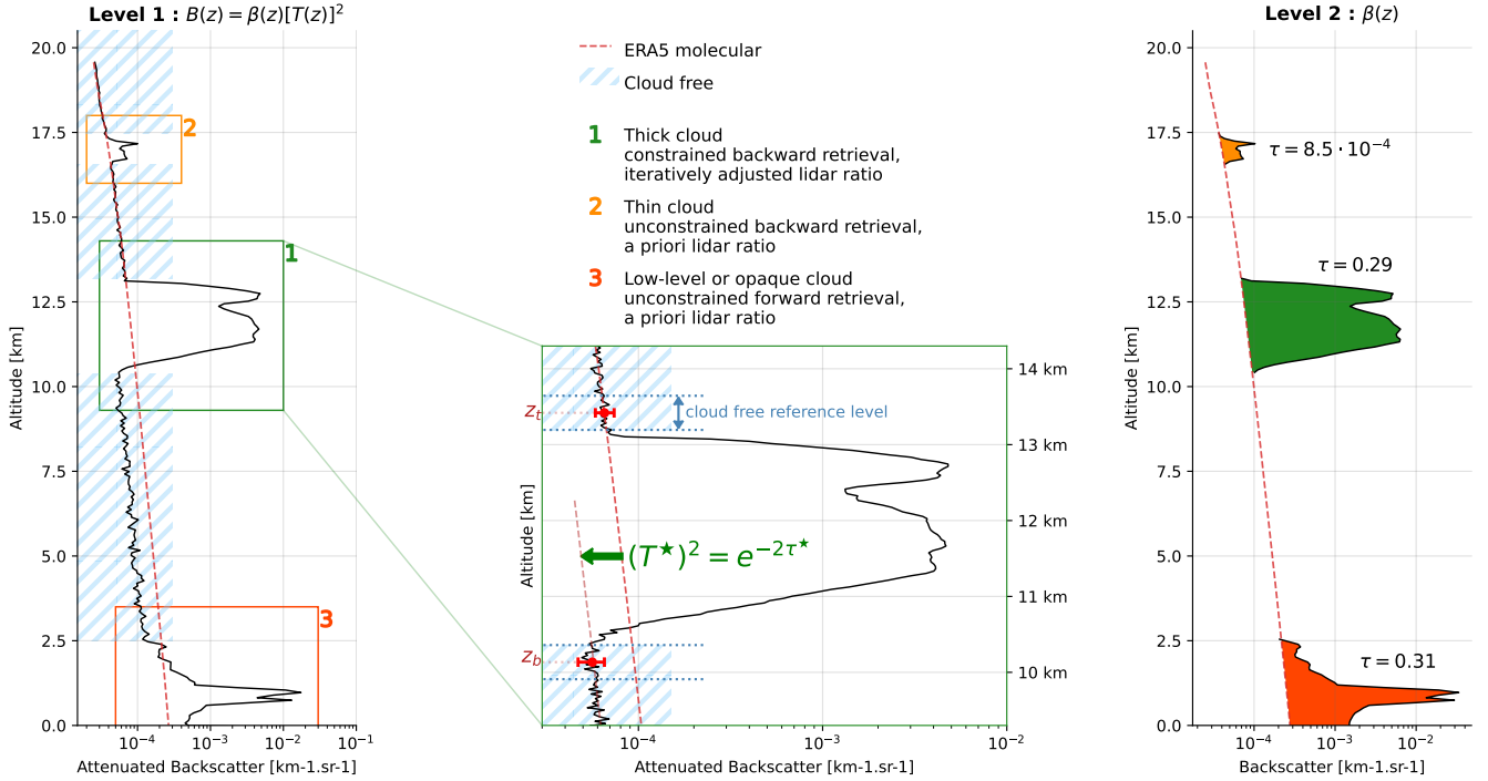
Figure 7. 10-min averaged lidar profile on October 21, 2021 (white arrow on Figure 6). The attenuated backscatter profile \beta[T(z)]^2 is plotted on the left panel, the backscatter profile \beta(z) on the right panel (the red dashed line is corresponding to \beta_m(z) ). The middle panel is a zoom of the left panel for the cloud in the middle of the profile. The upper and lower red dots correspond respectively to the values of the averaged quantity ( B^r ) at the bottom ( z_b ) and the top ( z_t ) of the cloud. The red brackets show the lower ( B^{r-} ) and upper ( B^{r+} ) values of these reference quantities. The colored areas on the right panel materialize the optical depth for backward constrained retrieval (green), backward unconstrained retrieval (orange) and forward unconstrained retrieval (dark orange).
