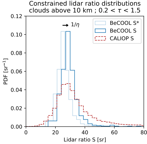
Figure 8. Probability distribution function (PDF) of the lidar ratio S . The light blue line corresponds to the PDF computed when the inversion of BeCOOL profiles is constrained, assuming no multiple scattering (the lidar ratio is noted S^* in this case). The red line corresponds to the PDF derived for the same category of clouds observed by CALIOP in the same region (optical depth between 0.2 and 1.5, altitude above 10 km). The dark blue line corresponds to the PDF computed when the inversion of BeCOOL profiles is constrained, assuming multiple scattering ( \eta correcting factor).
