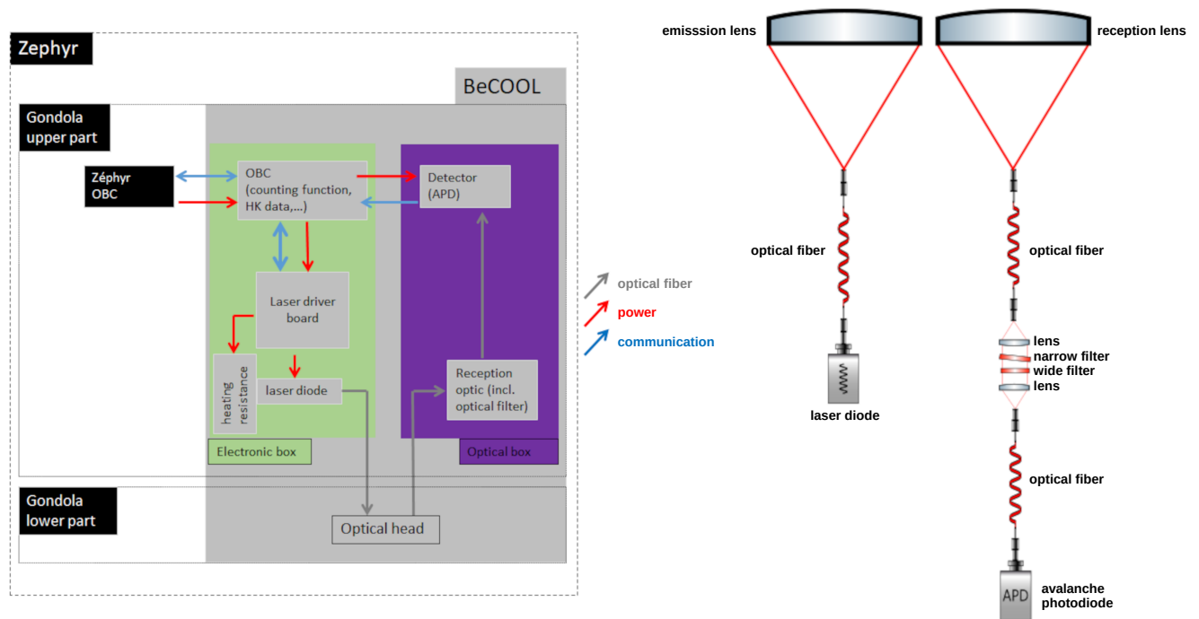
Figure 1. Left: BeCOOL block diagram. The green area corresponds to the electronic box. It includes the on-board computer (OBC) of the lidar. The purple area corresponds to the optical box (OB). It includes the avalanche photodiode (APD). The optical head includes the emission lens and the reception lens. Right: Optic schematic drawing showing both emission (left) and reception (right) channel .
