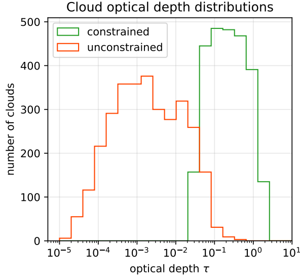
Figure 9. Distributions of retrieved cloud optical depth for the constrained (green line) and unconstrained (red line) backward retrievals.
