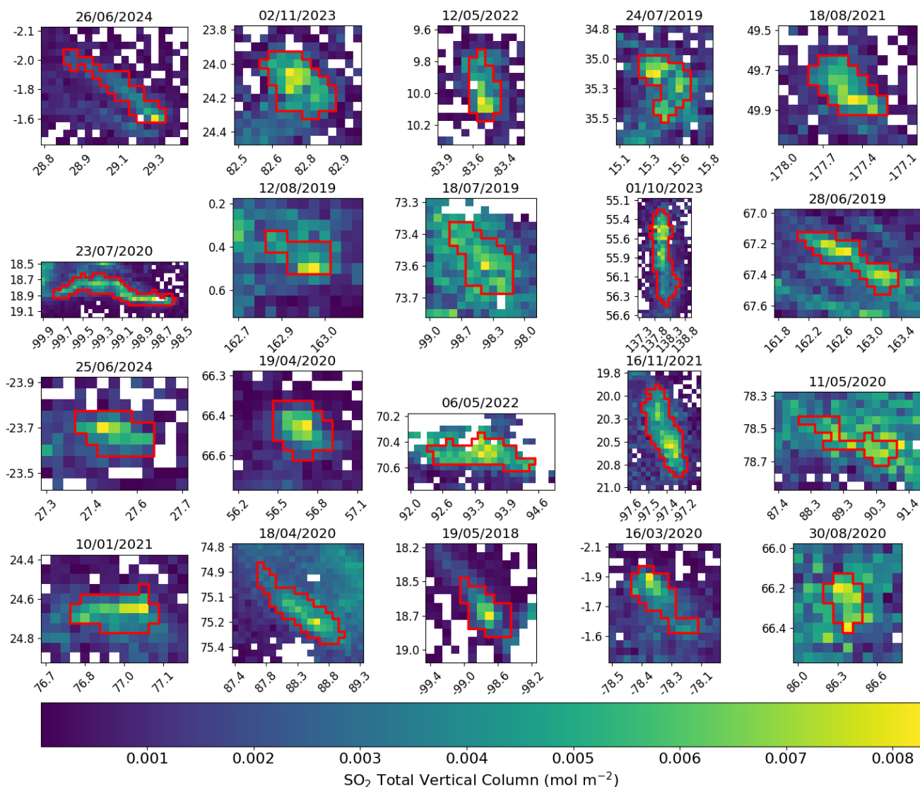
Figure 2. Examples of SO 2 plumes in the TROPOMI data and the predicted plume outline, shown as a red line. Warmer colours denote higher values The title of each image shows the date of observations and the x and y axes are longitude and latitude, respectively.
