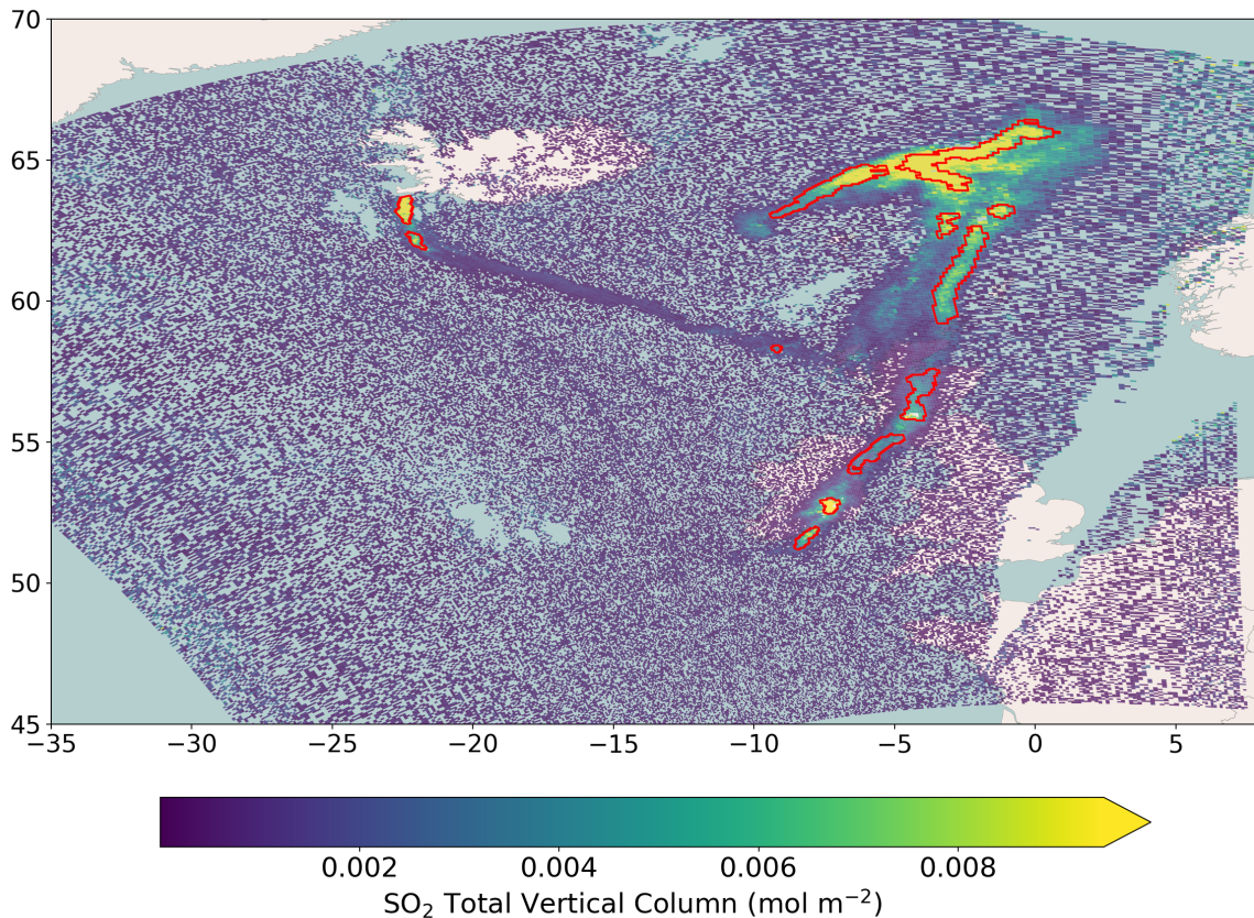
Figure 8. TROPOMI SO 2 total vertical column over the United Kingdom on 8th-24th August 2024 showing a plume from the Sundhnúkur volcano-Svartsengi volcanic system in Iceland.
