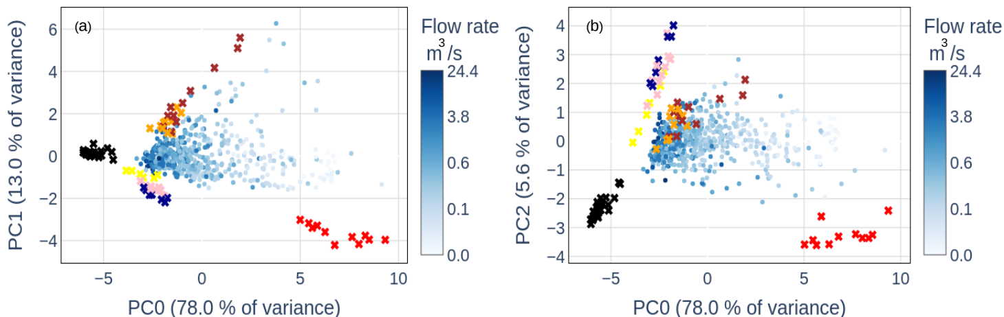
Figure 3. Results of the Principal Component Analysis (PCA) was performed using with streamwater samples (blue points, with outlet flow rate represented by the color scale). Source samples (cross symbols) were then are projected onto this PCA space: black crosses represent measurements from the gutters surface runoff collectors, while other colored crosses correspond to tributary sources. Each color correspond corresponds to a tributary, with the same colors of the crosses used in the Galabre map in Fig. 1 and Table 1. Multiple points with the same color indicate different sampling campaigns conducted within the same tributary. The association of colors to the different geologies and end-members are is: evaporite rocks (red), sedimentary rocks (yellow, pink, blue) and quaternary rocks (orange, brown), surface runoff (black).
