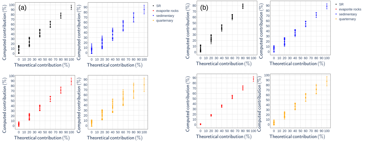
Figure A3. Results of the virtual test using the MB_{PCA,mean} (a) and MB_{mean} (b) End Member Modeling-Mixing Analysis methods.
