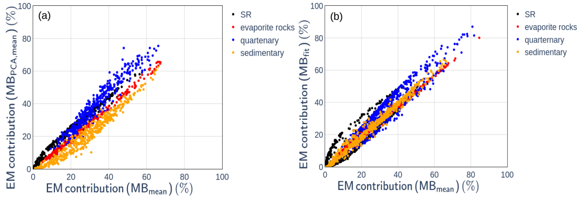
Figure A2. Comparison of end-member (EM) contributions obtained using different End Member Modeling-Mixing Analysis methods: (a) MB_{mean} versus MB_{PCA,mean} ; (b) MB_{mean} versus MB_{fit} .
