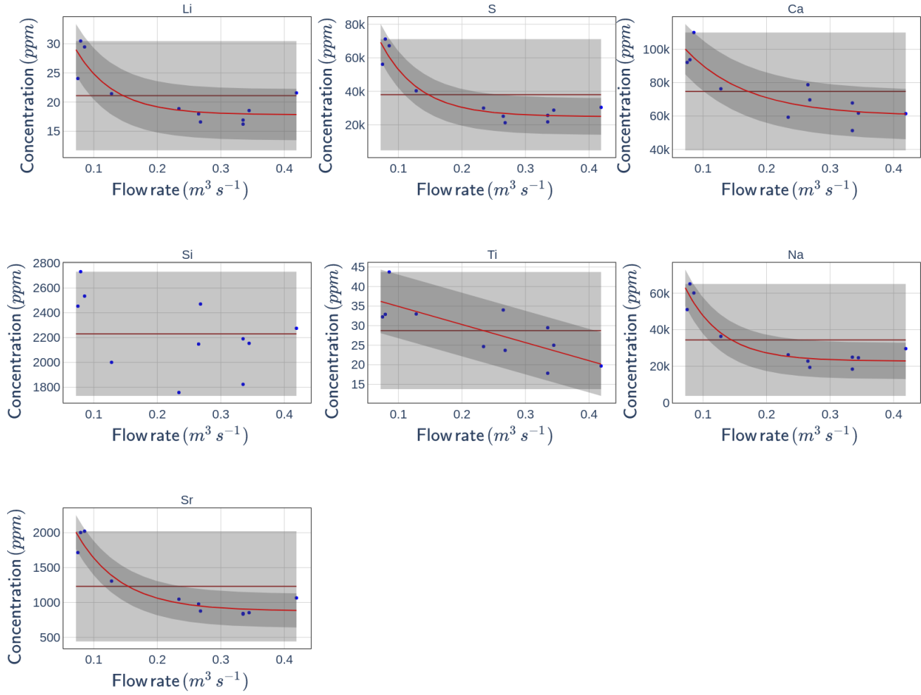
Figure A1. Relation between tracer concentration in the tributary "Arbres" and flow rate at the catchment outlet. Blue points are measurements, average concentration concentrations are brown lines, and decreasing exponential functions are red lines (for relation with r^2 > 0.5 R^2 > 0.5 ). Uncertainties associated with each relation are represented in grey, defined as the maximum deviation between the fitted curve and the measurements.
