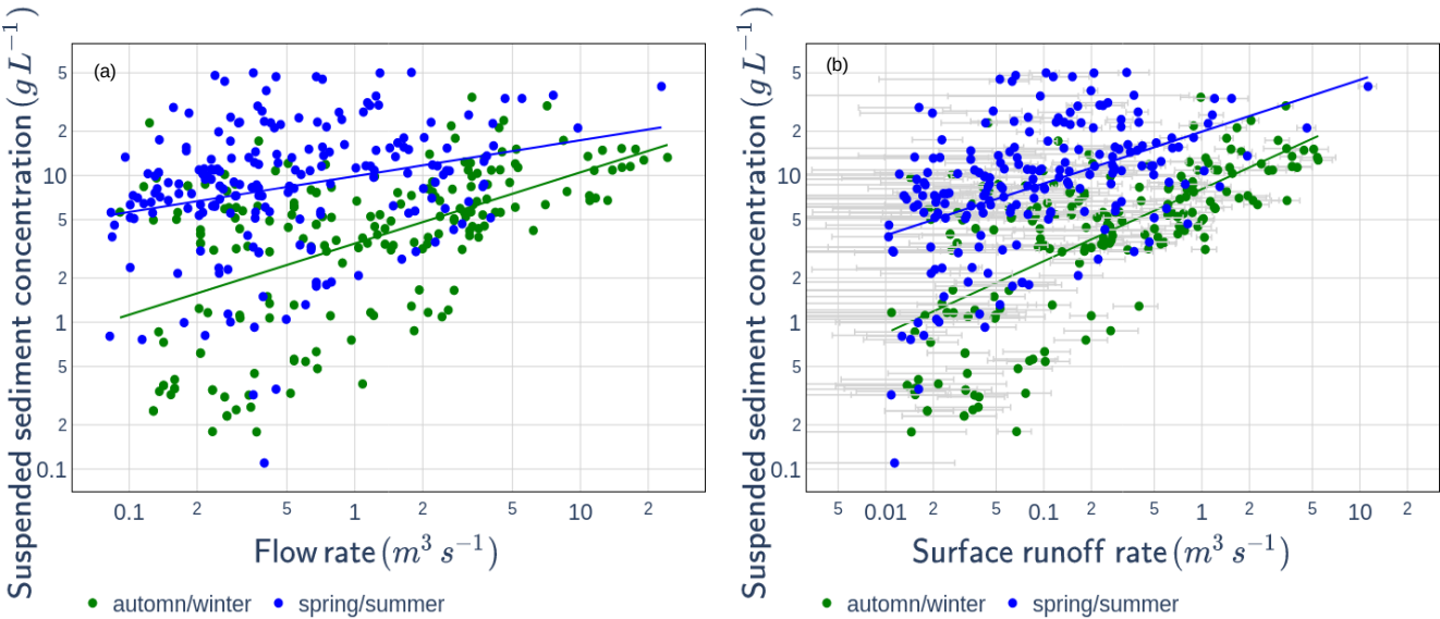
Figure 6. Relationship between suspended sediment concentration and (a) total flow rate or (b) surface runoff flow rate, distinguished by season: October-April (green) and May-September (blue). Light-grey uncertainty bars represent uncertainties associated with the End Member Modeling Mixing Analysis results.
