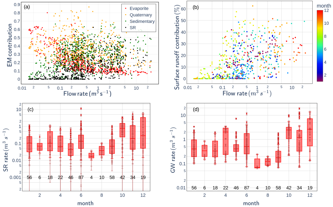
Figure 4. (a) Contributions of the different end-members (EM) as a function of flow rate at the Galabre outlet; (b) surface runoff contribution to total flow at the outlet as a function of flow rate, with points colored by month; (c) and (d) surface runoff (SR) flow rate and groundwater (GW) flow rate, respectively, at the Galabre outlet during rainfall-runoff events, shown by month. The number of samples per month is indicated above the x-axis.
