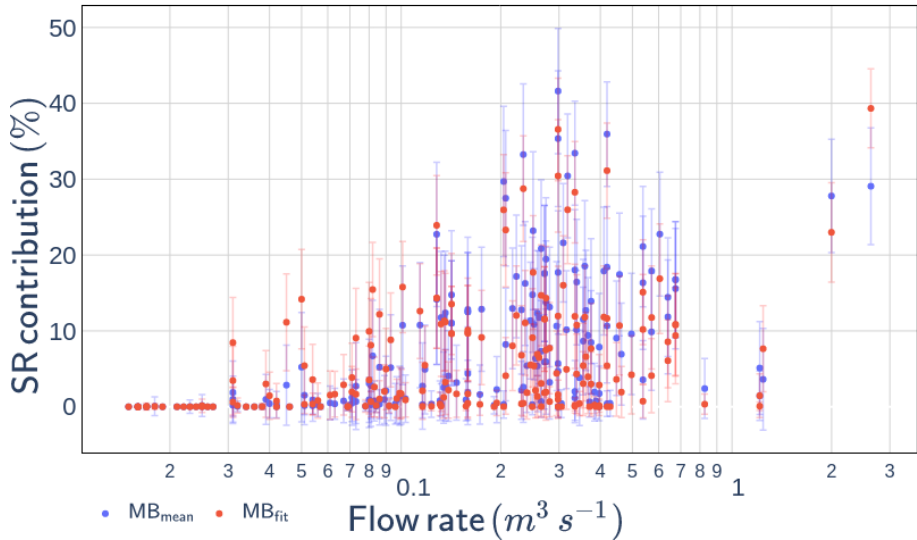
Figure A4. Surface runoff (SR) contribution for samples collected outside of rainfall-runoff events, calculated with the MB_{mean} and MB_{fit} End Member Modeling-Mixing Analysis methods.
