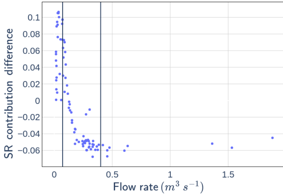
Figure A6. Event-averaged difference between the surface runoff (SR) contributions estimated by the MB_{fit} and MB_{mean} models, shown as a function of the initial flow rate of each event. The vertical lines indicate the flow-rate interval used to compute the adjustment between tracer concentration and flow rate (see Sect. 2.2)
