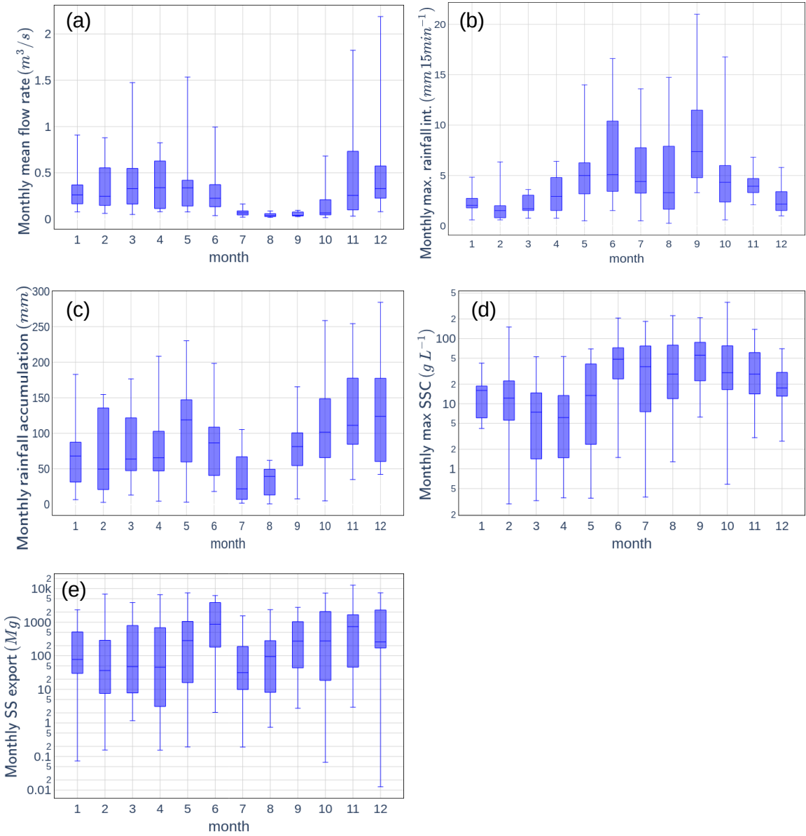
Figure 2. Seasonal variations of (a) monthly mean flow rate, (b) monthly maximum rainfall intensity, (c) monthly rainfall accumulation, (d) monthly maximum suspended sediment concentration (SSC) and (e) monthly suspended export (SS) export in the Galabre catchment, computed with data taken at the Galabre outlet and the meteorological station from 2007 to 2025.
