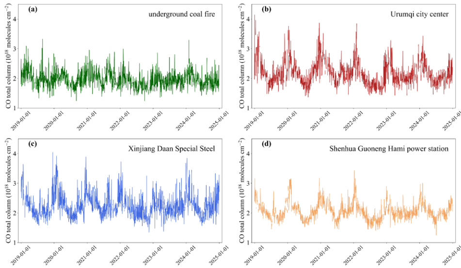
608 609 Figure 4. Time series of TROPOMI CO total columns in the 0.05^\circ \times 0.05^\circ grid cells containing (a) the Wugonggou underground 610 coal-fire site, (b) the center of Urumqi, (c) Xinjiang Daan Special Steel, and (d) Shenhua Guoneng Hami Power Station during 611 2019–2024.
