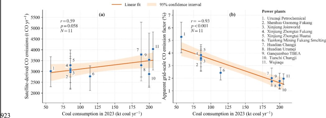
Figure 9. Relationship between satellite-derived CO emissions and coal consumption at selected coal-fired power plants. (a) Comparison between annual coal consumption and MFlEF-derived CO emissions for individual power-plant grid cells. (b) Relationship between coal consumption and the grid-scale CO emission-to-coal-consumption ratio. Circles and vertical error bars represent the means and 25th–75th percentile ranges, respectively.
