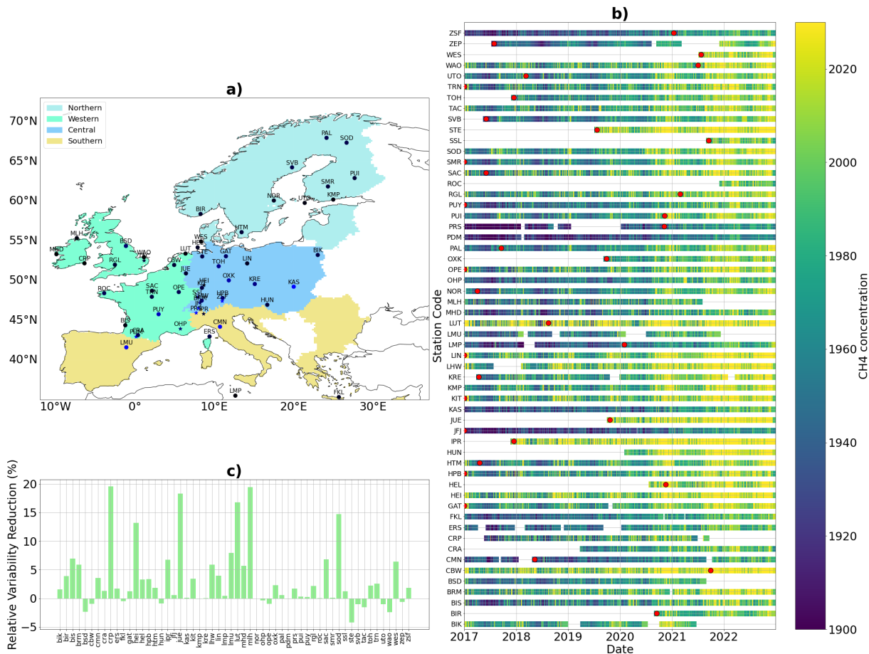
Figure 1. a) Distribution of the CH 4 observational network used in the inversion. Black dots indicate low-altitude stations (<1000 m a.s.l.), while blue dots represent high-altitude stations (>1000 m a.s.l.). Stations used in the sensitivity analysis are highlighted with star symbols. The EU27+3 countries are divided into four sub-regions, color-coded as indicated by the color-coded legend. b) Overview of daily mean CH 4 mole fractions from each assimilated station, including the timing of ICOS levelling. Data points after the red dot marker are ICOS-labelled, indicating that measurements have been processed according to ICOS protocols from the indicated date onward. White gaps indicate periods with missing data. c) Relative variability reduction (%) for each station, defined as (1 - \frac{\sigma_{\text{window}}}{\sigma_{\text{full}}}) \cdot 100 , where \sigma_{\text{full}} is the standard deviation over the full period (2017–2022), and \sigma_{\text{window}} is computed over 14:00–16:00 for low-altitude stations and 02:00–04:00 for high-altitude stations.
