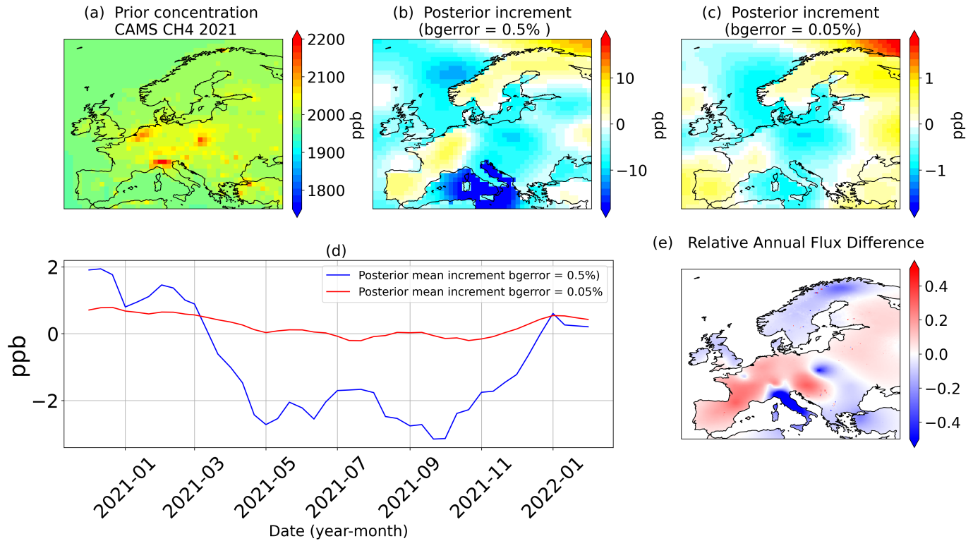
Figure 11. Impact of background error assumptions on optimized methane mole fractions and fluxes for 2021. Top row: (a) Prior mole fractions from CAMS and posterior increments with background error assumptions of (b) 0.5 % and (c) 0.05 %. Bottom row: (d) Time series of posterior mean increments under both settings and (e) relative annual flux difference between inversions with background errors of 0.5 % and 0.05 %. To quantify the impact of background-error assumptions, the relative difference was defined as 1 - \frac{F_{0.5\%}}{F_{0.05\%}} , where F_{0.5\%} and F_{0.05\%} denote the flux computed using a background-error assumption of ( 0.5 % ) and ( 0.05 % ) respectively.
