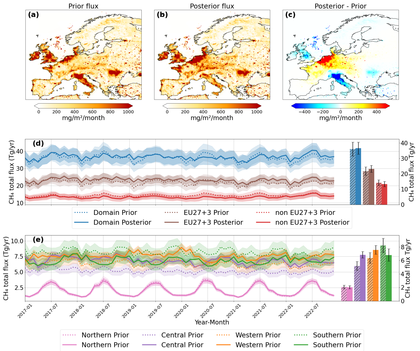
Figure 5. Top row: Mean methane (CH 4 ) fluxes over the EU27+3 domain for the study period (a) prior fluxes, (b) posterior fluxes after inversion, and (c) flux increments (posterior – prior). Middle rows: Monthly CH 4 flux time series averaged over the entire domain, within EU27+3, and outside EU27+3. Bottom row: Monthly CH 4 flux time series for selected EU27+3 subregions (Northern, Central, Southern, and Western), showing prior (dashed lines) and posterior (solid lines) estimates. Bars on the right summarize mean annual prior and posterior fluxes estimates (with a 1- \sigma interannual variability). Shaded areas denote the corresponding prior and posterior uncertainties in the time series, while error bars on the bars represent the associated annual uncertainties.
