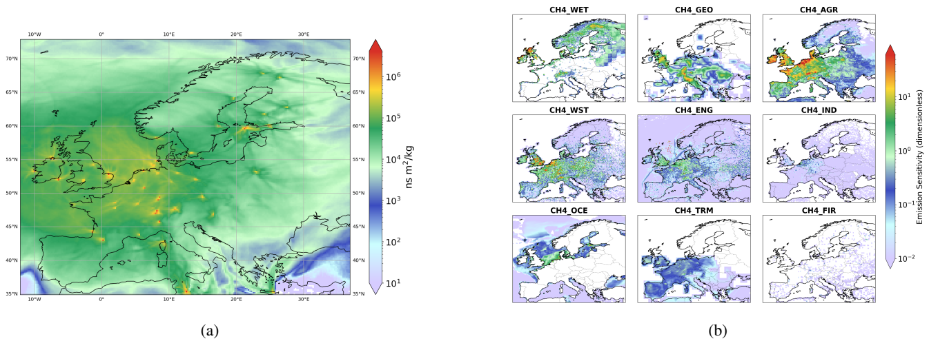
Figure A3. (a) FLEXPART footprint sensitivity to the assimilated observations, shown as the mean sensitivity field for July 2021, illustrating the spatial heterogeneity of observational constraints across Europe. Regions with denser measurement coverage exhibit stronger sensitivities. (b) Emission sensitivity, defined as the product of the footprint sensitivity and the monthly mean prior CH 4 flux for each emission sector, indicating where prior emissions and observational sensitivity jointly contribute to constraining the inversion.
