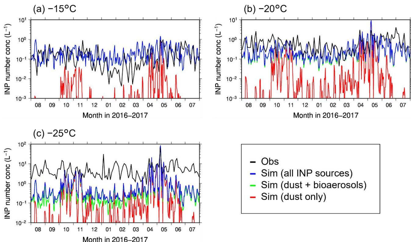
240 Figure 4. INP number concentrations observed at Tokyo Skytree, Japan, throughout the year (three-day mean) at freezing temperatures of (a) -15^{\circ}\text{C} , (b) -20^{\circ}\text{C} , and (c) -25^{\circ}\text{C} (Tobo et al., 2020) (black), and those simulated for the corresponding location and period (daily mean) for dust only (red), dust + bioaerosols (green), and all INP sources (blue).
