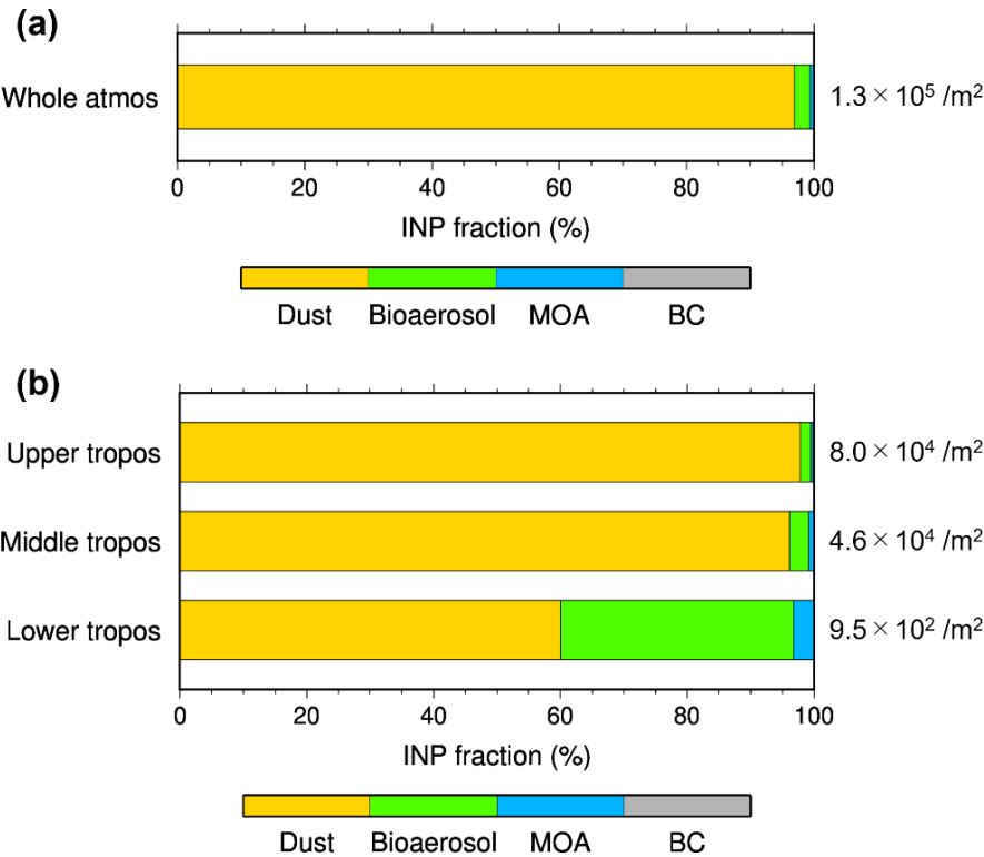
265 Figure 5. Fractions of dust (yellow), bioaerosols (green), MOA (blue), and BC (gray) in the annual and global mean vertically integrated total INP number concentrations (shown on the right) in (a) the whole atmosphere (2–1000 hPa) and (b) the upper (100–400 hPa), middle (400–700 hPa), and lower troposphere (700–1000 hPa).
