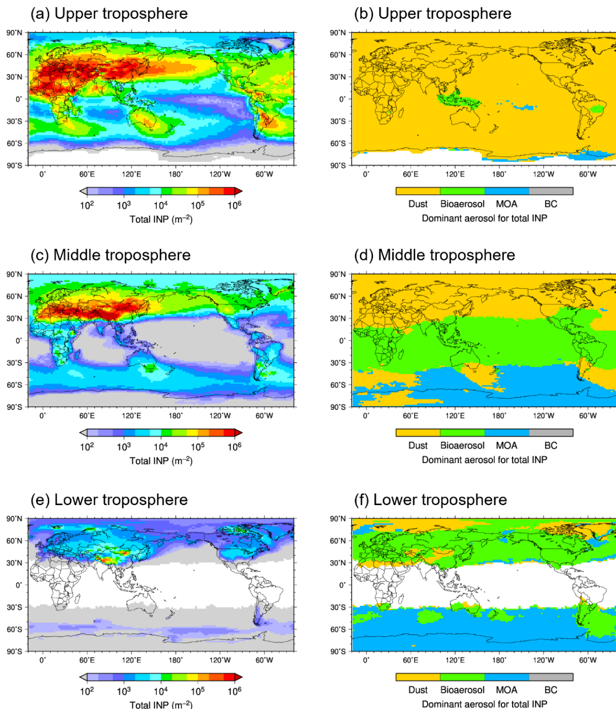
315 Figure 9. (a, c, e) Annual mean vertically integrated total INP number concentrations and (b, d, f) dominant aerosol species contributing the largest fraction of total INPs in (a, b) the upper, (c, d) middle, and (e, f) lower troposphere (same pressure levels as Fig. 5).
