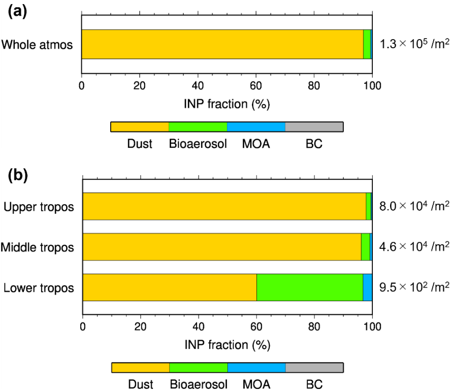
Figure 35. Fractions of dust (orangeyellow), bioaerosols (green), MOA (blue), and BC (gray) in the annual and global mean vertically integrated total INP number concentrations (shown on the right) in (a) the whole atmosphere (2–1000 hPa) and (b) the upper (100–400 hPa), middle (400–700 hPa), and lower troposphere (700–1000 hPa).
