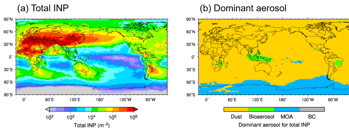
Figure 57. (a) Annual mean vertically integrated INP number concentrations of all aerosol species (total INPs). (b) Dominant aerosol species contributing the largest fraction of the total INP number concentration in each grid.
