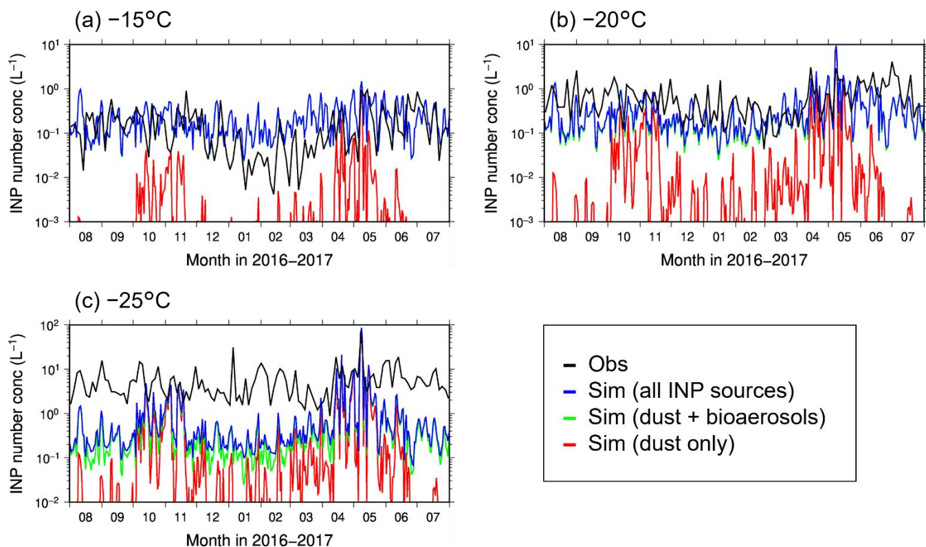
Figure 24. INP number concentrations observed at Tokyo Skytree, Japan, throughout the year (three-day mean) at freezing temperatures of (a) -15^{\circ}\text{C} , (b) -20^{\circ}\text{C} , and (c) -25^{\circ}\text{C} (Tobo et al., 2020) (black), and those simulated for the corresponding location and period (daily mean) for dust only (red), dust + bioaerosols (green), and all INP sources (blue).
