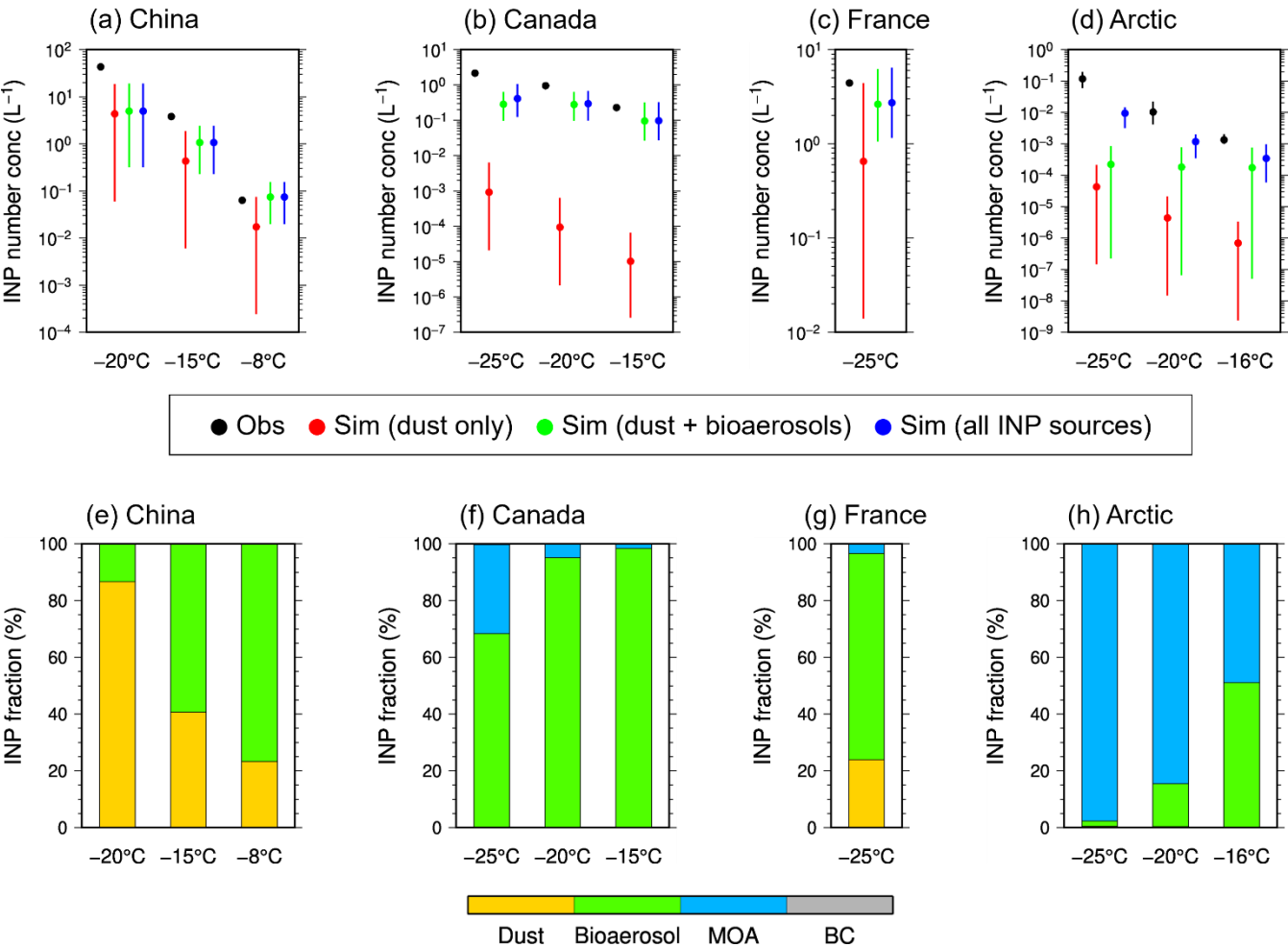
245 Figure 13. (a–d) INP number concentrations observed at (a) Beijing, China (Hu et al., 2023); (b) Vancouver Island, Canada; (c) Saclay, France (Mason et al., 2016); and (d) Svalbard, Arctic (March 2017) (Tobo et al., 2019) at different freezing temperatures (black), and those simulated for the corresponding locations and periods for dust only (red), dust + bioaerosols (green), and all INP sources (blue). Dots and bars represent the averages and ranges (where available) during the observation periods, respectively. (e–h) Fractions of dust (orange), bioaerosols (green), MOA (blue), and BC (gray) in the simulated total INP number concentrations for each location.
