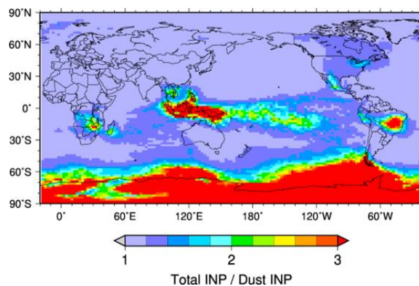
Figure 68. Ratio of the annual mean vertically integrated INP number concentrations of all aerosol species (Fig. 57a) and dust (Fig. 46a).
