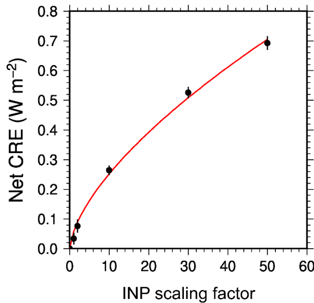
205 Figure 2. Relationship between INP scaling factors and net CREs via dust INPs estimated from the 1-, 2-, 10-, 30-, and 50-fold simulations – 0-fold simulation. Dots and bars indicate the 10-year means and standard deviations of annual mean CREs. The red line represents the fitted power-law function ( y = ax^b ) used to infer the CREs corresponding to the 1-fold – 0-fold simulations.
