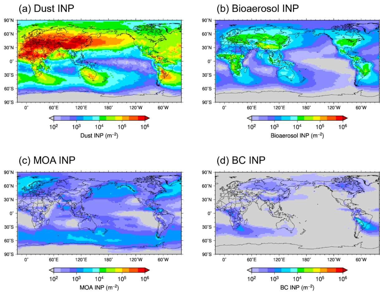
Figure 46. Annual mean vertically integrated INP number concentrations of (a) dust, (b) bioaerosols, (c) MOA, and (d) BC.
