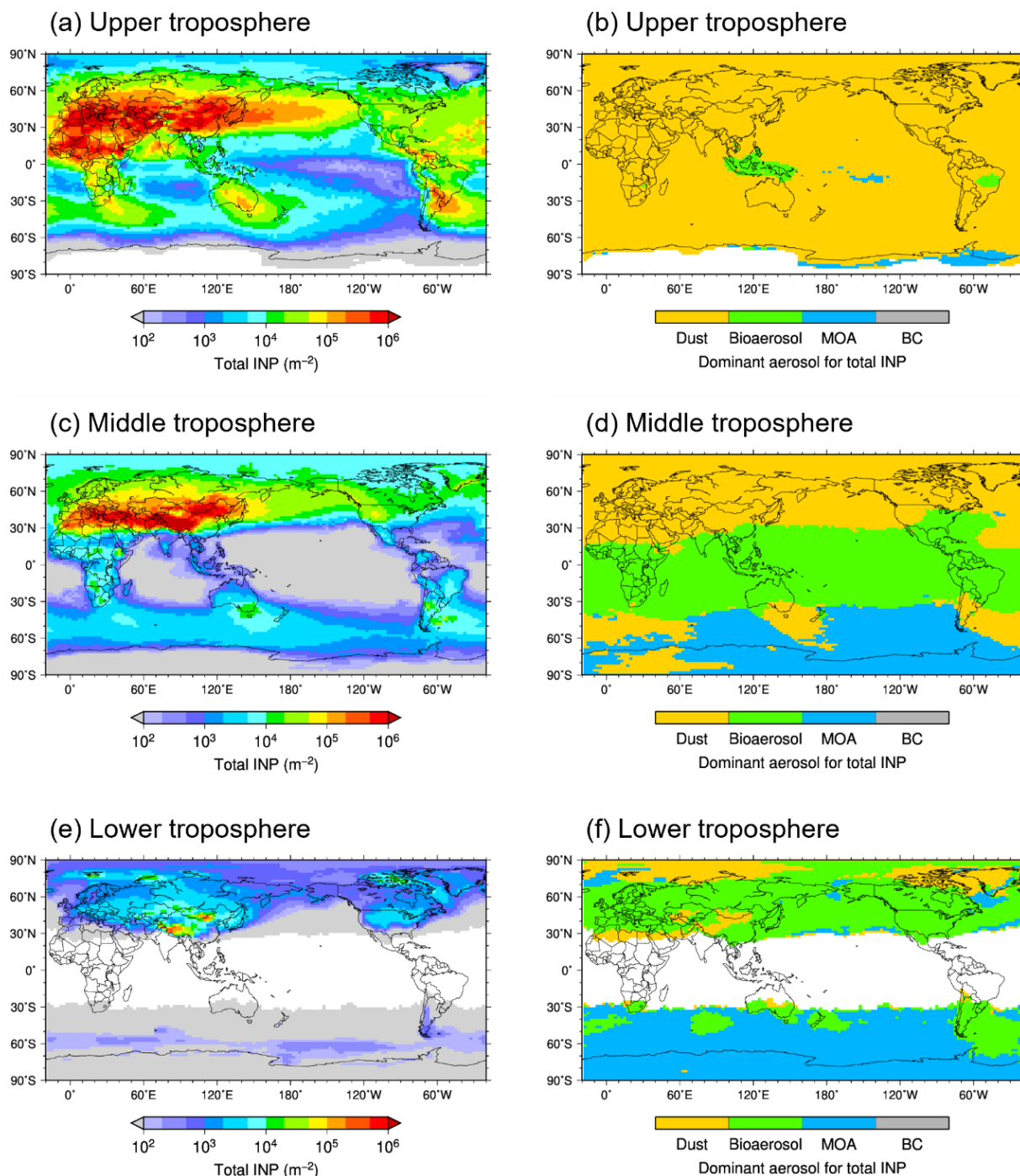
Figure 79. (a, c, e) Annual mean vertically integrated total INP number concentrations and (b, d, f) dominant aerosol species contributing the largest fraction of total INPs in (a, b) the upper, (c, d) middle, and (e, f) lower troposphere (same pressure levels as Fig. 35).
