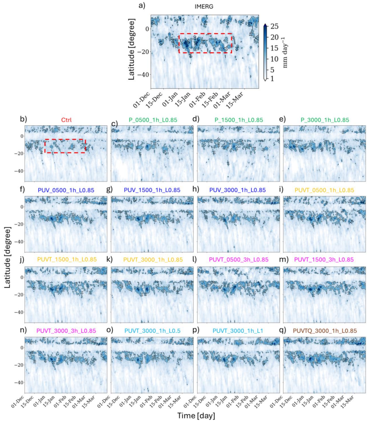
Figure 6 Hovmöller diagram of zonally averaged daily precipitation ( \text{mm day}^{-1} ) from the IMERG dataset for the period 1 December 2010 to 31 March 2011, averaged over 90°E to 170°E. Dash red box indicates the regions of MJO-related peak precipitation.
