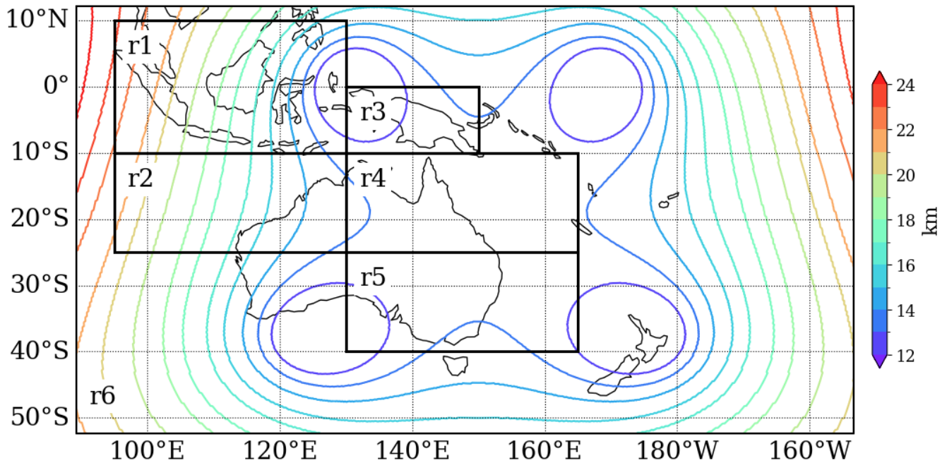
230 Figure 1 CCAM simulation domain with grid resolution ranging from 12 to 25 km, shown in contour colours. The study domain is divided into six subregions, labelled R1 to R6, representing the Maritime Continent, northwest Australia, southwestern pacific, northeast Australia, southeast Australia, and the whole simulated domain (50°S – 10°N, 90°E – 150°W), respectively.
