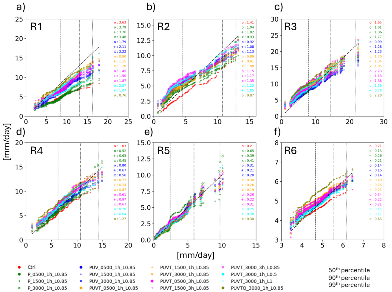
445 Figure 9 Quantile–quantile plots of regionally averaged daily precipitation (mm day -1 ) against IMERG for six subregions. Coloured symbols denote different CCAM simulations (see legend). The dashed 1:1 line represents perfect agreement with observations. The numbers indicate the area formed by the 1:1 and model line. Numbers on the top right of each panel indicate the area between IMERG and CCAM in which the larger the number, the larger the difference between the two.
