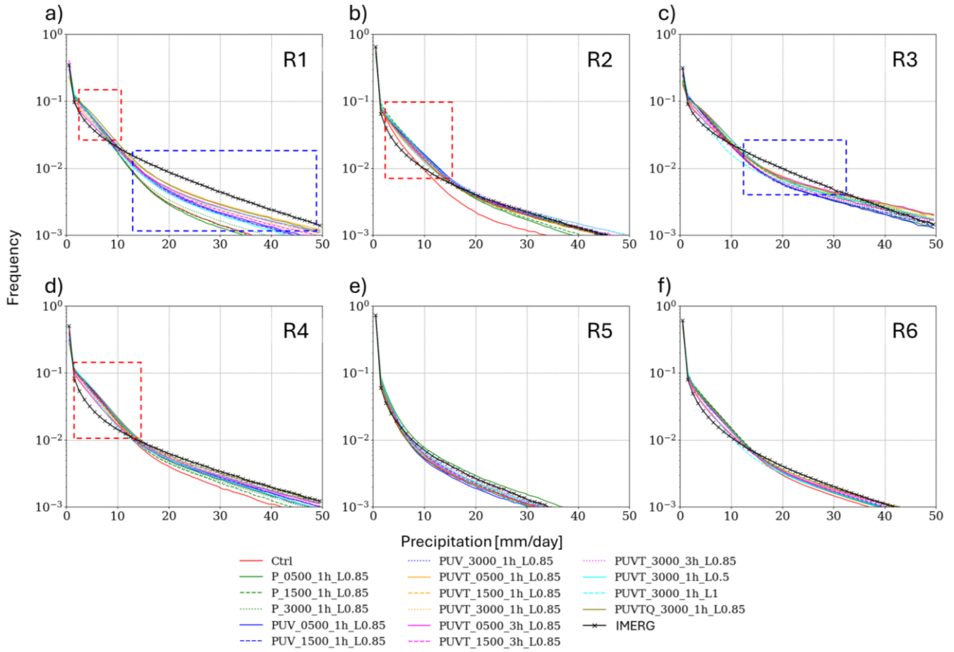
Figure 4 Frequency of daily precipitation intensity for IMERG and 16 CCAM simulations averaged over each region from December 2010 to March 2011. The dashed red and blue boxes indicate regions where the model respectively overestimates and underestimates precipitation compared to IMERG
