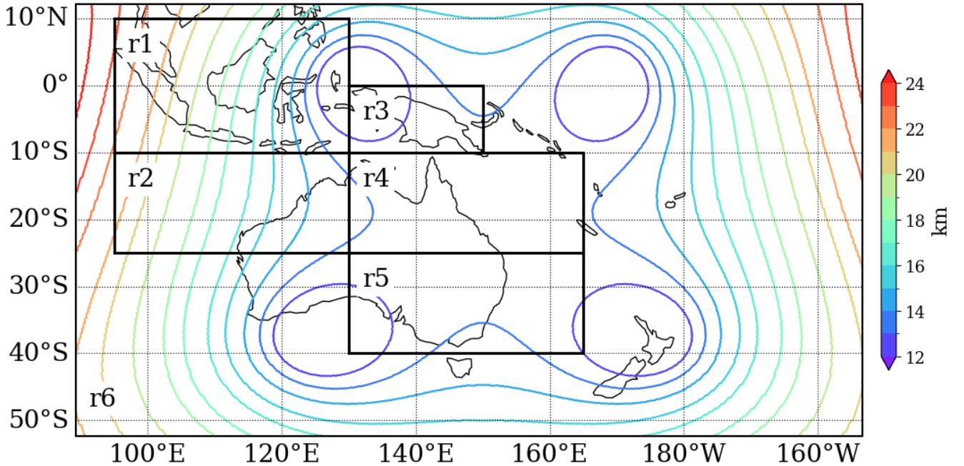
Figure 1 CCAM simulation domain with grid resolution ranging from 12 to 25 km, shown in contour colours. The study domain is divided into six subregions, labelled R1 to R6, representing the Maritime Continent, northwest Australia,
