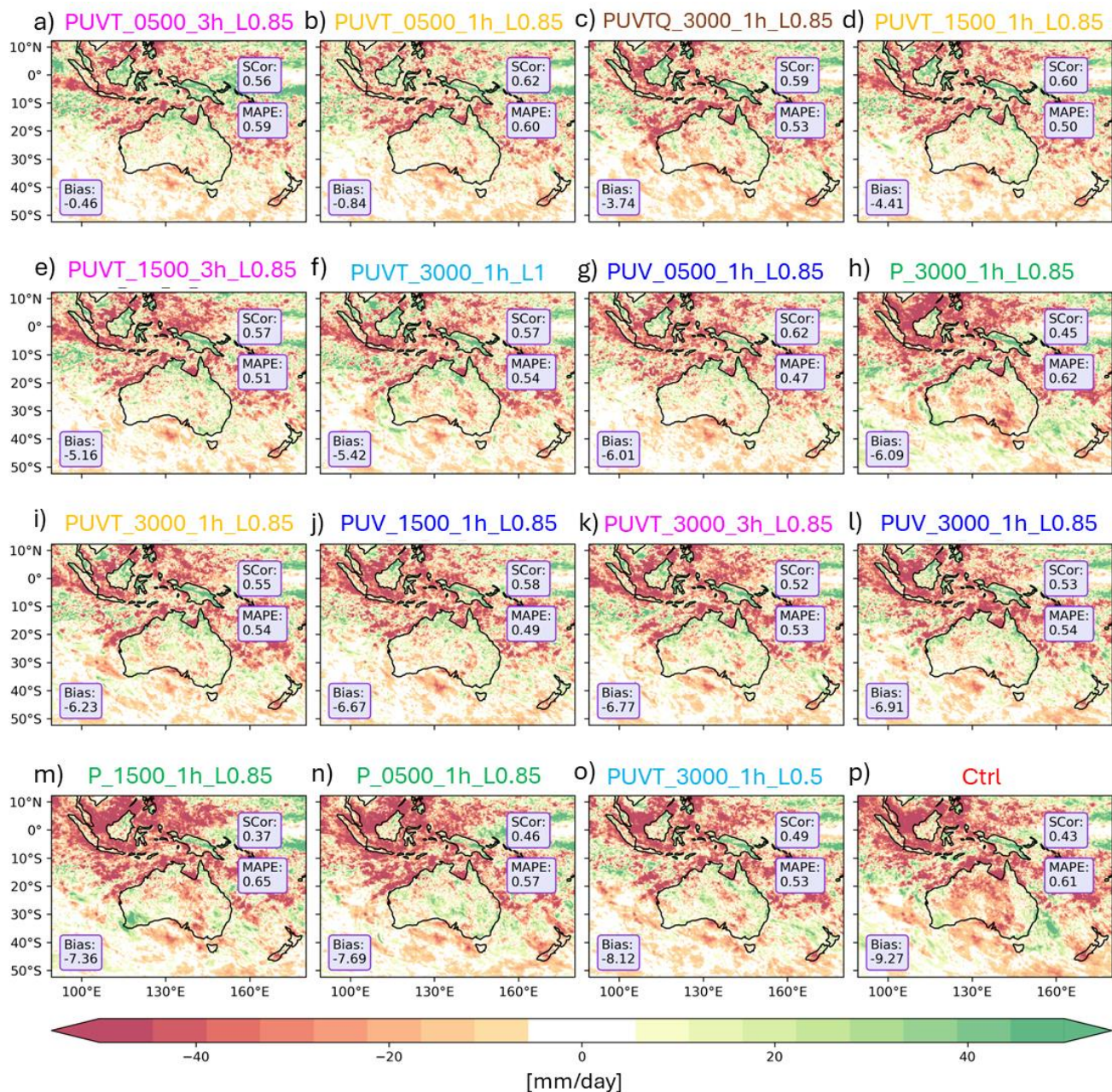
470 Figure 10. Bias of monthly maximum 1-day precipitation (Rx1day; mm day -1 ) from December 2010 to March 2011 475 relative to IMERG. Each panel shows one CCAM spectral nudging simulation (see labels), with shading indicating spatial bias across the CORDEX–Australasia domain. Statistics included in each panel are the spatial correlation (SCor), mean absolute percentage error (MAPE), and domain-averaged bias. Panels (a)–(p) are ordered from the wettest to driest model configurations.
