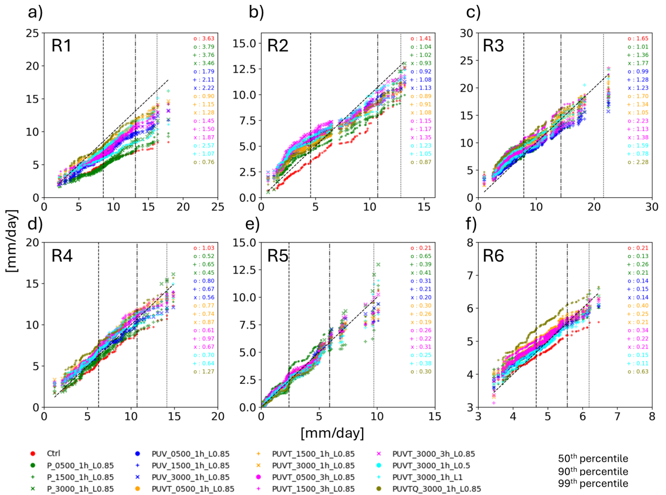
Figure 9 Quantile–quantile plots of regionally averaged daily precipitation ( \text{mm day}^{-1} ) against IMERG for six subregions. Coloured symbols denote different CCAM simulations (see legend). The dashed 1:1 line represents perfect agreement with observations. The numbers indicate the area formed by the 1:1 and model line. Numbers on the top right of each panel indicate the area between IMERG and CCAM in which the larger the number, the larger the difference between the two.
