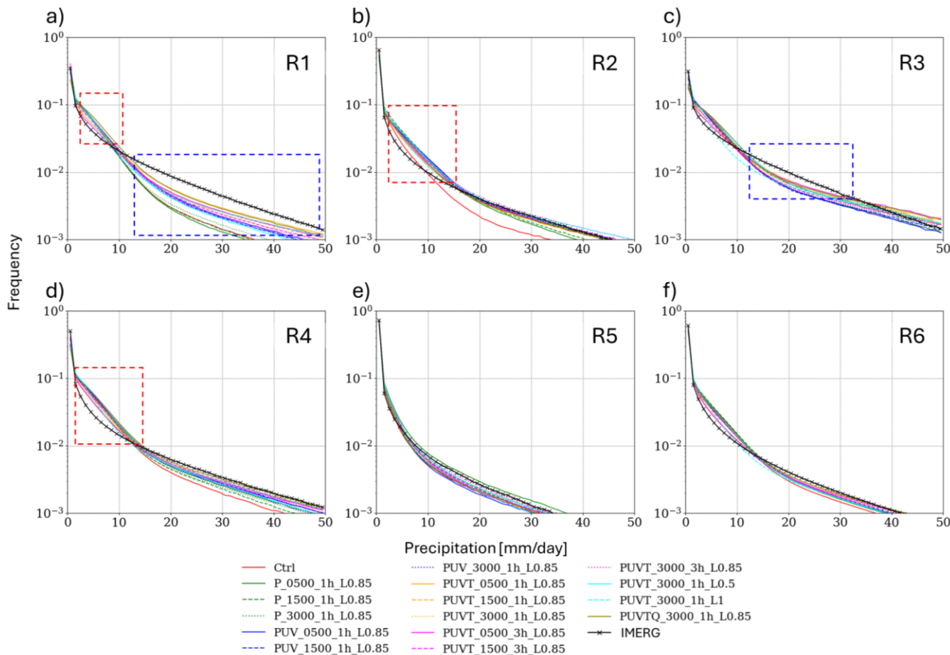
310 Figure 4 Frequency of daily precipitation intensity for IMERG and 16 CCAM simulations averaged over each region from December 2010 to March 2011. The dashed red and blue boxes indicate regions where the model respectively overestimates and underestimates precipitation compared to IMERG
