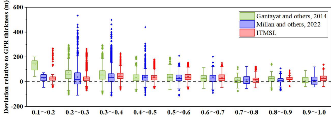
Figure 10: Comparative analysis of ice thickness estimation deviations for different ratios of basal sliding to surface velocity.
