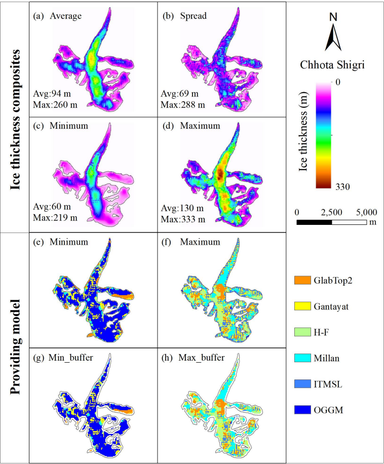
520 Figure 12: Comparison of simulated ice thickness among models. The first four panels present composite results from the models: (a) average, (b) spread, (c) minimal, and (d) maximal ice thickness distribution. The models corresponding to the minimum and maximum ice thickness at each pixel are shown in (e) and (f), respectively; Models corresponding to the minimum (g) and maximum (h) ice thickness at each pixel after excluding the 3×30 m buffer zone.
