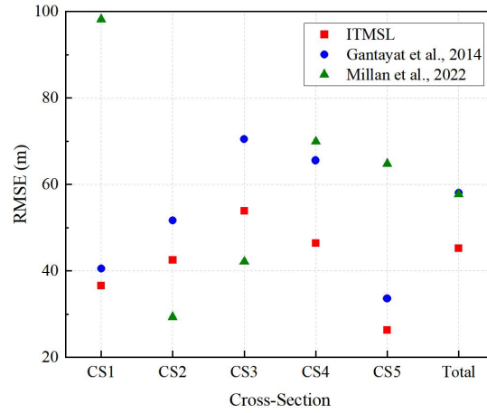
Figure 5: RMSE of CTSG glacier 5 cross-sections.
