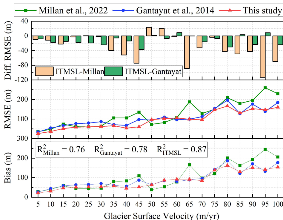
435 Figure 8: Comparison of ice-thickness inversion bias, root-mean-square error (RMSE), and their differences among ITMSL, Gantayat, and Millan models across surface velocity intervals.
