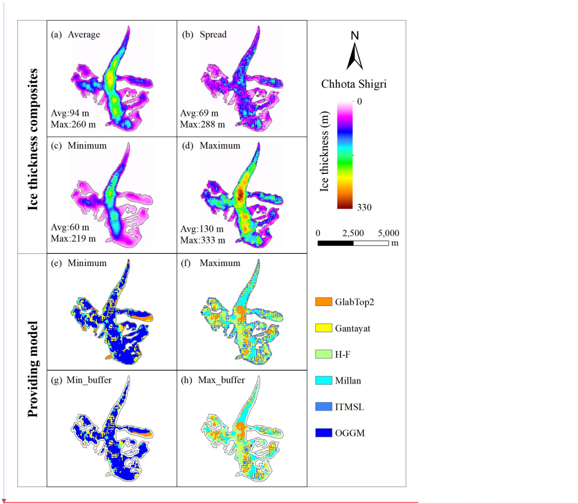
520 Figure 12: Comparison of simulated ice thickness among models. The first four panels present composite results from the models: (a) average, (b) spread, (c) minimal, and (d) maximal ice thickness distribution. The models corresponding to the minimum and maximum ice thickness at each pixel are shown in (e) and (f), respectively; Models corresponding to the minimum (g) and maximum (h) ice thickness at each pixel after excluding the 3×30 m buffer zone.
