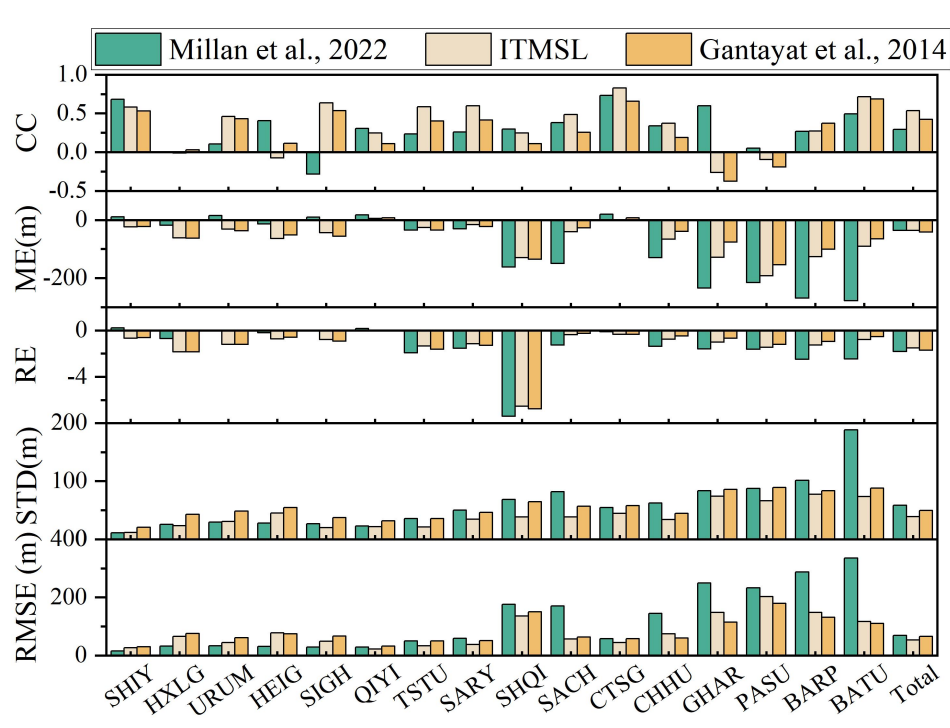
Figure 7: Comparison of ice-thickness inversion accuracy among three SIA-based models (Millan, Gantayat, ITMSL), referenced against GPR measurements. Metrics: correlation coefficient (CC), mean error (ME),
