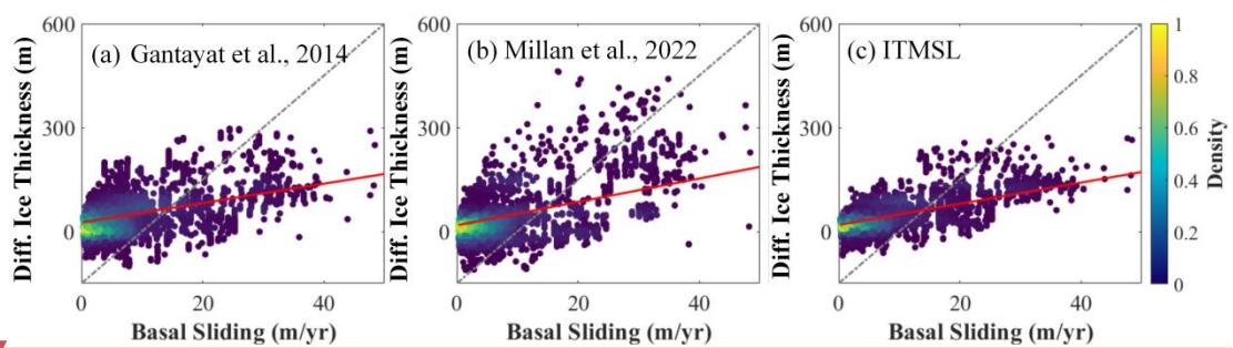
Figure 11: Deviations of ice thickness estimates from three laminar flow models at different basal sliding. (a) Gantayat; (b) Millan; (c) ITMSL.
