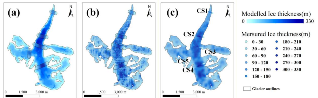
Figure 4: CTSG glacier thickness estimated by the three models. (a) Millan et al., 2022, (b) Gantayat et al., 2014, (c) ITMSL.
