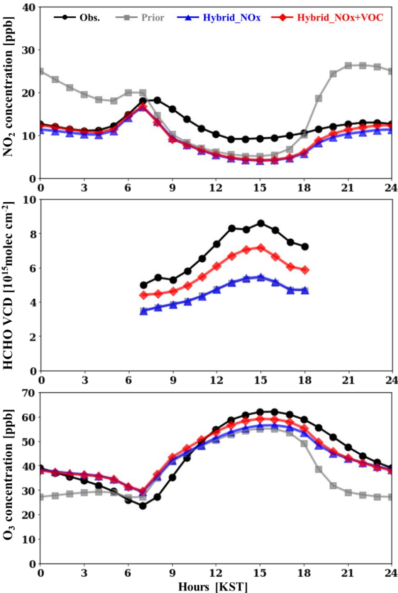
430 Figure 7: Diurnal variations of NO 2 (top) and O 3 (bottom) concentrations for each experiment (Prior: gray, Hybrid_NOx: blue, Hybrid_NOx+VOC: red, Observations: black) in comparison to the observations. The data are averaged over all observation station locations in South Korea during the study period.
