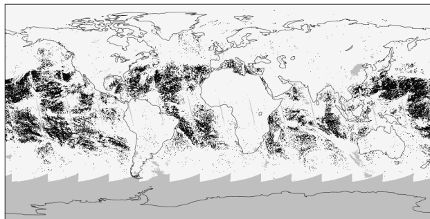
Figure 6. Map of ground pixels with Q_{\text{RMS}}^{430} \geq 2.0 in black and the other pixels in white from all orbits of 5 June 2019; a colour scale version of the map is given in Fig. C1 for clear-sky and cloudy pixels separately. (Maps like this one are made with Panoply.)
