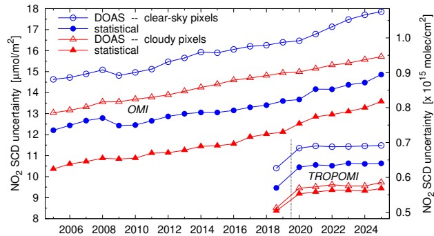
Figure 2. Yearly average DOAS (open symbols) and statistical (filled symbols) uncertainties for clear-sky (blue symbols) and cloudy (red symbols) pixels for-of the OMI (top four curves) and TROPOMI (bottom-right four curves) NO 2 slant column retrieval over the Pacific Ocean . In view of the TROPOMI pixel size reduction on 6 Aug. 2019 (indicated by the vertical dotted line), the first year cannot be a calendar year; instead the period 1 Aug. 2018 through 31 July 2019 is used.
