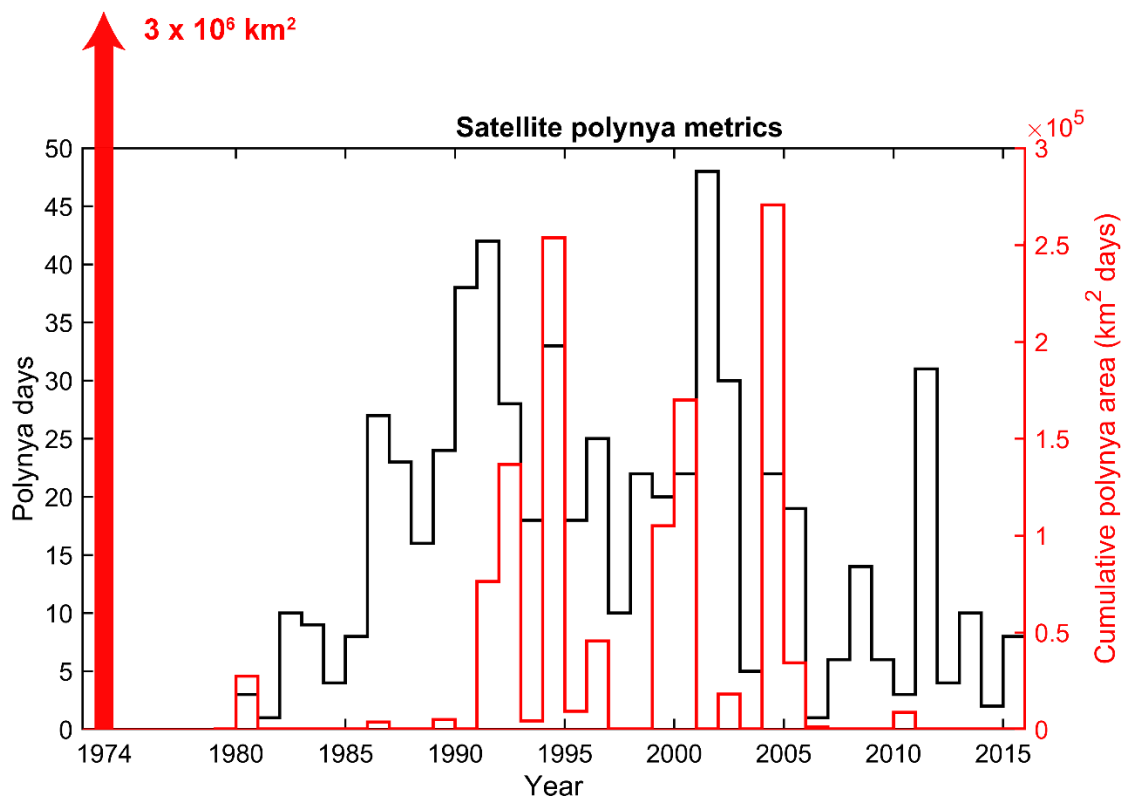
Figure 4 | Satellite polynya metrics. Two different annual metrics of satellite-derived polynya
