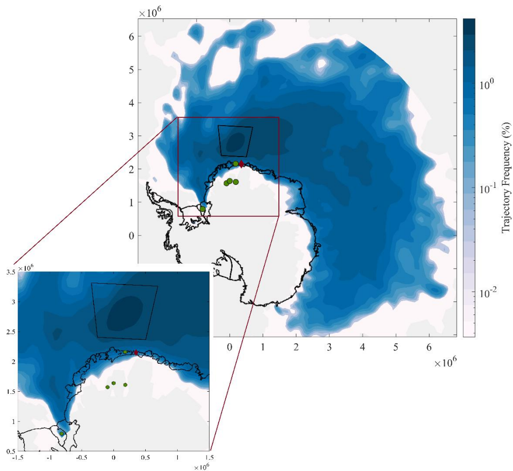
638 Figure 5 | Airmass transport pathways originating from MRP: EndpointTrajectory 639 frequency of forward trajectories originating over the polynya-prone region (Heuzé et al., 640 2021) of the Weddell Sea, showing the prevalent transport pathway during the winter to early 641 spring months for the period 1948 – 2016. A significant proportion of the trajectories end over 642 our ice core site (red diamond). Location of ice cores used by Goosse et al., (2021) are shown 643 with green circles. The gray region shows area with no trajectory endpoints Location of ice 644 cores used by Goosse et al. (2021) are shown with green circles. The black trapezium shows 645 the polynya prone regions. The gray region shows area with no trajectories.
