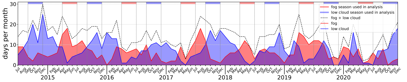
Figure 2. Time series of monthly counts of fog (red) and low-cloud (blue) events and their sum (dashed line) between 4 and 6 UTC at CM, according to combined SEVIRI-based low-cloud data and in situ fog precipitation. Bars at the top and dotted vertical lines indicate the months of peak seasons at CM of fog (red, April-May-June) and low clouds (blue, September-October-November).
