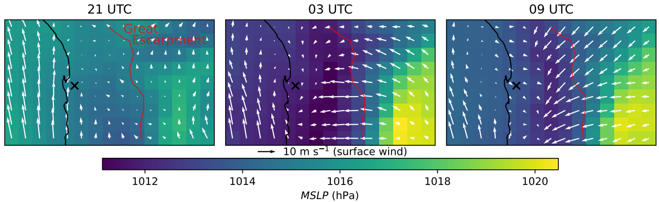
Figure A2. Mean sea level pressure ( MSLP ) during the fog night 22./23.09.2017. Quivers denote the surface wind at 10 m. The red line provides an approximate indication of the Great Escarpment (1000 m elevation contour).
