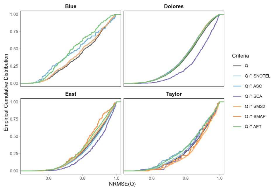
Figure 5. The cumulative distribution of streamflow performance, NRMSE(Q), for differentis influenced by intersections withbetween streamflow and alternative observations. The black line represents the distribution when filtering with Q only. A distribution that is closer to zero (left) is considered informative in the case of NRMSE.
