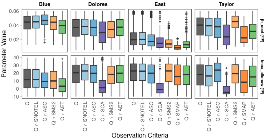
385 Figure 6. The inter-quartile ranges of behavioral parameter values fluctuate across observation intersection criteria. For catchments that have more than one stream gauge, the behavioral intersection of both stream gauges is used. For SNOTEL , SMS2, and ASO, the best performing site/acquisition is shown. Datasets that returned an insufficient number of behavioral parameter sets are excluded.
