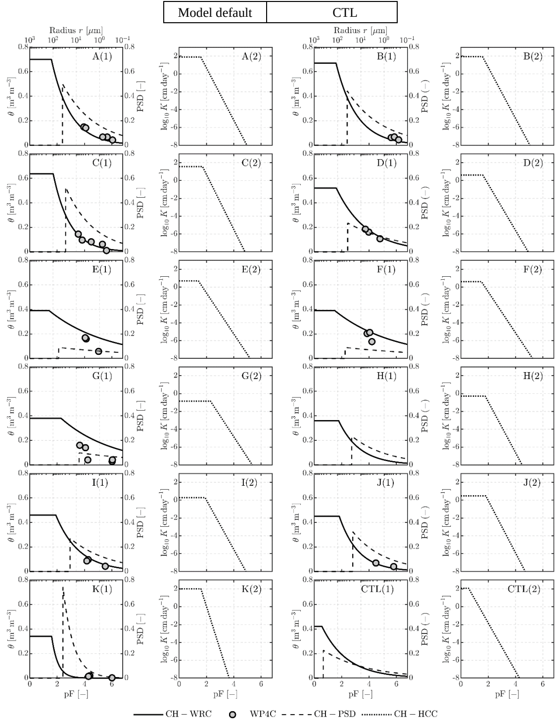
Fig. 7. Vertical profiles of measured and modeled WRC, PSD, and HCC for different soil depths (solid line: CH–WRC; dashed line: CH–PSD; dotted line: CH–HCC; gray circles: WP4C measurements).
