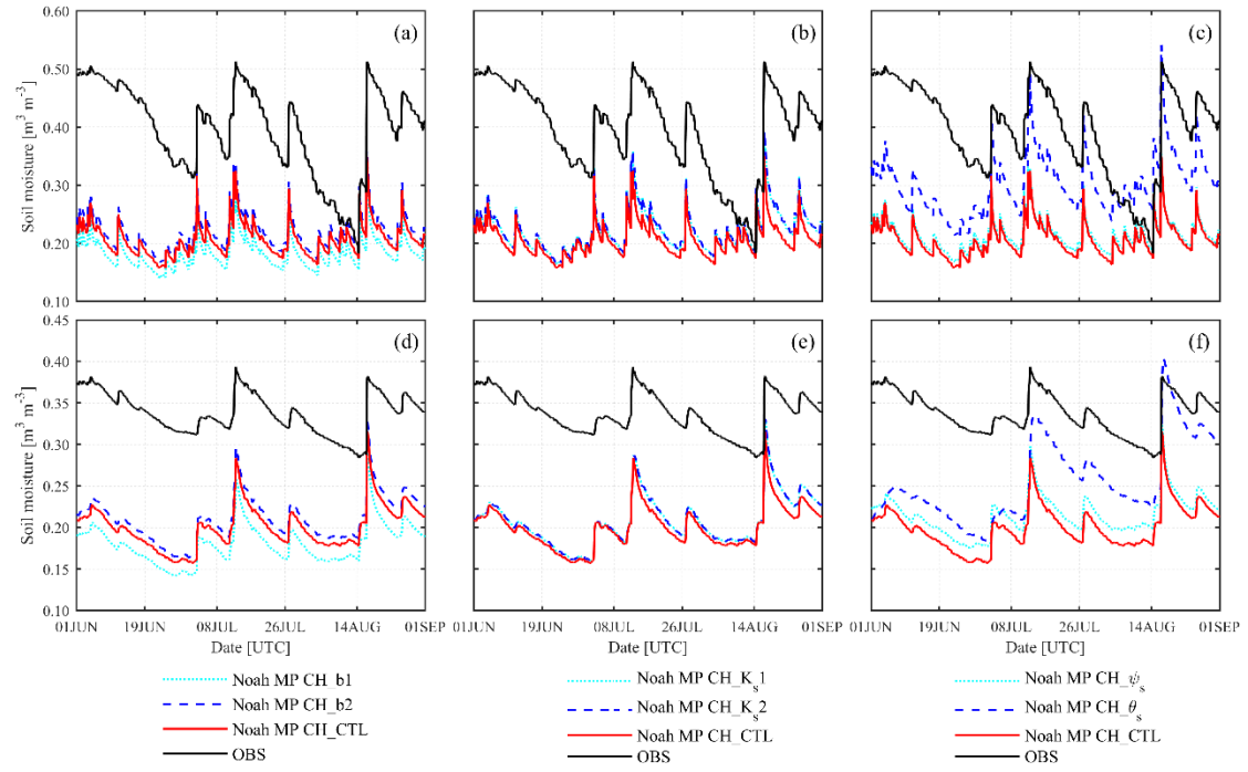
Fig. 14. Simulated diurnal soil moisture at two depths over June–August, 2023.
