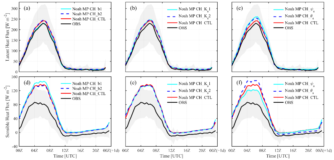
Fig. 11. Modeled diurnal variations of LHF and SHF under different soil hydraulic parameter scenarios, averaged for June–August 2023. (Panels (a,d) show sensitivity experiments for the b parameter; panels (b,e) for K_s ; and panels (c,f) for \psi_s and \theta_s . All times are in Coordinated Universal Time (UTC, Z). Local time = UTC + 8 h).
