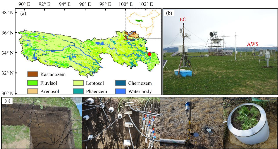
Fig. 1. Soil classification in the Sanjiangyuan region and overview of the observation site. (a) Spatial distribution of main soil types in the Sanjiangyuan region; (b) summer view of the station and main observation systems, including the eddy covariance (EC) and automatic weather station (AWS); (c) soil profile and monitoring instruments at the observation site, including soil temperature and moisture profile sensors, infrared surface temperature sensors, and a lysimeter.
