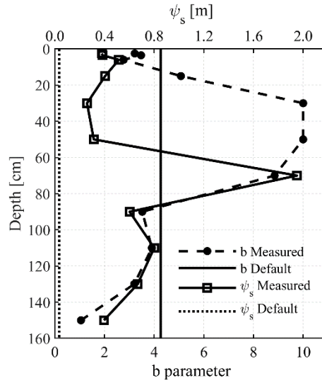
Fig. 5. Comparison of the \psi_s and the index b obtained from evaporation experiments with the Noah-MP default parameters.
