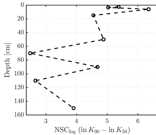
Fig. 10. Vertical profiles of near saturated connectivity (NSC-log).
