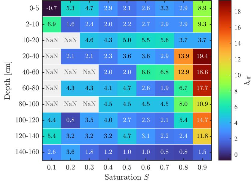
Fig. 8. Two-dimensional distribution of effective exponent b_{eff}(S) across soil depths.
