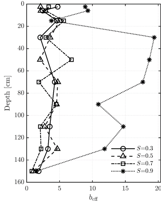
Fig. 9. Vertical profiles of b_{eff} under typical saturation levels ( S = 0.3, 0.5, 0.7, 0.9 ).
