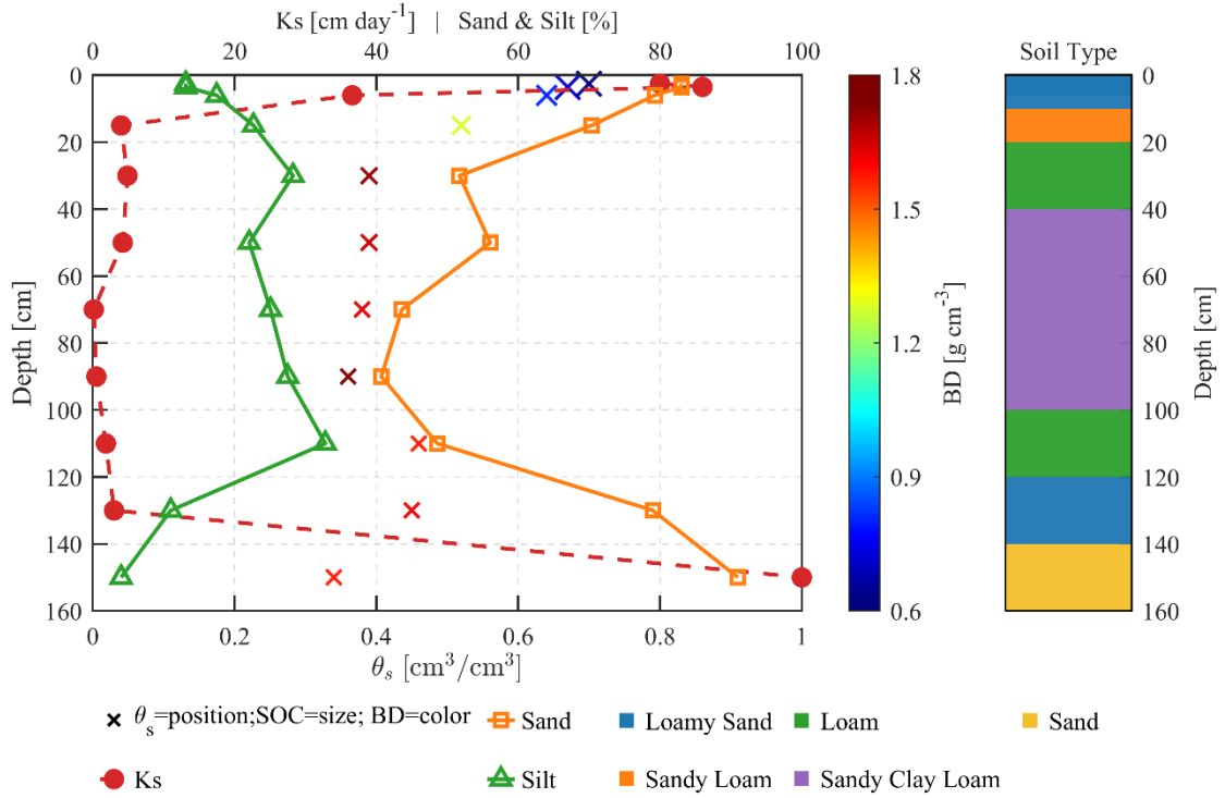
Fig. 4. Vertical distribution of hydraulic properties in the wetland soil (Crosses indicate sampling positions of \theta_s ; cross size represents SOC content, and color corresponds to BD. Red circles denote K_s ; orange squares and green triangles represent sand and silt contents, respectively. The colored blocks on the right show the distribution of soil types at different depths (Loamy Sand, Loam, Sand, Sandy Loam, Sandy Clay Loam)).
