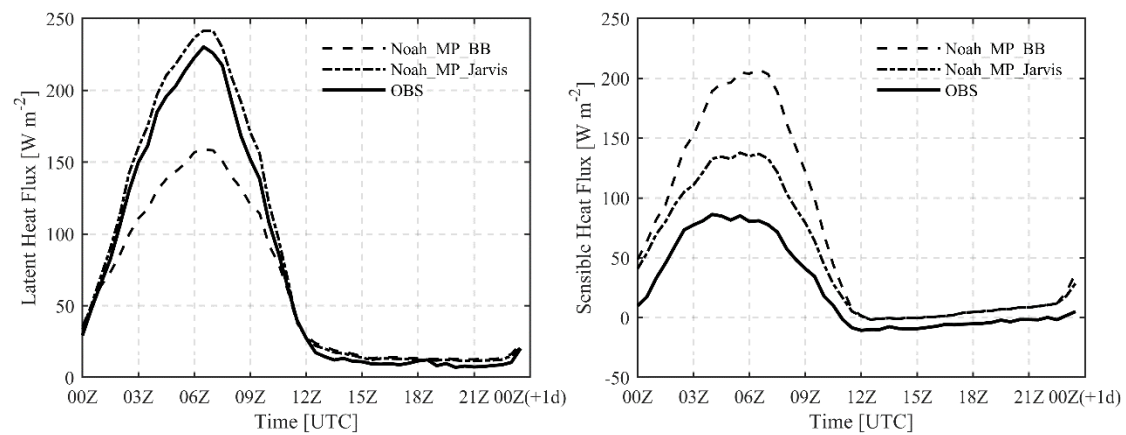
Fig. 13. Impact of the Jarvis and Ball Berry schemes on the simulated mean diurnal cycle.
