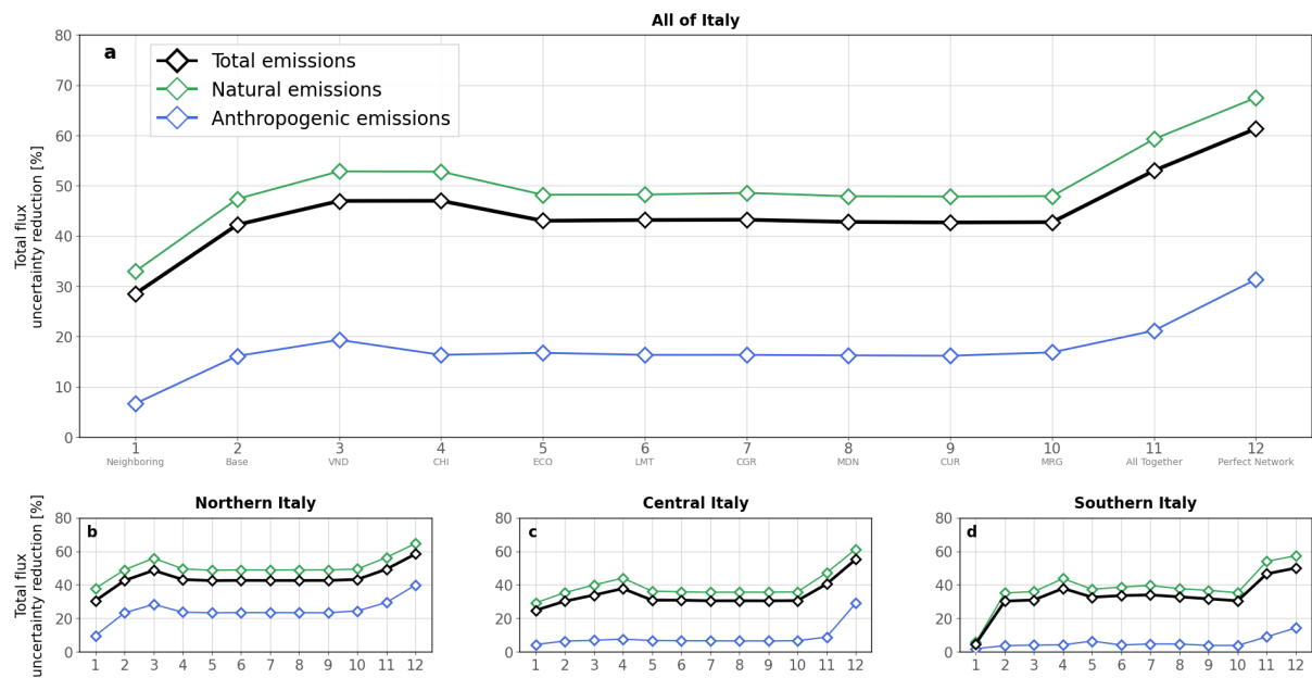
Figure C2. TUR for each network scenario over all of Italy, Northern Italy, Central Italy, and Southern Italy. Black, green, and blue lines represent TUR for total, natural, and anthropogenic emissions, respectively.
