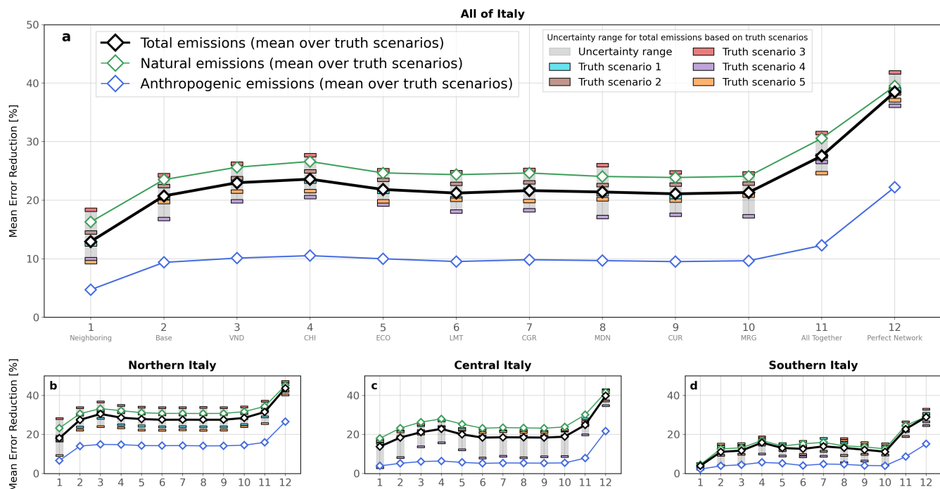
Figure 5. MER for each network scenario over all of Italy, Northern Italy, Central Italy, and Southern Italy. Black, green, and blue lines represent MER for total, natural, and anthropogenic emissions, respectively, averaged across all truth scenarios. The shaded area indicates the uncertainty range of MER for total emissions arising from different truth scenarios, while the colored rectangles show MER calculated for the individual truth scenarios.
