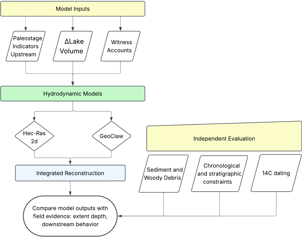
90 Figure 2. Conceptual workflow for reconstruction of the 1989 Laguna del Cerro Largo GLOF.
