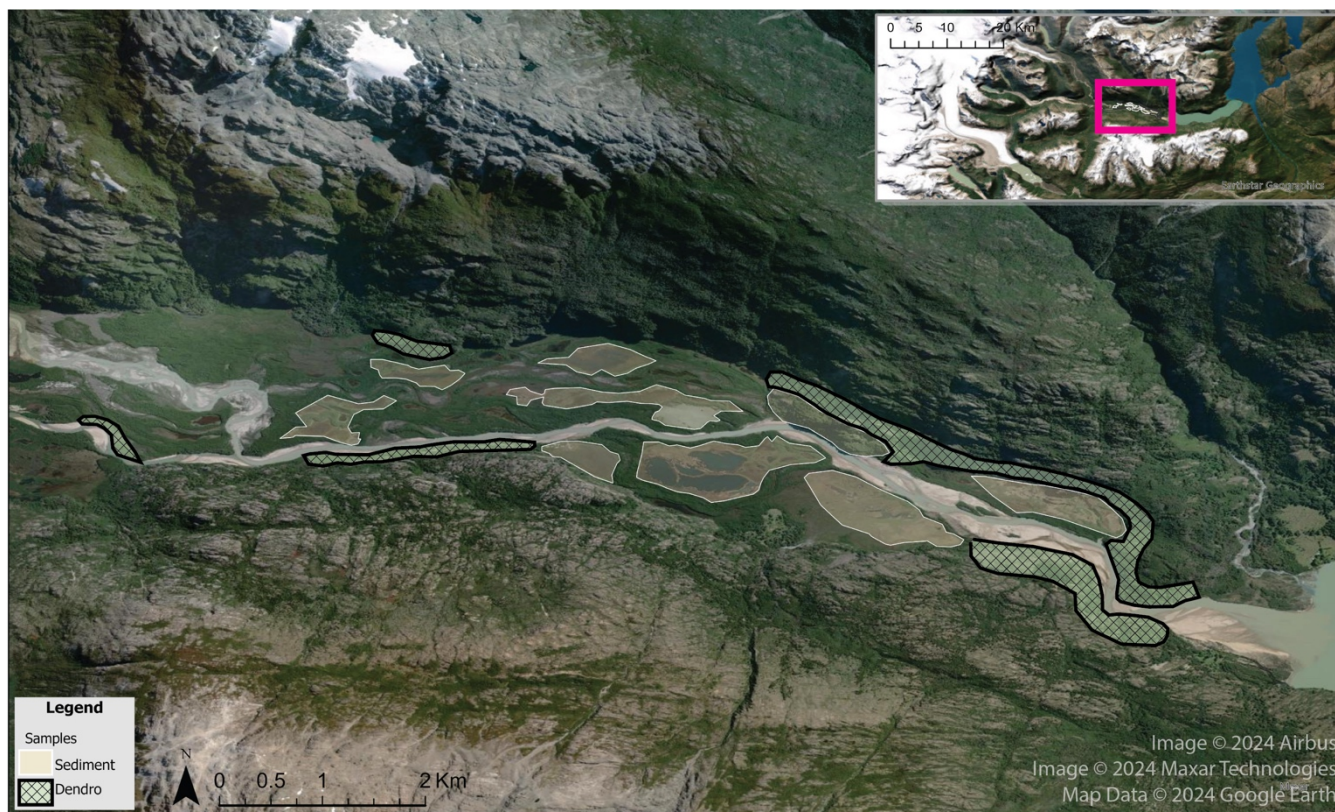
180 Figure 3. Map of identified potential sampling sites for both sediment (tan) and dendrogeomorphic (hatched light green) of the lower Valle Soler. Maps data: © Google Earth 2024; images: © Airbus, Maxar Technologies.
