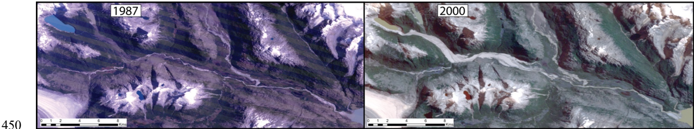
Figure 12. Historic imagery Landsat 5 (TM) of Valle Soler. Valle Soler deposits are clearly visible in the post-GLOF (2000) image, and similar impacts are visible emanating from Laguna Turbio.
