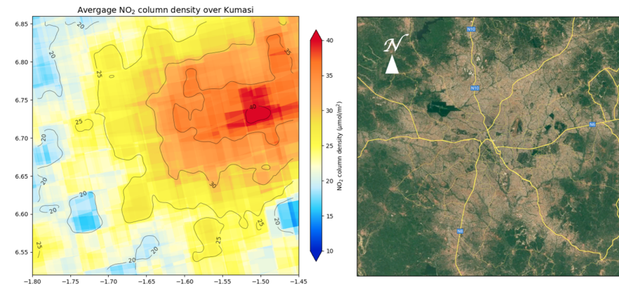
375 Figure 9: Averaged satellite measurement of tropospheric NO 2 columns density over Kumasi from 7 March to 3 April 2025. The map represents an area of 38 x 38 km 2 . Contour lines are shown for the measurement field smoothed with a Gaussian kernel of \sigma=400 m. (Basemap taken from Google Maps ©2025 Google.)
