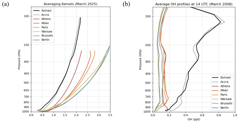
440 Figure 11: (a) Tropospheric averaging kernels from TROPOMI over selected cities, averaged over March 2025. (b) Average OH profiles around satellite overpass time from TM5-MP simulations at 1°×1° resolution for March 2008.
