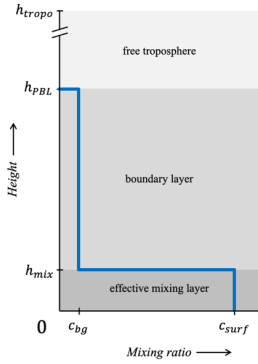
480 Figure 12: Vertical distribution model for urban \text{NO}_2 (blue line) with two fit parameters: the background is assumed to be well-mixed throughout the boundary layer with mixing ratio c_{\text{bg}} , while the urban contribution is only well-mixed up to an effective height h_{\text{mix}} . There is no \text{NO}_2 in the free troposphere.
