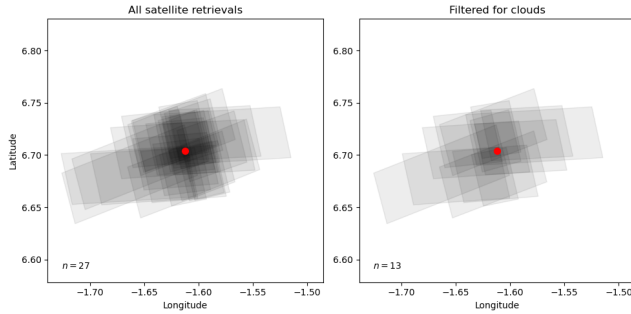
Figure 3: Sampling of location KU-016 (red dot) by TROPOMI during the measurement campaign (7 March – 3 April). The left panel shows all satellite footprints in this period for a 28 \times 28 \text{ km}^2 area ( n=27 ); the right panel shows only satellite footprints from valid retrievals under sufficiently cloud-free conditions ( n=13 ).
