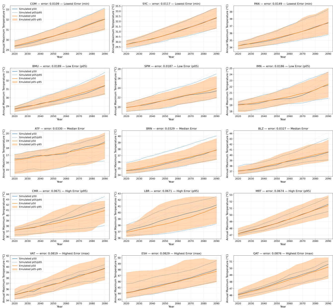
Figure D6. Time series of the 5th, 50th, and 95th percentile values of annual maximum temperature (°C) as emulated by RIME-X for the SSP3-7.0 scenario, compared to the corresponding empirical percentiles derived from ISIMIP simulations. The figure shows results for 15 selected regions: the three regions with the lowest, median, and highest normalized mean absolute error, as well as three regions each around the 5th and 95th percentile of the error distribution.
