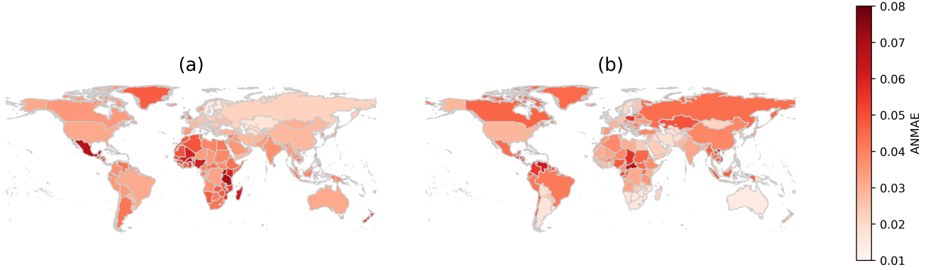
Figure 7. The average normalized mean absolute error ( ANMAE , see section 3.2.1) of emulated vs. simulated percentiles in each country. Panel (a) shows the annual average regional surface temperature compared to the 1995-2014 baseline for SSP2-4.5 in °C, and panel (b) shows the annual average regional precipitation compared to the 1995-2014 baseline for SSP2-4.5 in percent.
