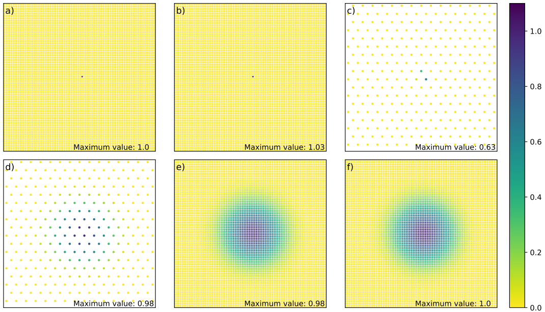
Figure 10. NICAS steps for an isotropic correlation function: \delta_i (a), N^T \delta_i (b), S^T N^T \delta_i (c), \widehat{C} S^T N^T \delta_i (d), \widehat{S} \widehat{C} S^T N^T \delta_i (e) and N \widehat{S} \widehat{C} S^T N^T \delta_i (f). The exact maximum value is indicated at the bottom right for each panel.
