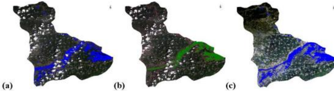
420 Figure 5: Comparison of monitoring results in the flood area of Weihui City based on the Z-score method. (a), 07/26/2021, (b), 07/27/2021, (c), 07/31/2021. The blue or green areas in the picture represent the areas affected by the flood.
