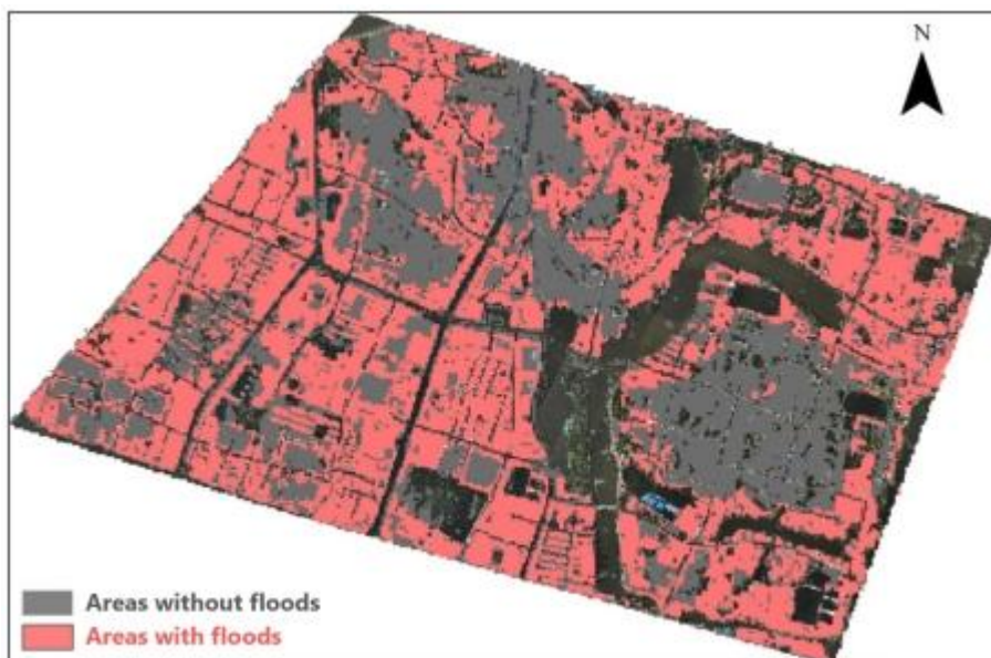
Figure 7: Flood monitoring results in the building area of Weihui City based on Sentinel-1 images and the Z-score method (Sentinel-1 data courtesy of ESA Copernicus). Grey indicates that the area has not been affected by the flood; red indicates that the area has been affected by the flood. The UAV imaging range is shown in Figure 1.
