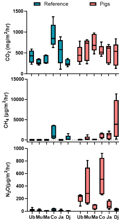
Figure 3. Greenhouse gas emissions (CO 2 , CH 4 and N 2 O) from reference plots (blue-left) and plots disturbed by feral pigs (red-right) for six sites across the floodplains during the Yekke season in Kakadu National Park: Ub = Ubirr, Mu = Munmarlay, Ma = Mamukala, Co = Coolaboo, Ja = Djaja, Dj = Djabulukgu. The box plots show the mean and standard error for five chambers at five plots within five sites; whiskers represent the minimum and maximum values.
