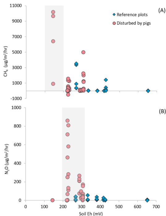
Figure 6. Relationship between soil Eh (mV) and (A) CH 4 and (B) N 2 O fluxes (μg m -2 hr -1 ) from reference (blue diamonds) and disturbed plots (red circles) by feral pigs. Low Eh (< 200 mV) values were associated with the highest CH 4 emissions, and values between 200 and 300 mV were associated with high N 2 O emissions, but only at plots disturbed by pigs. Shaded areas represent Eh conditions that favoured CH 4 (< 200 mV; A) and N 2 O (~200-300 mV; B) emissions.
