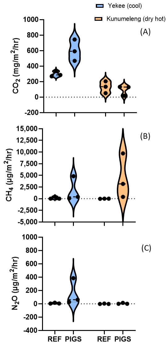
265 Figure 5. Greenhouse gas ( \text{CO}_2 , \text{CH}_4 and \text{N}_2\text{O} ) fluxes for two seasons: Yekke or cool season (blue-left) and Kunumeleng or pre-monsoon season (orange-right), for three plots without (REF-reference) and with feral pig disturbance (PIGS). Violins represent the distribution of the average of five chambers at three plots within three sites ( n = 3 ; Djabulukgu, Mamukala, and Munmurly-Coolaboo).
