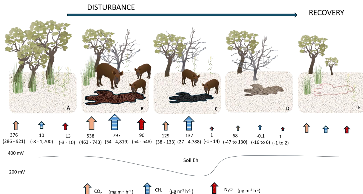
Figure 7. Schematic diagram on the greenhouse gas emission changes in a floodplain wetland (A) before pig disturbance; (B) during pig disturbance as vegetation is lost, surface soil Eh decreases, and soil decomposition and nitrogen inputs increase, resulting in very high CO 2 , CH 4 and N 2 O emissions; (C) as the site is less used as animals move closer to the remaining waterholes during drier months, N 2 O emissions decrease but CH 4 emissions remain high as oxygen is very low; (D) finally, once the site is abandoned, the soil is depleted of carbon and nitrogen, surface soil Eh potential increases, and fluxes are minimal; (E) potential pathway of recovery if feral pigs are managed.
