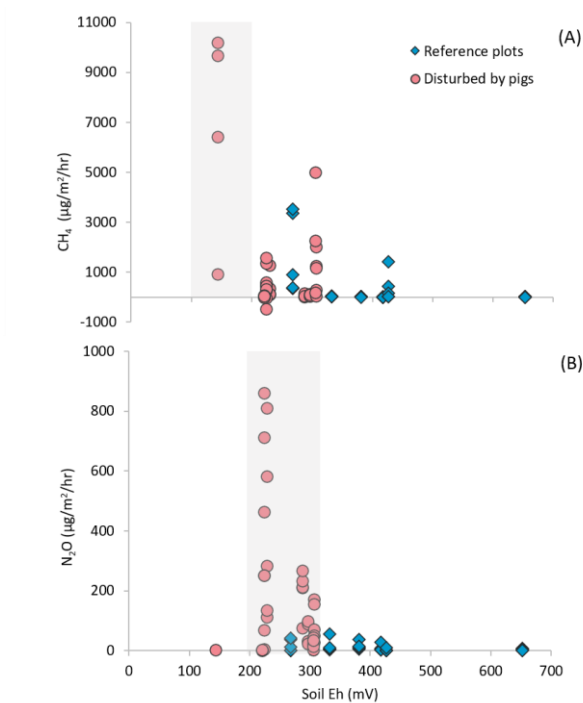
Figure 6. Relationship between soil Eh (mV) and (A) CH 4 and (B) N 2 O fluxes ( \mu\text{g m}^{-2} \text{ hr}^{-1} ) from reference (blue diamonds) and disturbed plots (red circles) by feral pigs. Low Eh ( < 200 mV) values were associated with the highest CH 4 emissions, and values between 200 and 300 mV were associated with high N 2 O emissions, but only at plots disturbed by pigs. Shaded areas represent Eh conditions that favoured CH 4 ( < 200 mV; A) and N 2 O ( \sim 200\text{-}300 mV; B) emissions.
