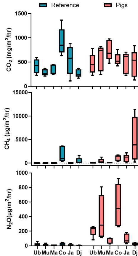
Figure 3. Greenhouse gas emissions ( \text{CO}_2 , \text{CH}_4 and \text{N}_2\text{O} ) from reference plots (blue-left) and plots disturbed by feral pigs (red-right) for six sites across the floodplains during the Yekke season in Kakadu National Park: Ub = Ubirr, Mu = Munmarlay, Ma = Mamukala, Co = Coolaboo, Ja = Djaja, Dj = Djabulukgu. The box plots show the mean and standard error for five chambers at five plots within five sites; whiskers represent the minimum and maximum values.
