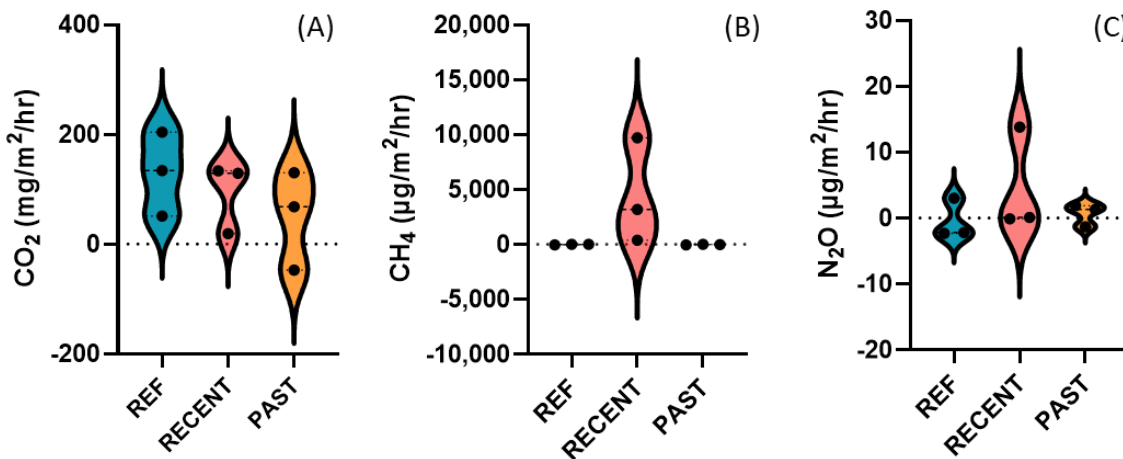
Figure 4. Greenhouse gas ( \text{CO}_2 , \text{CH}_4 , and \text{N}_2\text{O} ) fluxes of reference sites (REF- blue), sites previously used by pigs (PAST- orange), and recently used by pigs (RECENT-red). Violins represent the distribution of the average of five chambers of three plots within three sites (Djabulukgu, Mamukala, and Munmarlay) during Kunumeleng (pre-monsoon) season.
