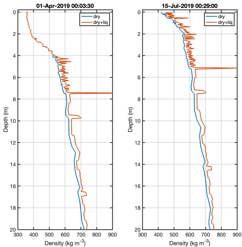
Figure A7. Modeled depth-density profiles for April and July of 2019 at Site MLD, showing the ablation of the snow layer, and the dry and wet densities.
