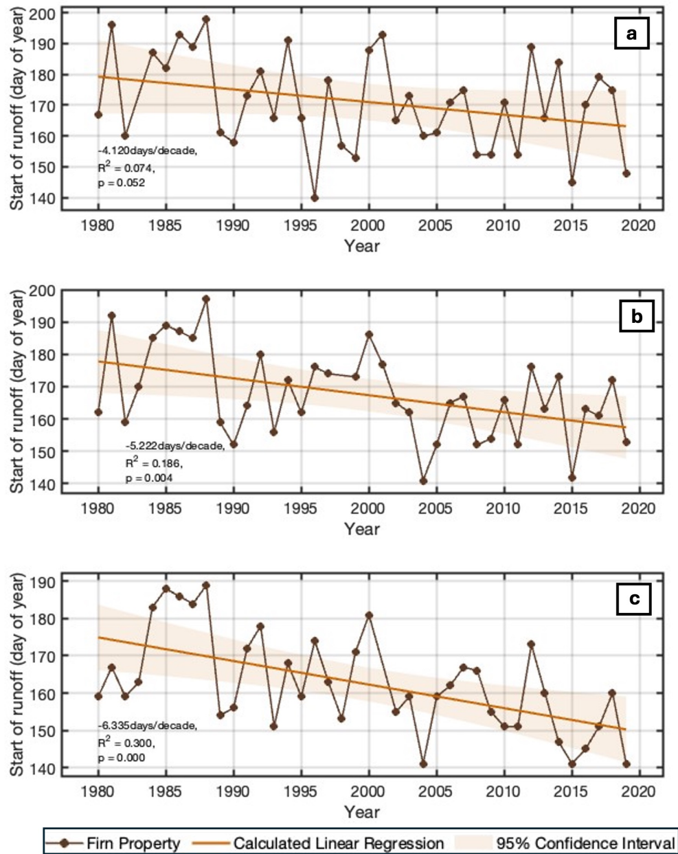
Figure A10. Modeled onset of runoff (day of year) for: a) MLD, b) MG3, and c) NWB1.
