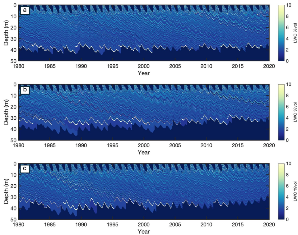
Figure A6. Modeled liquid-water content (LWC) evolution for the three sites: a) MLD, b) MG3, and c) NWB1.
