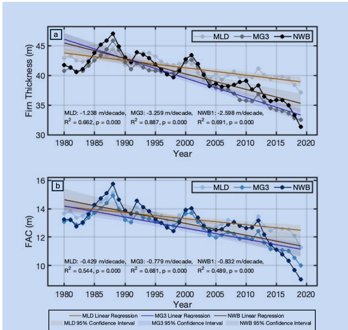
Figure 6. Modeled a) mean annual firn thickness and b) mean annual firn-air content (FAC) from the Kuipers Munneke (2015) firn-densification model at the accumulation-zone sites MLD, MG3, and NWB1 from 1980 to 2019.
