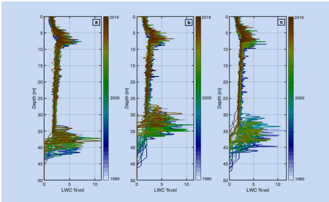
Figure A7. Modeled mean-annual liquid-water content (LWC) profiles for the three sites: a) MLD, b) MG3, and c) NWB1.
