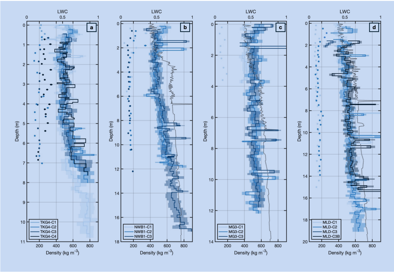
Figure 4. Measured density (blue lines), uncertainty estimates for observed density (shaded region), modeled depth-density profile for 1 June 2019 (dotted black line for accumulation zone sites), and measured liquid water content (blue circles). a) Site TKG4; b) Site NWB1; c) Site MG3; d) Site MLD.
