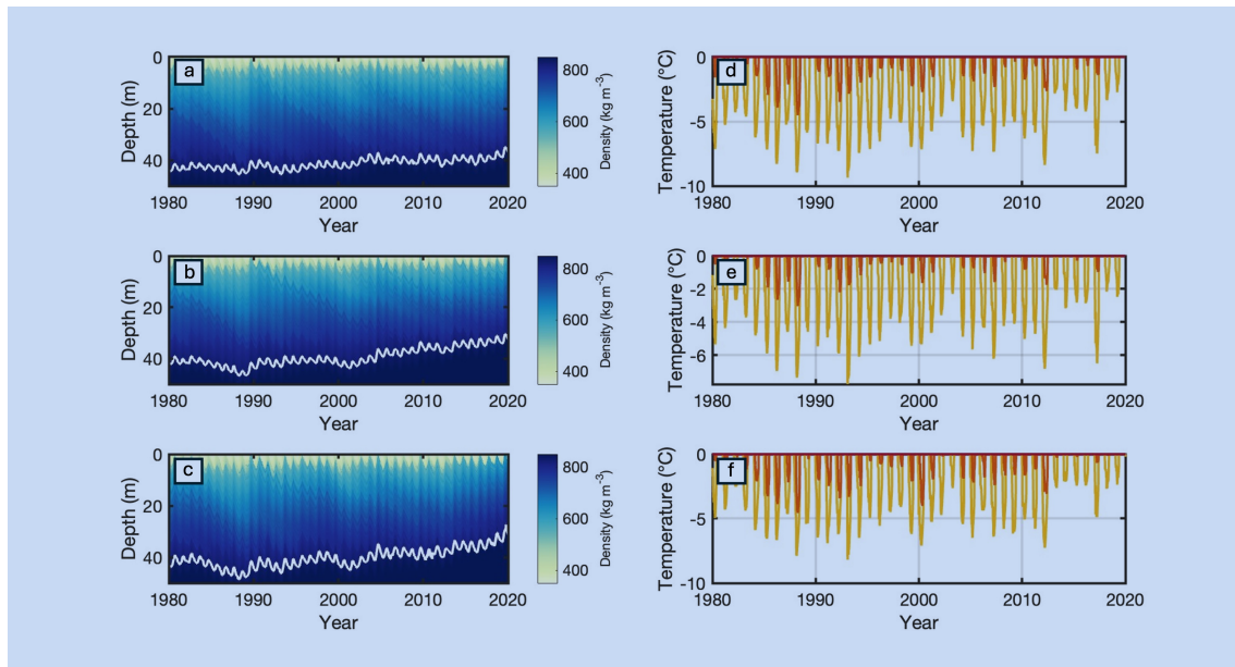
Figure 5. Modeled profiles of density (a-c) and modeled firn temperature (d-f) from 1980 to 2019 from Kuipers Munneke (2015) firn-densification model at the MLD site (a and d); MG3 site (b and e); and NWB1 site (c and f). Temperatures are shown at 3-m depth (light orange), 5-m depth (dark orange), and 8-m depth (red) in d-f. The temperature at 8-m depth was always at 0 °C over this interval, see Figure A5. Bubble close-off depth (approximately 830 \text{ kg m}^{-3} ) is delineated by the white line on a-c.
