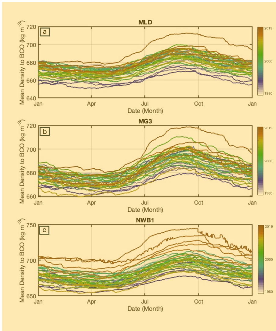
Figure A9. Modeled seasonal mean density (dry + liquid) from 1980-2019 for the three sites: a) MLD, b) MG3, and c) NWB1.
