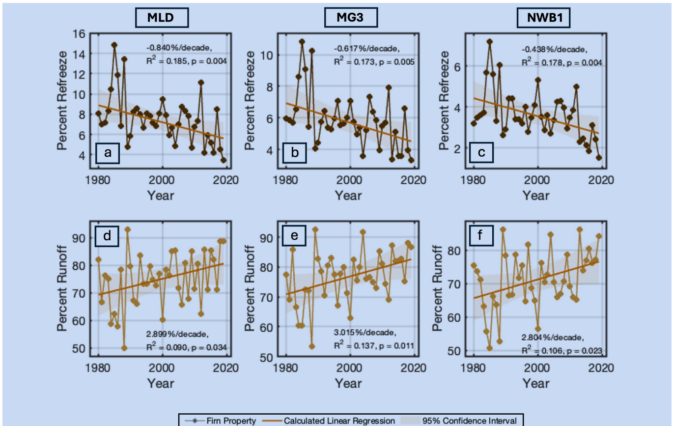
Figure 8. Percent of modeled mean annual melt and rain that refroze in the firn (a-c), and percent of modeled mean annual melt and rain that ran off from the firn (d-f) from 1980 to 2019.
