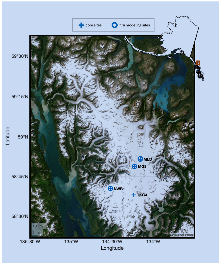
Figure 1. Overview map of the Juneau Icefield and the four primary study sites, situated along the Taku Glacier and two of its tributaries (Matthes Glacier and Northwest Branch). Core sites are marked by blue crosses (MLD, MG3, NWB1, and TKG4). Sites that are in the accumulation zone - for which the Community Firn Model was run - are marked by a blue cross and blue circle (MLD, MG3, and NWB1). The brown rectangle represents the icefield region within Alaska. The base map is derived from the Randolph Glacier Inventory (Consortium et al., 2023).
