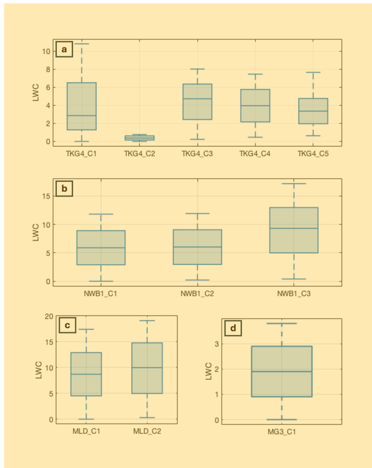
Figure 4. Box plots of repeated measurements of liquid water content (LWC) of the full cores at all the four sites.
