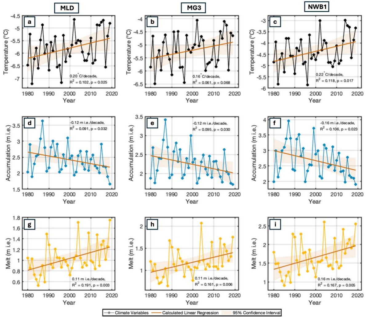
Figure 2. Mean annual climate at each site (MLD, MG3, NWB1) in the accumulation zone from the product by Ing et al. (2024): mean annual skin temperature (a-c), cumulative annual snow-accumulation (d-f), and cumulative surface melt (g-i).
