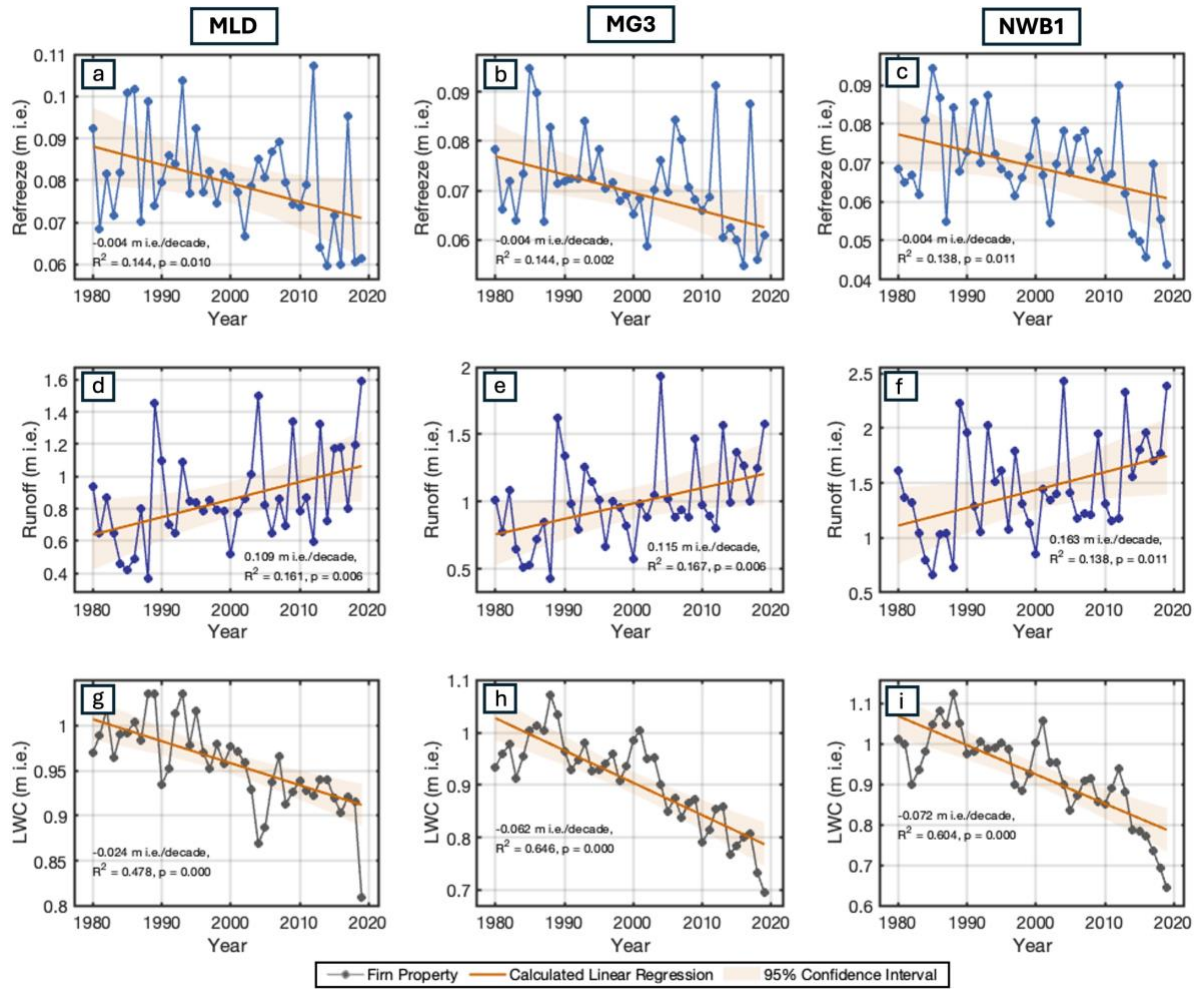
Figure 7. Modeled cumulative annual refreeze in the firn (a-c), modeled cumulative annual runoff (d-f), and modeled annual depth-averaged liquid-water content (LWC) in the firn (g-i).
