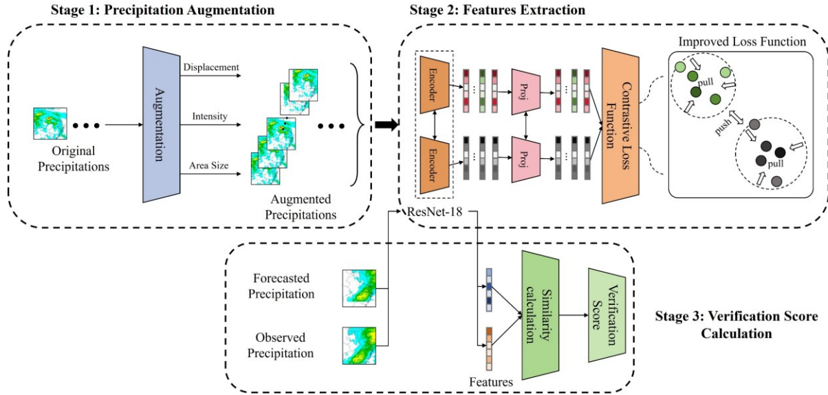
Figure 1: The overall framework of CLPFV.
