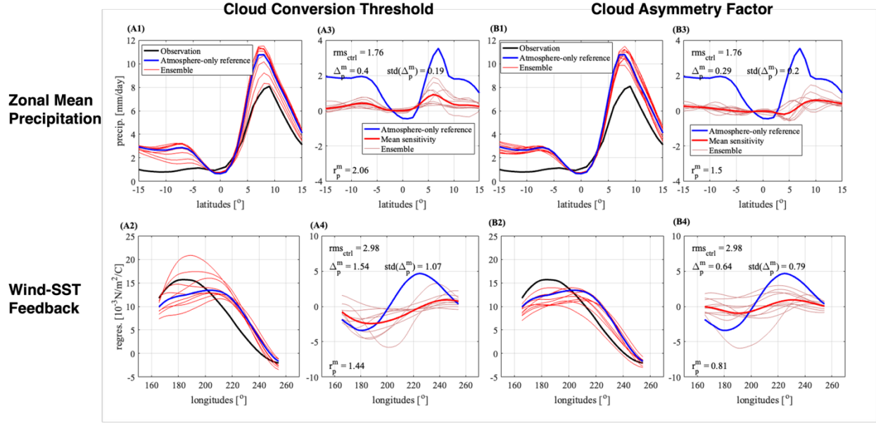
Figure 2: ENSO metric of Pacific zonal mean precipitation (upper row) and zonal wind-SST regression (lower row) for observations (black), reference atmosphere-only run (blue) and perturbed cloud conversion threshold (tune_rprcon) parameters for atmosphere-only runs (red). Column 2 (A3, A4): correspond sensitivity estimate for each perturbation runs (thin red lines); the ensemble means of them (thick red line) and the reference bias (blue line). B1, B2, B3 and B4 are for cloud asymmetry factor parameter (tune_box_liq_asy).
