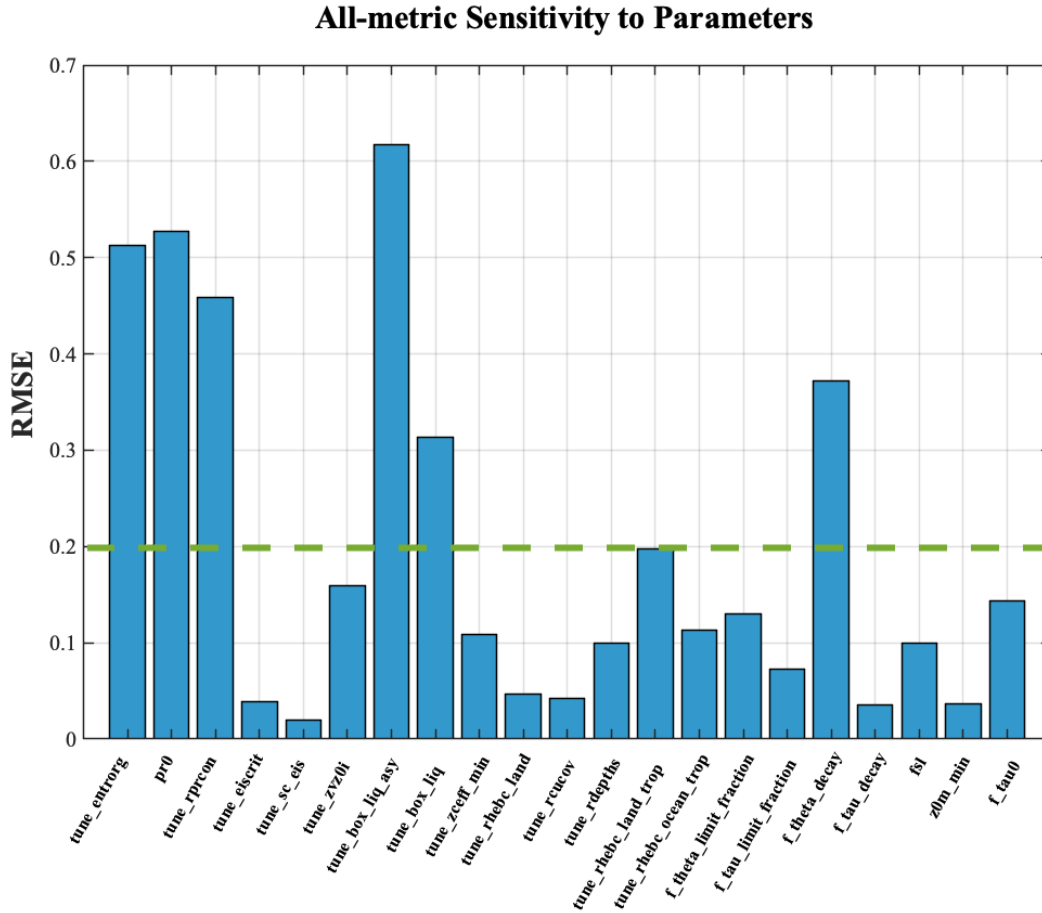
Figure 5: mean RMS values of the sensitivity of the combined ENSO metrics in atmosphere-only runs for all 21 parameters. A mean RMS sensitivity of 1.0 refers to a sensitivity as strong in amplitude as the atmosphere-only control run biases. Parameters exhibiting RMSE values above the threshold of 0.2 (horizontal green dashed line) are considered to have significant impacts on ENSO simulation during the atmosphere-only model tuning phase.
