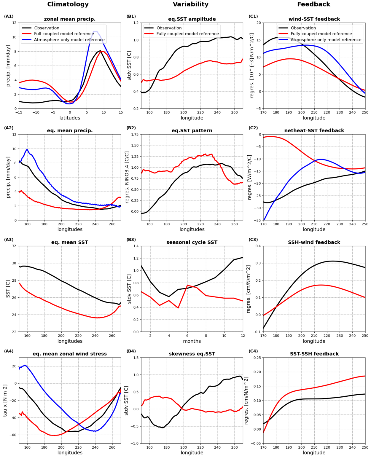
Figure 1. Comparison of some ENSO Metrics for Observations (black), ICON atmosphere-only model (blue), and ICON fully coupled (red) reference simulations for climatology (left), variability (middle) and feedback (right). The metrics definition can be found in Planton et al. (2021).
