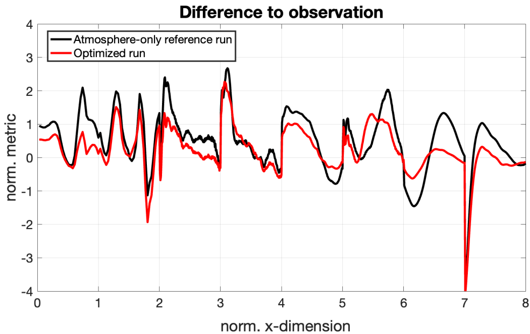
Figure 6: Normalized and combined ENSO metrics in atmosphere-only simulations for a simulation with the atmosphere-only reference parameters (black) and for a run with 21 optimized parameters (red). A zero value suggest a match to the observed reference. The norm. X-dimension has same definition with in Fig. 3.
