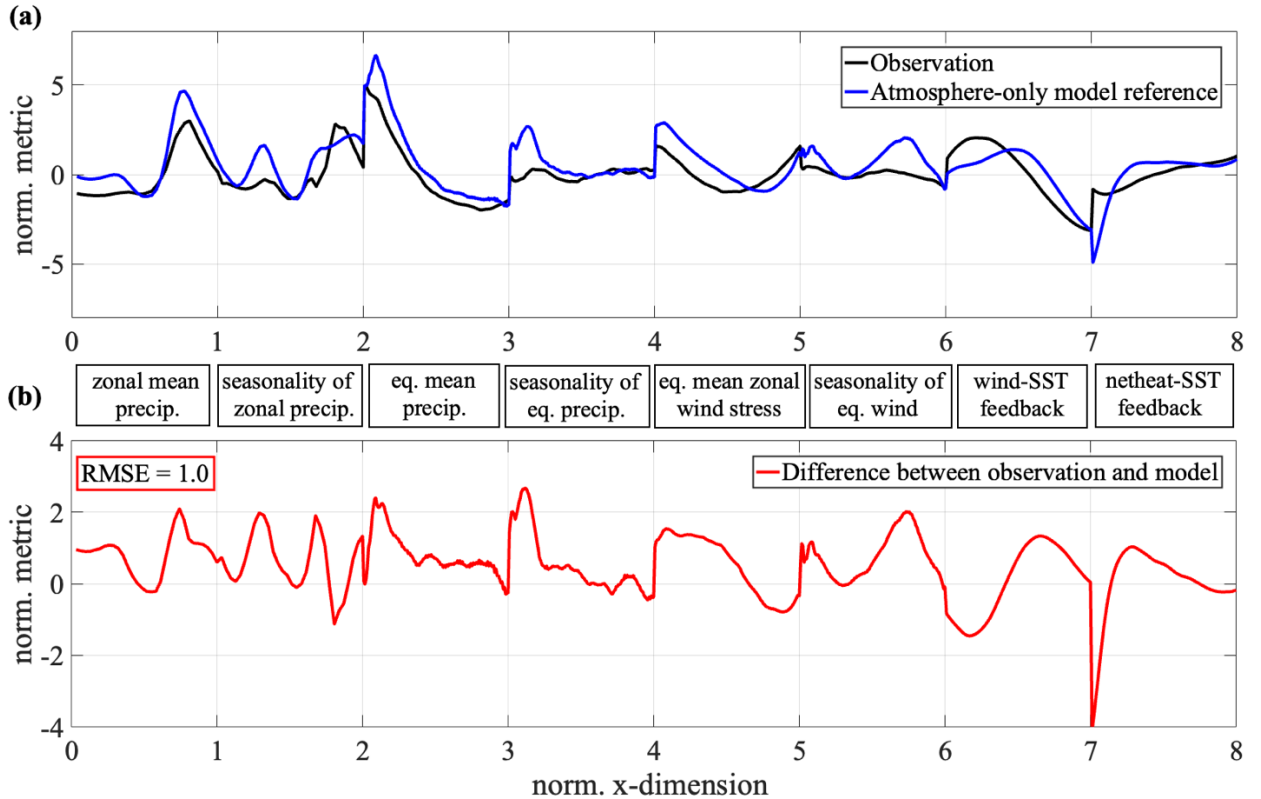
Figure 3. Normalized and combined ENSO metric for the atmosphere-only simulations. (a) shows the observed (black) and atmosphere-only simulation (blue) values of the combined ENSO metric. The x-axis is a combined dimension of the 8 ENSO metrics used for atmosphere-only simulations with the labels marking which part of the x-axis corresponds to which ENSO metric. (b) shows the difference between the atmosphere-only model run and the
