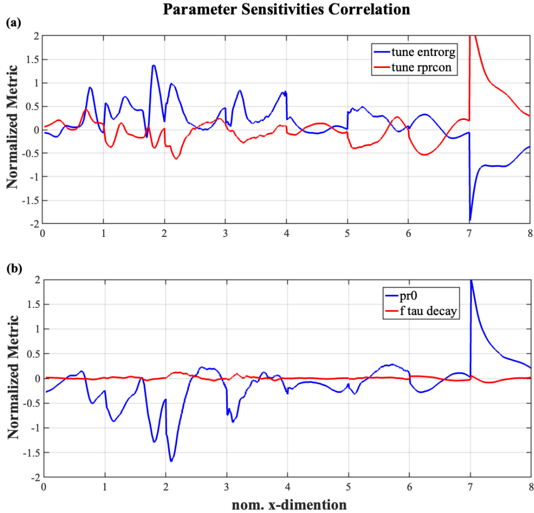
Figure 4: Normalized sensitivity of the combined ENSO metrics in atmosphere-only runs for four different tuning parameters, (a): tune_entrorg and tune_rprcon; (b): pr0 and f_tau_decay. The correlation between the pair of sensitivities is shown in the heading of each panel. The norm. X-dimension has same definition with in Fig. 3.
