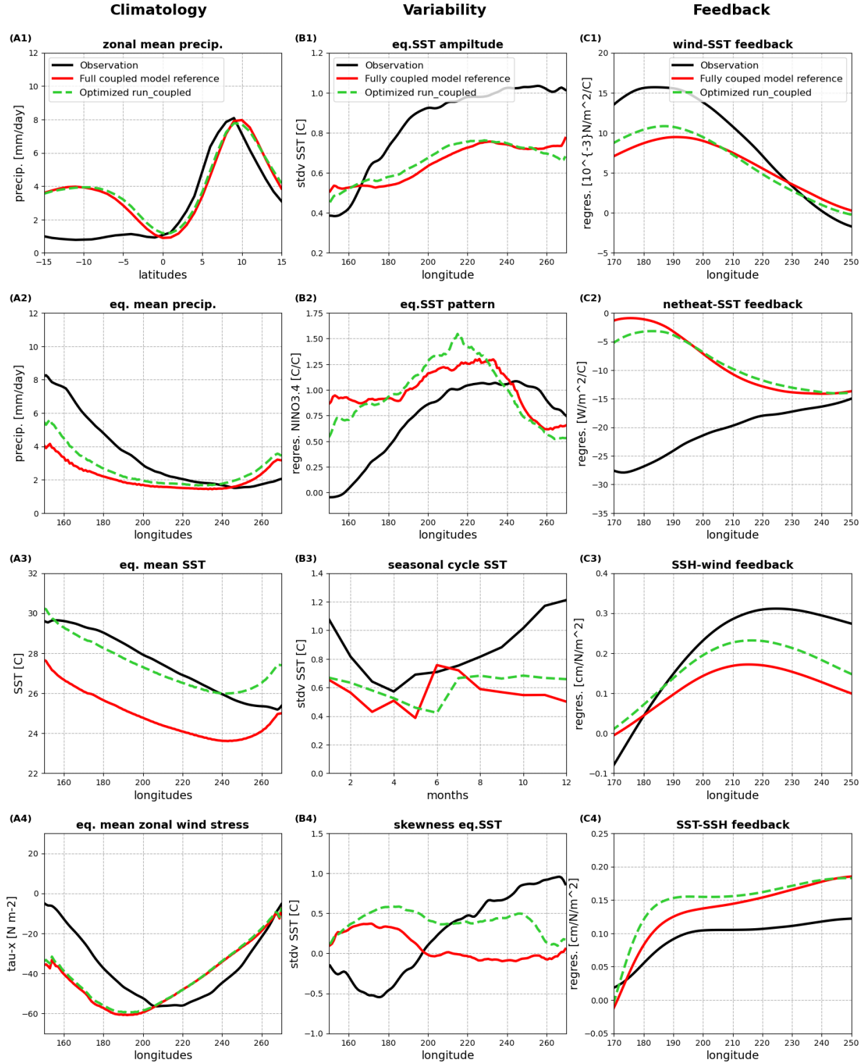
Figure 9. Comparison of ENSO metrics from the ICON XPP fully coupled reference simulation (“Fully coupled model reference”, red line), observations (“Observation”, black line), and the
