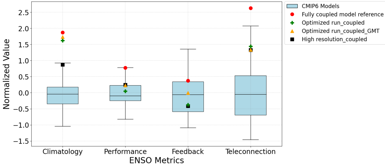
Figure 10. Summary of ICON XPP model performance across different categories of ENSO metrics—tropical climatology, ENSO characteristics, feedbacks, and teleconnections—comparing the fully coupled reference run (“Fully coupled model reference”, red point), optimized coupled-model experiment (“Optimized run_coupled”, green cross), fully coupled high resolution run for ICON XPP model (“high resolution_coupled”, black rectangle), optimized coupled-model experiment with global mean temperature (GMT) correction (“Optimized run_coupled_GMT”, yellow triangle). The CMIP6 distribution is shown as a boxplot with the box representing the interquartile range (25th–75th percentile), the central line indicating the median, and whiskers showing the full model spread (minimum to maximum). See Planton et al. (2021) for detailed definitions of all ENSO metrics and different categories. The ENSO metrics values for observation are -2.43, -1.77, -2.27, and -6.82 for Climatology, Performance, Feedback, and Teleconnection, respectively.
