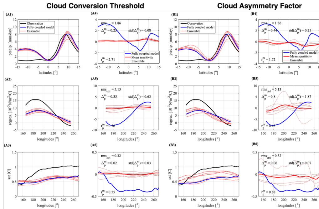
Figure 8. Sensitivity of ENSO-relevant metrics to perturbations in the cloud conversion threshold ( tune_rprcon ) (A1-A6) and cloud asymmetry factor parameter ( tune_box_liq_asy ) (B1-B6) from fully coupled simulations. Panels (A1-A3 and B1-B3) show metric values from observations (black), ICON XPP fully coupled reference run (blue), and perturbed parameters ensemble (ensemble) simulations (red) same with atmosphere-only sensitivity results in Figure 3. Corresponding sensitivity estimates are shown in panels (A4-A6, and B4-B6), including ensemble mean sensitivity (thick red), spread (thin red), and reference bias (blue). The third row (A3, A6, B3 and B6) are for ENSO amplitude, standard deviation of Sea Surface Temperature Anomalies (SSTA) in the central equatorial Pacific, which is not included in the atmosphere-only results.
