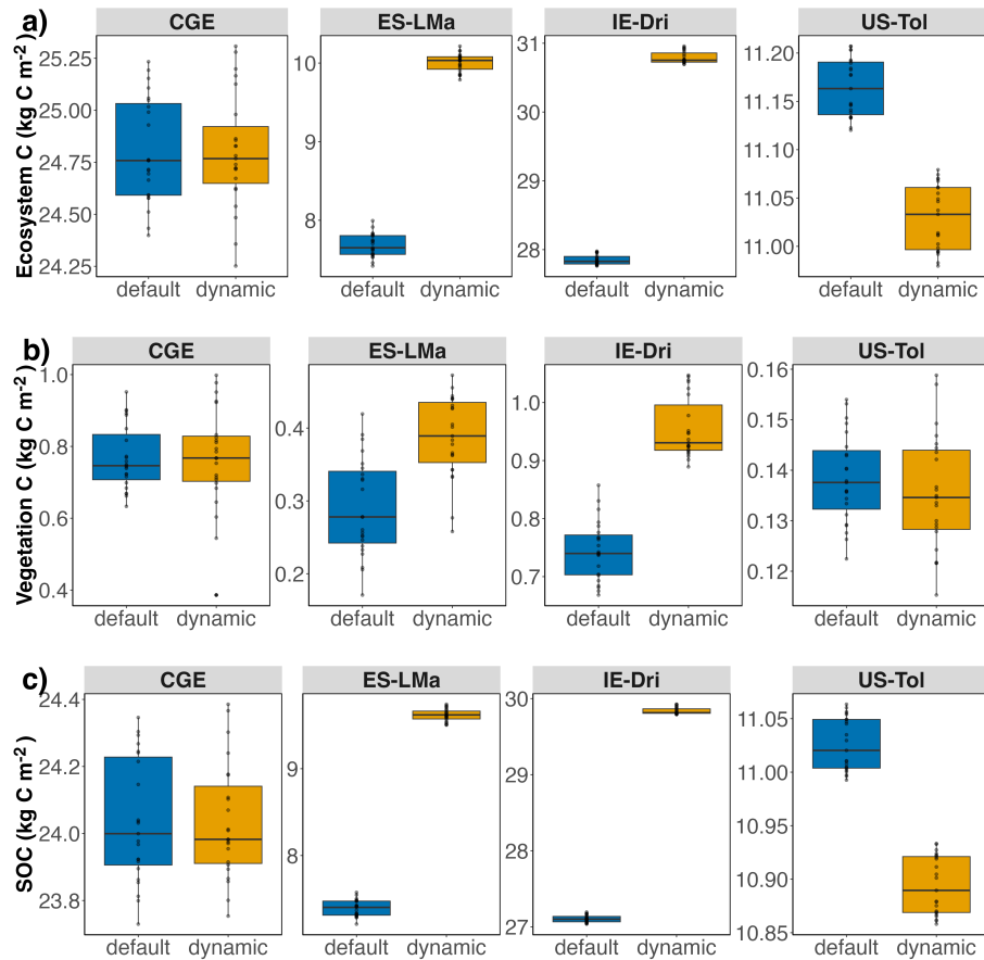
Figure 4. Mean annual ecosystem C (a) vegetation ecosystem C , (b) vegetation C and (c) soil organic carbon (SOC; e ) of the default model and dynamic model at the four main sites IE-Dri, CGE, ES-LMa and US-Tol for the years 2000-2022. Statistical results are shown in Table C3.
