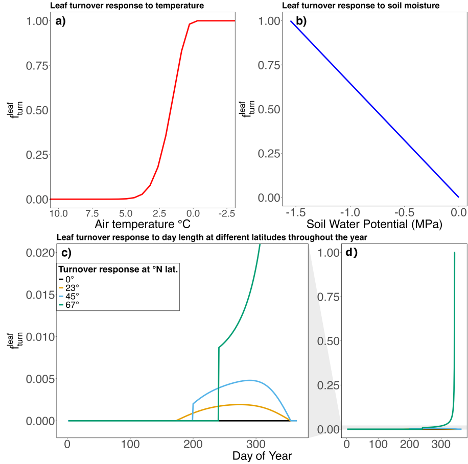
Figure 1. The three-components individual impacts of the dynamic-turnover-model , three environmental stressors: a) air temperature (a see Eq. 6), b) soil moisture (b see Eq. 7), and c) and d) day length response (c see Eq. 13-15) and their impact on leaf turnover ( f_{turn}^{leaf} ) in the dynamic model (see Section 2.3). The combined f_{turn}^{leaf} from these three components is shown in Eq. 16. The leaf turnover response to day length response (c and d) is shown for different example latitudes and on the left part of northern hemisphere, but the figure-model provides continuous global coverage for all latitudes. Panel d) shows the full range of light induced leaf turnover and panel c) is an enlarged view of the right day-length plot this to show the exact pattern as well as timing of leaf turnover response to changing day length.
